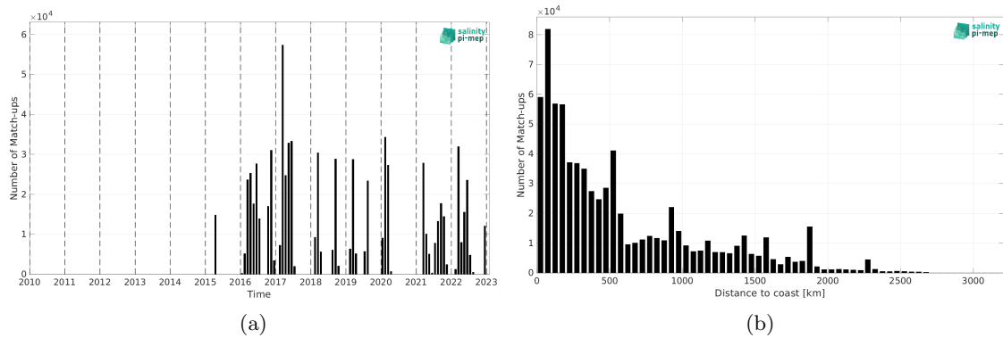
Figure 2: Number of match-ups between TSG (GOSUD-Research-vessel) and SMAP SSS L3 v6 - 8-Day running (RSS) SSS as a function of time (a) and as function of the distance to coast (b) over the Tropical Atlantic Ocean Pi-MEP region and for the full satellite product period.
