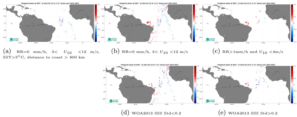
Figure 14: Temporal mean gridded over spatial boxes of size 1^\circ \times 1^\circ of \Delta\text{SSS} (SMAP SSS L3 v6 - 8-Day running (RSS) - TSG (CSIC-UTM)) for 5 different subdatasets corresponding to:RR=0 mm/h, 3 < U_{10} < 12 m/s, SST >5^\circ\text{C} , distance to coast > 800 km (a), RR=0 mm/h, 3 < U_{10} < 12 m/s (b), RR >1 mm/h and U_{10} < 4 m/s (c), WOA2013 SSS Std <0.2 (d), WOA2013 SSS Std >0.2 (e).
