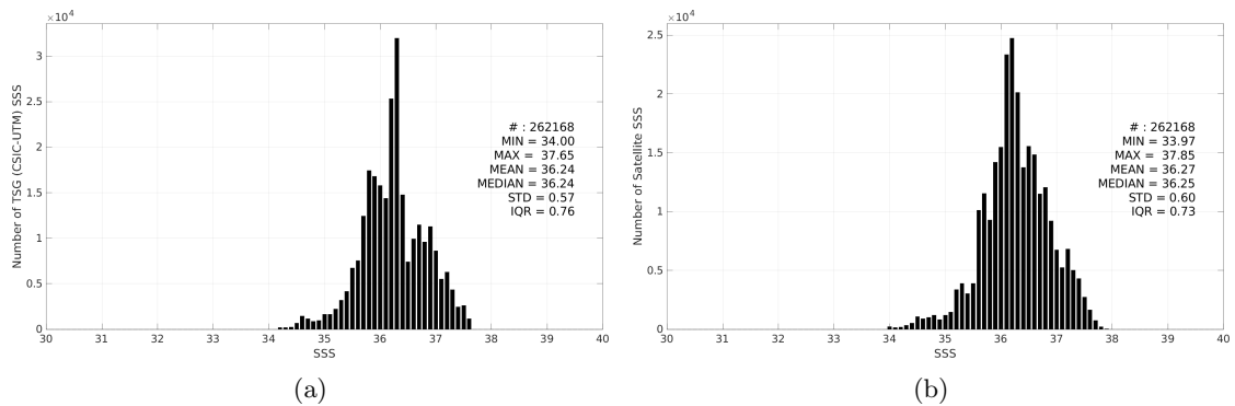
Figure 3: Histograms of SSS from TSG (CSIC-UTM) (a) and SMAP SSS L3 v6 - 8-Day running (RSS) (b) considering all match-up pairs per bins of 0.1 over the Tropical Atlantic Ocean Pi-MEP region and for the full satellite product period.
