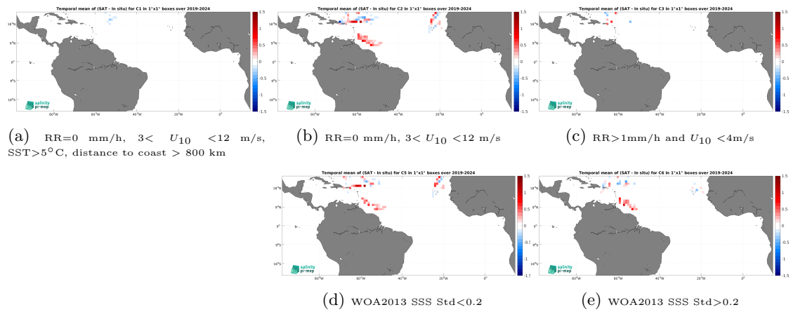
Figure 14: Temporal mean gridded over spatial boxes of size 1^\circ \times 1^\circ of \Delta\text{SSS} (SMAP SSS L3 v6 - 8-Day running (RSS) - Saildrone) for 5 different subdatasets corresponding to: RR=0 mm/h, 3 < U_{10} < 12 m/s, SST > 5°C, distance to coast > 800 km (a), RR=0 mm/h, 3 < U_{10} < 12 m/s (b), RR > 1 mm/h and U_{10} < 4 m/s (c), WOA2013 SSS Std < 0.2 (d), WOA2013 SSS Std > 0.2 (e).
