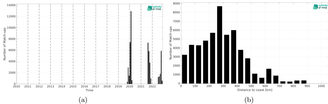
Figure 2: Number of match-ups between Saildrone and SMAP SSS L3 v6 - 8-Day running (RSS) SSS as a function of time (a) and as function of the distance to coast (b) over the Tropical Atlantic Ocean Pi-MEP region and for the full satellite product period.
