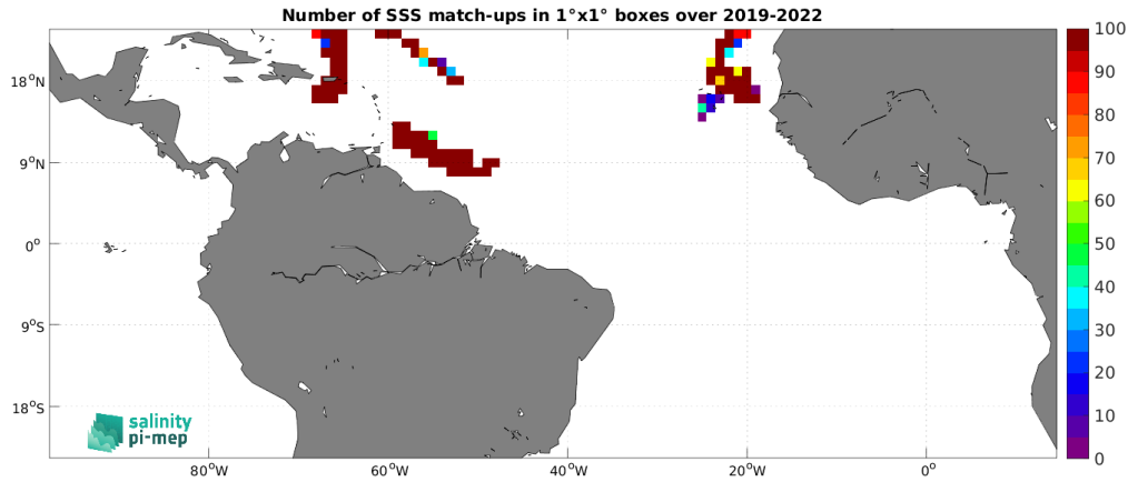
Figure 5: Number of SSS match-ups between Saildrone SSS and the SMAP SSS L3 v6 - 8-Day running (RSS) SSS product for the Tropical Atlantic Ocean Pi-MEP region over 1^\circ \times 1^\circ boxes and for the full satellite product period.
