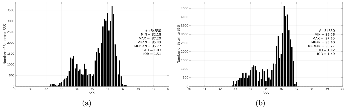
Figure 3: Histograms of SSS from Saildrone (a) and SMAP SSS L3 v6 - 8-Day running (RSS) (b) considering all match-up pairs per bins of 0.1 over the Tropical Atlantic Ocean Pi-MEP region and for the full satellite product period.
