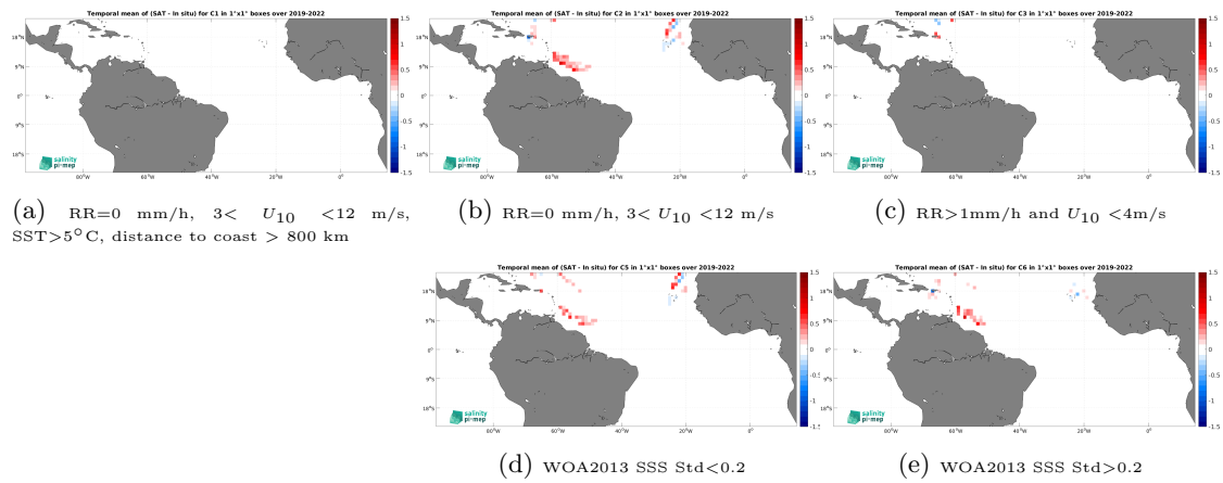
Figure 14: Temporal mean gridded over spatial boxes of size 1^\circ \times 1^\circ of \Delta\text{SSS} (SMAP SSS L3 v6 - 8-Day running (RSS) - Sairdrone) for 5 different subdatasets corresponding to:RR=0 mm/h, 3 < U_{10} < 12 m/s, SST>5°C, distance to coast > 800 km (a), RR=0 mm/h, 3 < U_{10} < 12 m/s (b), RR>1mm/h and U_{10} < 4 m/s (c), WOA2013 SSS Std<0.2 (d), WOA2013 SSS Std>0.2 (e).
