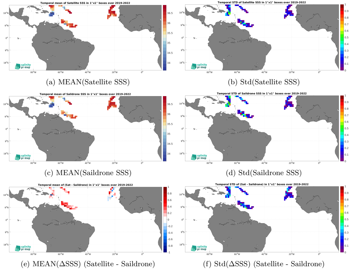
Figure 7: Temporal mean (left) and Std (right) of SSS from SMAP SSS L3 v6 - 8-Day running (RSS) (top), Saildrone (middle), and of \Delta\text{SSS} (Satellite - Saildrone). Only match-up pairs are used to generate these maps.
