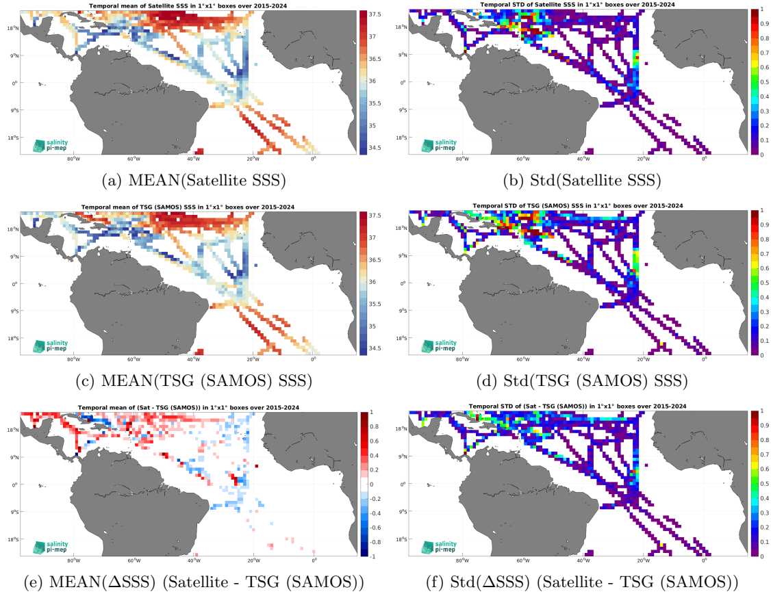
Figure 7: Temporal mean (left) and Std (right) of SSS from SMAP SSS L3 v6 - Monthly (RSS) (top), TSG (SAMOS) (middle), and of \Delta\text{SSS} (Satellite - TSG (SAMOS)). Only match-up pairs are used to generate these maps.
