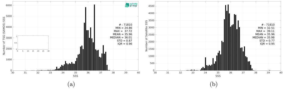
Figure 3: Histograms of SSS from TSG (SAMOS) (a) and SMAP SSS L3 v6 - Monthly (RSS) (b) considering all match-up pairs per bins of 0.1 over the Tropical Atlantic Ocean Pi-MEP region and for the full satellite product period.
