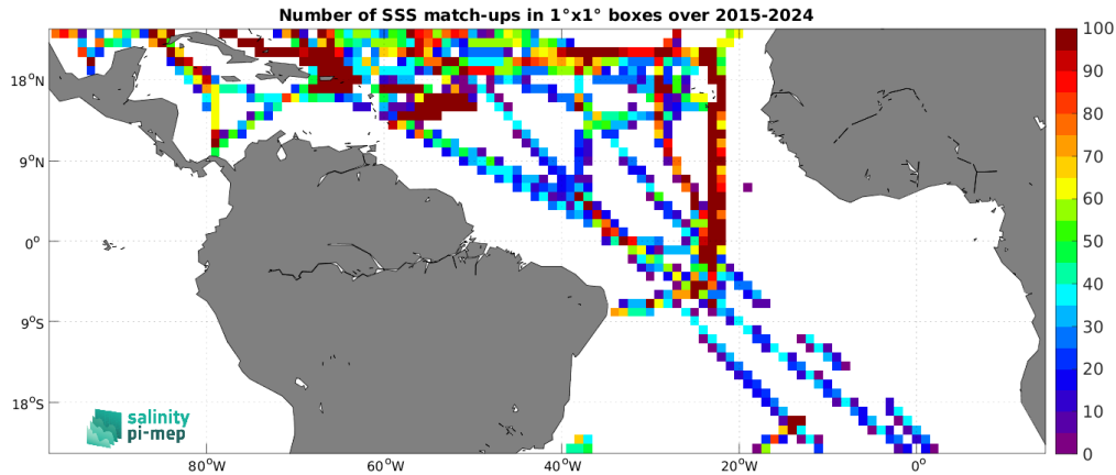
Figure 5: Number of SSS match-ups between TSG (SAMOS) SSS and the SMAP SSS L3 v6 - Monthly (RSS) SSS product for the Tropical Atlantic Ocean Pi-MEP region over 1^\circ \times 1^\circ boxes and for the full satellite product period.
