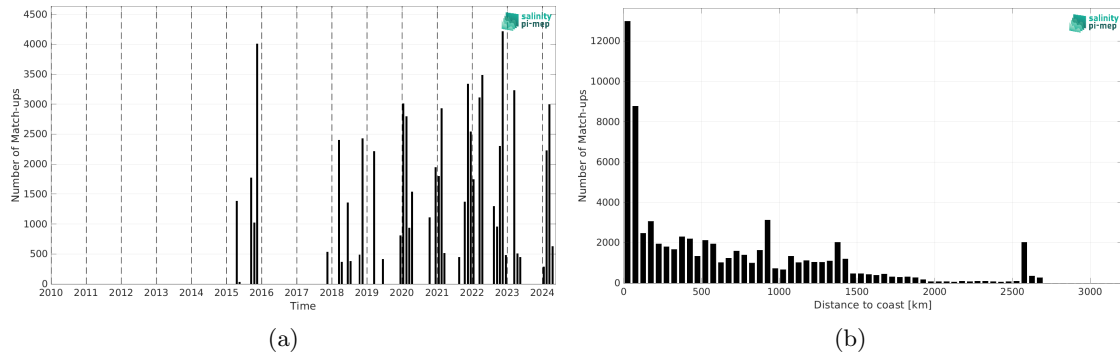
Figure 2: Number of match-ups between TSG (SAMOS) and SMAP SSS L3 v6 - Monthly (RSS) SSS as a function of time (a) and as function of the distance to coast (b) over the Tropical Atlantic Ocean Pi-MEP region and for the full satellite product period.
