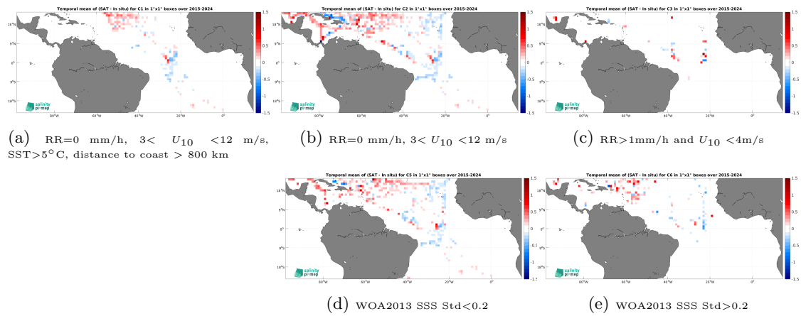
Figure 14: Temporal mean gridded over spatial boxes of size 1^\circ \times 1^\circ of \Delta\text{SSS} (SMAP SSS L3 v6 - Monthly (RSS) - TSG (SAMOS)) for 5 different subdatasets corresponding to:RR=0 mm/h, 3 < U_{10} < 12 m/s, SST >5^\circ\text{C} , distance to coast > 800 km (a), RR=0 mm/h, 3 < U_{10} < 12 m/s (b), RR >1 mm/h and U_{10} < 4 m/s (c), WOA2013 SSS Std <0.2 (d), WOA2013 SSS Std >0.2 (e).
