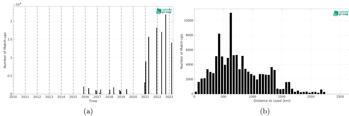
Figure 2: Number of match-ups between TSG (Polarstern) and SMAP SSS L3 v6 - Monthly (RSS) SSS as a function of time (a) and as function of the distance to coast (b) over the Tropical Atlantic Ocean Pi-MEP region and for the full satellite product period.
