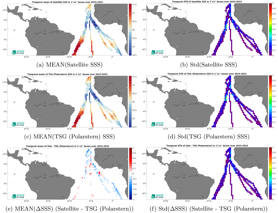
Figure 7: Temporal mean (left) and Std (right) of SSS from SMAP SSS L3 v6 - Monthly (RSS) (top), TSG (Polarstern) (middle), and of \Delta\text{SSS} (Satellite - TSG (Polarstern)). Only match-up pairs are used to generate these maps.
