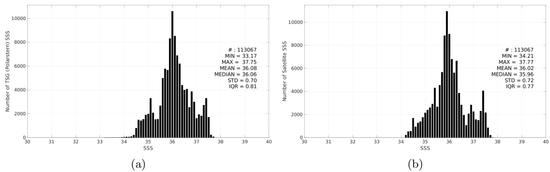
Figure 3: Histograms of SSS from TSG (Polarstern) (a) and SMAP SSS L3 v6 - Monthly (RSS) (b) considering all match-up pairs per bins of 0.1 over the Tropical Atlantic Ocean Pi-MEP region and for the full satellite product period.
