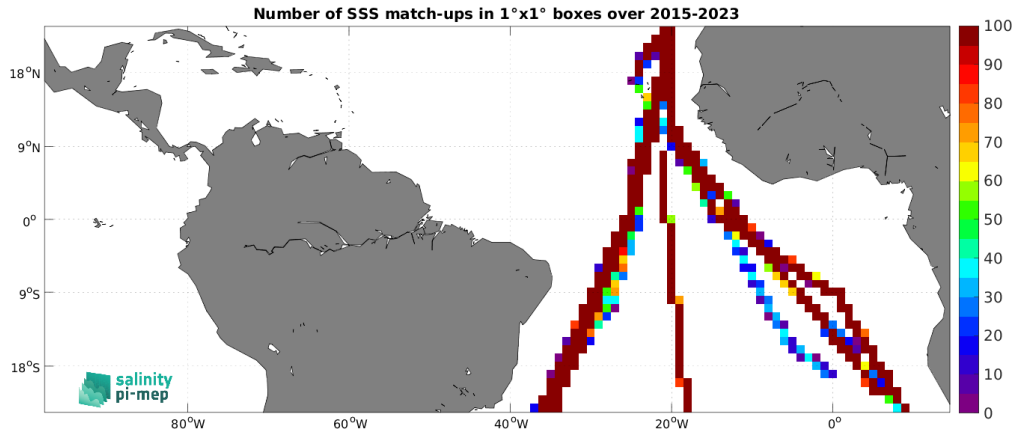
Figure 5: Number of SSS match-ups between TSG (Polarstern) SSS and the SMAP SSS L3 v6 - Monthly (RSS) SSS product for the Tropical Atlantic Ocean Pi-MEP region over 1^\circ \times 1^\circ boxes and for the full satellite product period.
