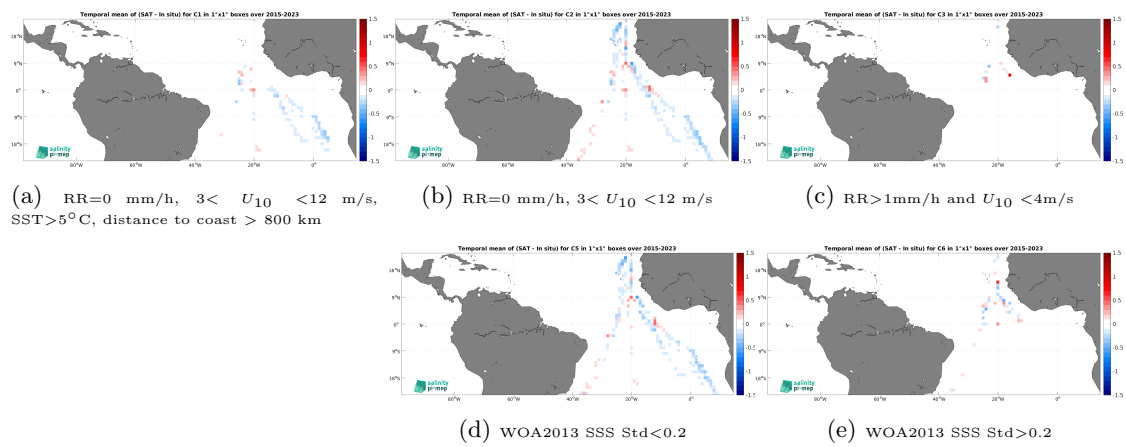
Figure 14: Temporal mean gridded over spatial boxes of size 1^\circ \times 1^\circ of \Delta\text{SSS} (SMAP SSS L3 v6 - Monthly (RSS) - TSG (Polarstern)) for 5 different subdatasets corresponding to:RR=0 mm/h, 3 < U_{10} < 12 m/s, SST >5^\circ\text{C} , distance to coast > 800 km (a), RR=0 mm/h, 3 < U_{10} < 12 m/s (b), RR >1 mm/h and U_{10} < 4 m/s (c), WOA2013 SSS Std <0.2 (d), WOA2013 SSS Std >0.2 (e).
