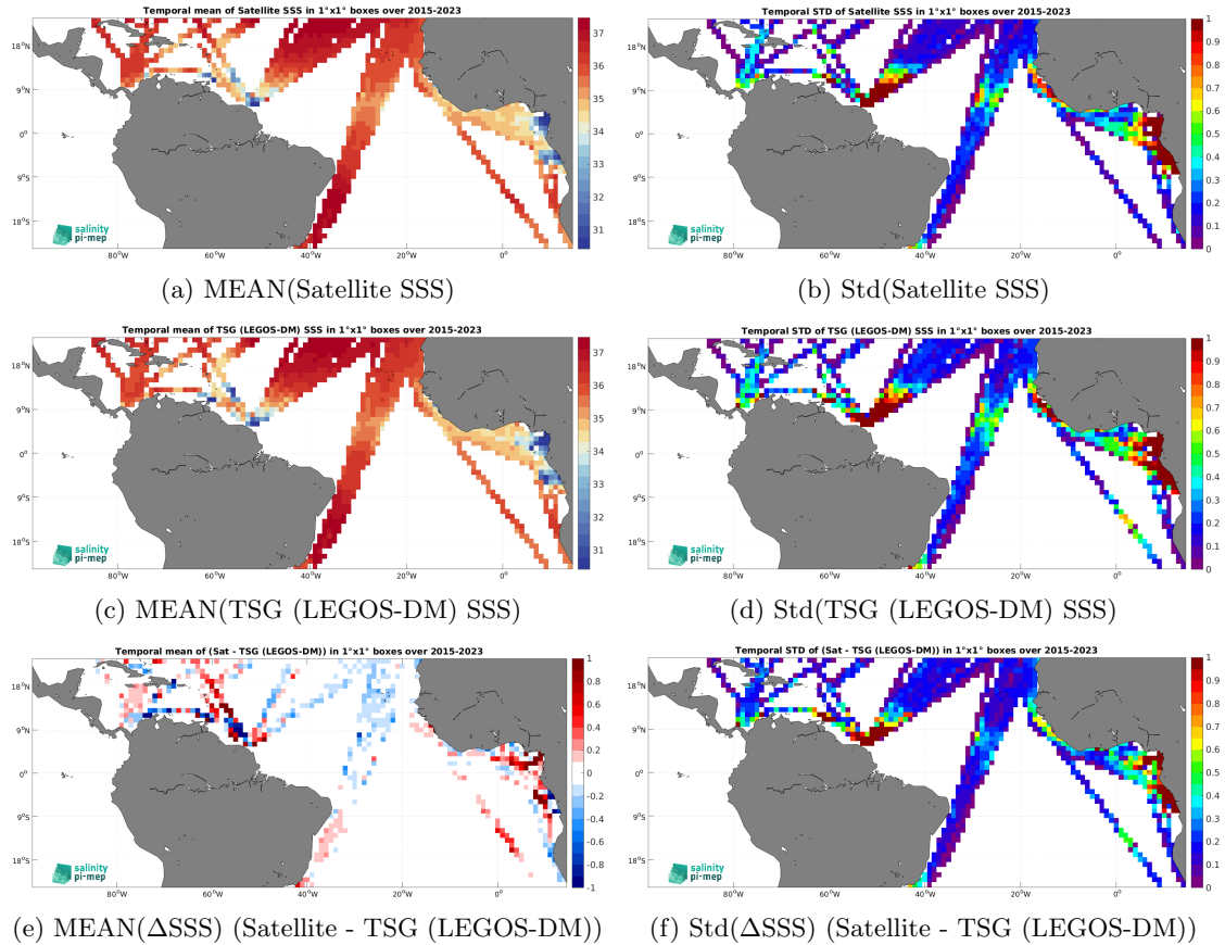
Figure 7: Temporal mean (left) and Std (right) of SSS from SMAP SSS L3 v6 - Monthly (RSS) (top), TSG (LEGOS-DM) (middle), and of \Delta\text{SSS}(\text{Satellite} - \text{TSG}(\text{LEGOS-DM})) . Only match-up pairs are used to generate these maps.
