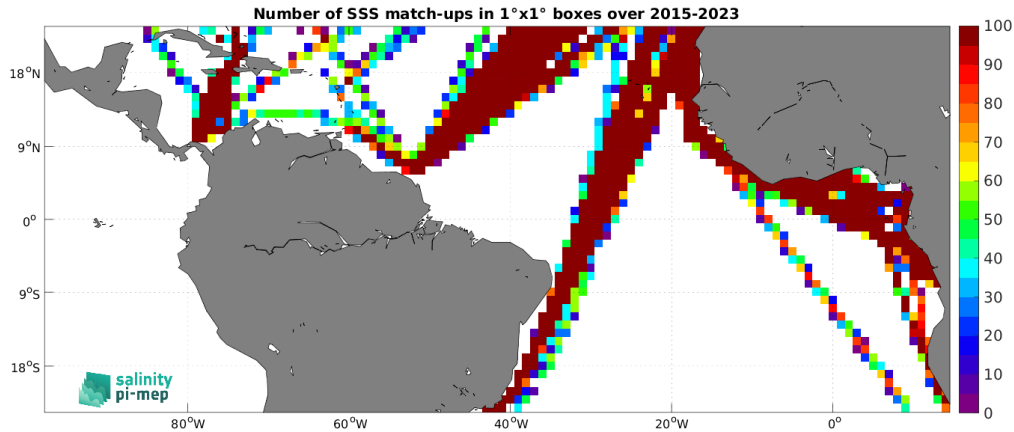
Figure 5: Number of SSS match-ups between TSG (LEGOS-DM) SSS and the SMAP SSS L3 v6 - Monthly (RSS) SSS product for the Tropical Atlantic Ocean Pi-MEP region over 1^\circ \times 1^\circ boxes and for the full satellite product period.
