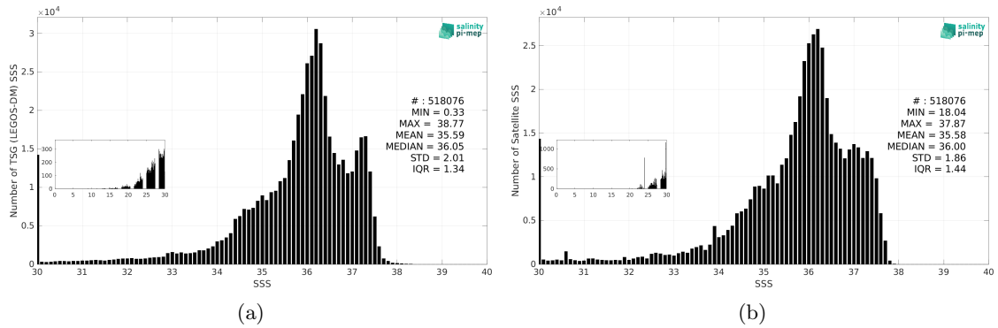
Figure 3: Histograms of SSS from TSG (LEGOS-DM) (a) and SMAP SSS L3 v6 - Monthly (RSS) (b) considering all match-up pairs per bins of 0.1 over the Tropical Atlantic Ocean Pi-MEP region and for the full satellite product period.
