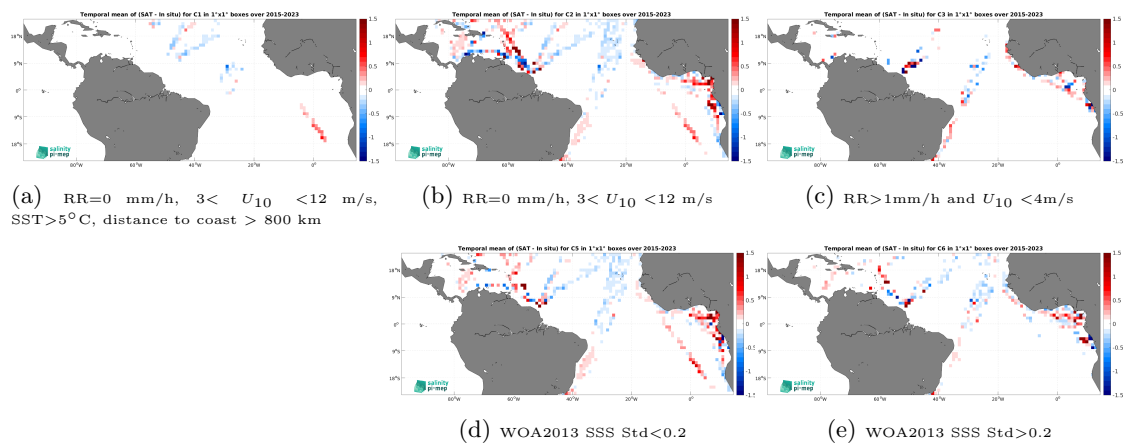
Figure 14: Temporal mean gridded over spatial boxes of size 1^\circ \times 1^\circ of \Delta\text{SSS} (SMAP SSS L3 v6 - Monthly (RSS) - TSG (LEGOS-DM)) for 5 different subdatasets corresponding to:RR=0 mm/h, 3 < U_{10} < 12 m/s, SST >5^\circ\text{C} , distance to coast > 800 km (a), RR=0 mm/h, 3 < U_{10} < 12 m/s (b), RR >1 mm/h and U_{10} < 4 m/s (c), WOA2013 SSS Std <0.2 (d), WOA2013 SSS Std >0.2 (e).
