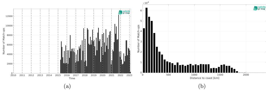
Figure 2: Number of match-ups between TSG (LEGOS-DM) and SMAP SSS L3 v6 - Monthly (RSS) SSS as a function of time (a) and as function of the distance to coast (b) over the Tropical Atlantic Ocean Pi-MEP region and for the full satellite product period.
