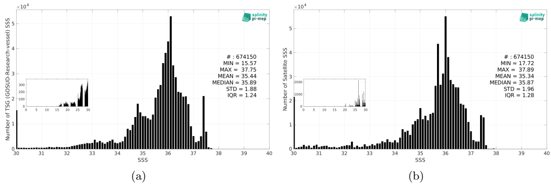
Figure 3: Histograms of SSS from TSG (GOSUD-Research-vessel) (a) and SMAP SSS L3 v6 - Monthly (RSS) (b) considering all match-up pairs per bins of 0.1 over the Tropical Atlantic Ocean Pi-MEP region and for the full satellite product period.
