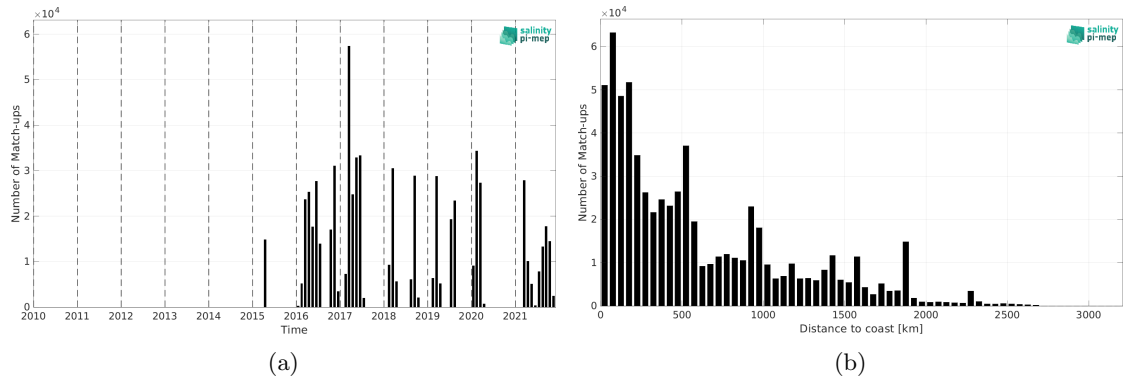
Figure 2: Number of match-ups between TSG (GOSUD-Research-vessel) and SMAP SSS L3 v6 - Monthly (RSS) SSS as a function of time (a) and as function of the distance to coast (b) over the Tropical Atlantic Ocean Pi-MEP region and for the full satellite product period.
