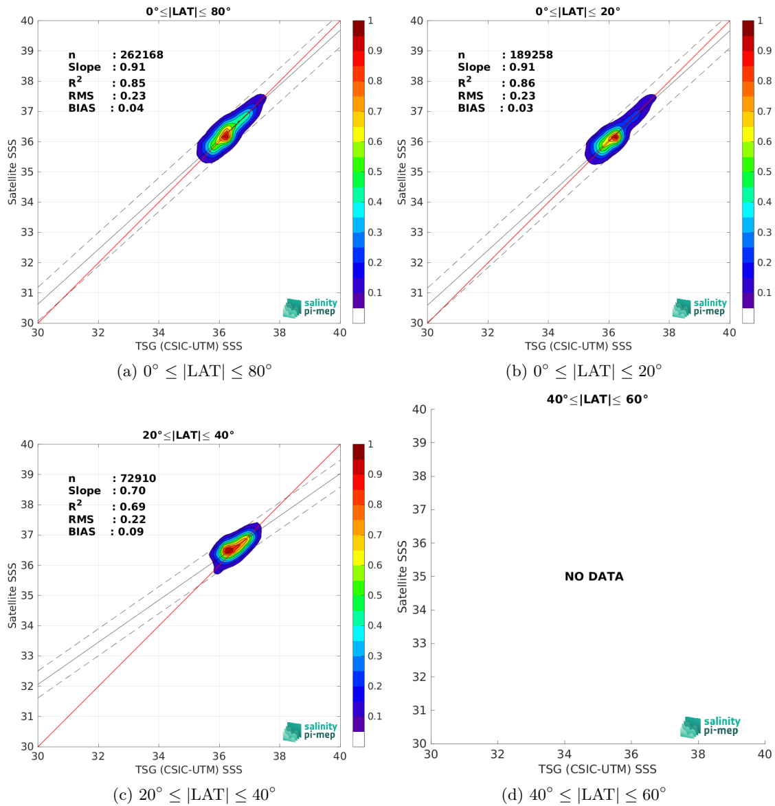
Figure 10: Contour maps of the concentration of SMAP SSS L3 v6 - Monthly (RSS) SSS (y-axis) versus TSG (CSIC-UTM) SSS (x-axis) at match-up pairs for different latitude bands. For each plot, the red line shows x=y . The black thin and dashed lines indicate a linear fit through the data cloud and the \pm 95\% confidence levels, respectively. The number match-up pairs n , the slope and R^2 coefficient of the linear fit, the root mean square (RMS) and the mean bias between satellite and in situ data are indicated for each latitude band in each plots.
