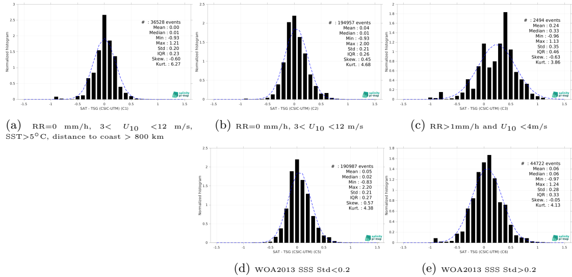
Figure 15: Normalized histogram of \Delta SSS (SMAP SSS L3 v6 - Monthly (RSS) - TSG (CSIC-UTM)) for 5 different subdatasets corresponding to: RR=0 mm/h, 3 < U_{10} < 12 m/s, SST>5°C, distance to coast > 800 km (a), RR=0 mm/h, 3 < U_{10} < 12 m/s (b), RR>1mm/h and U_{10} < 4 m/s (c), WOA2013 SSS Std<0.2 (d), WOA2013 SSS Std>0.2 (e).
