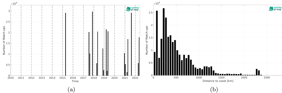
Figure 2: Number of match-ups between TSG (CSIC-UTM) and SMAP SSS L3 v6 - Monthly (RSS) SSS as a function of time (a) and as function of the distance to coast (b) over the Tropical Atlantic Ocean Pi-MEP region and for the full satellite product period.
