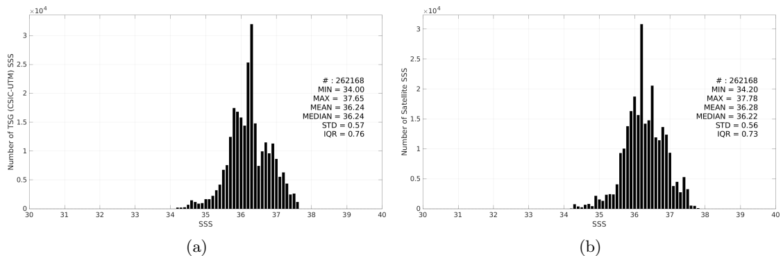
Figure 3: Histograms of SSS from TSG (CSIC-UTM) (a) and SMAP SSS L3 v6 - Monthly (RSS) (b) considering all match-up pairs per bins of 0.1 over the Tropical Atlantic Ocean Pi-MEP region and for the full satellite product period.
