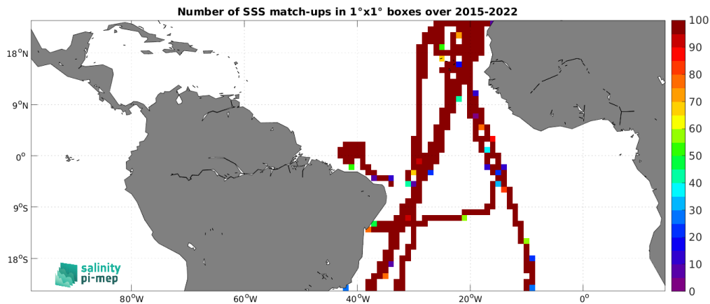
Figure 5: Number of SSS match-ups between TSG (CSIC-UTM) SSS and the SMAP SSS L3 v6 - Monthly (RSS) SSS product for the Tropical Atlantic Ocean Pi-MEP region over 1^\circ \times 1^\circ boxes and for the full satellite product period.
