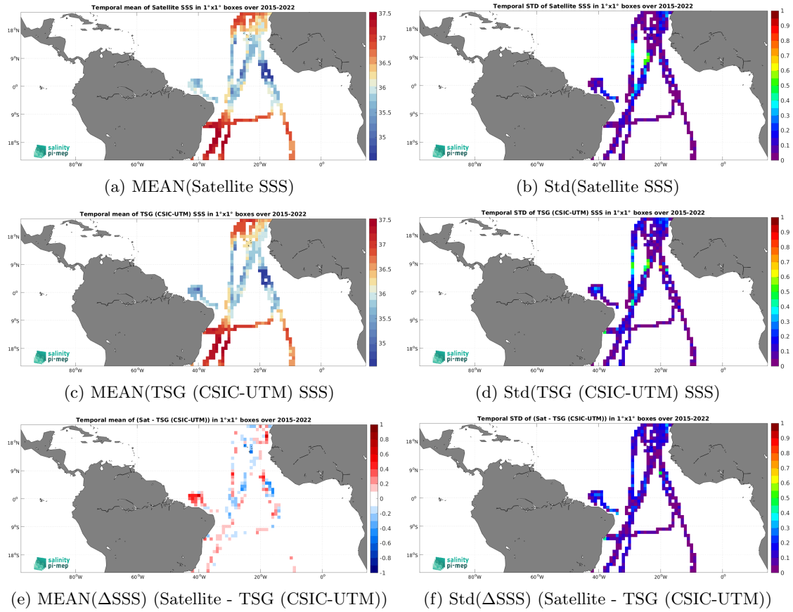
Figure 7: Temporal mean (left) and Std (right) of SSS from SMAP SSS L3 v6 - Monthly (RSS) (top), TSG (CSIC-UTM) (middle), and of \Delta SSS (Satellite - TSG (CSIC-UTM)). Only match-up pairs are used to generate these maps.
