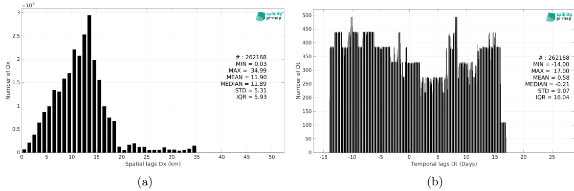
Figure 6: Histograms of the spatial (a) and temporal (b) lags between the location/time of the TSG (CSIC-UTM) measurement and the date of the corresponding SMAP SSS L3 v6 - Monthly (RSS) SSS pixel.
