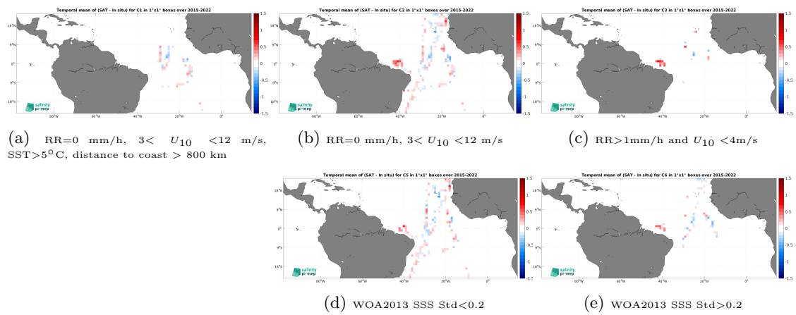
Figure 14: Temporal mean gridded over spatial boxes of size 1^\circ \times 1^\circ of \Delta\text{SSS} (SMAP SSS L3 v6 - Monthly (RSS) - TSG (CSIC-UTM)) for 5 different subdatasets corresponding to:RR=0 mm/h, 3 < U_{10} < 12 m/s, SST >5^\circ\text{C} , distance to coast > 800 km (a), RR=0 mm/h, 3 < U_{10} < 12 m/s (b), RR >1 mm/h and U_{10} < 4 m/s (c), WOA2013 SSS Std <0.2 (d), WOA2013 SSS Std >0.2 (e).
