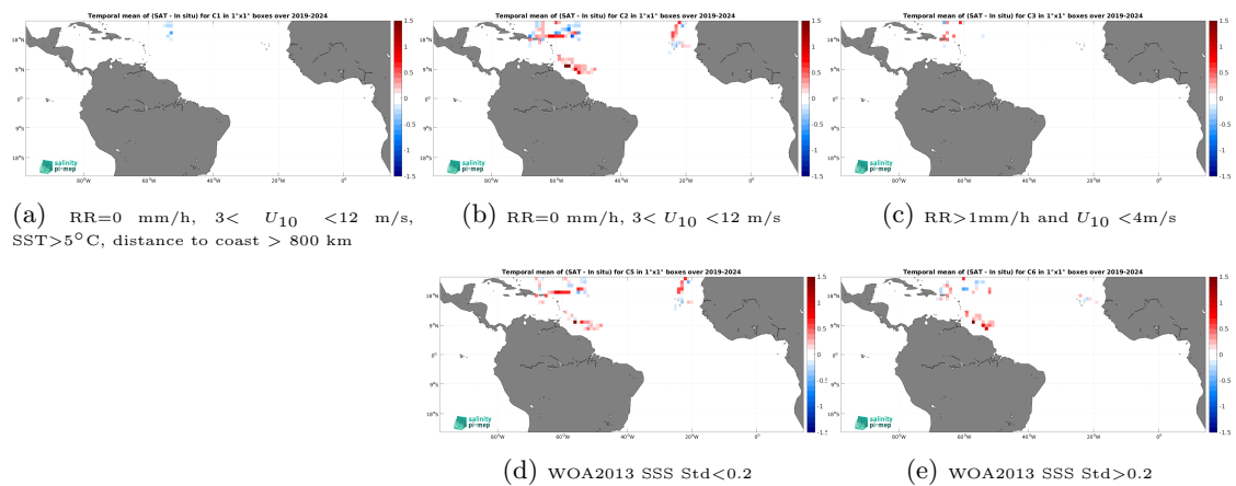
Figure 14: Temporal mean gridded over spatial boxes of size 1^\circ \times 1^\circ of \Delta SSS (SMAP SSS L3 v6 - Monthly (RSS) - Sailydrone) for 5 different subdatasets corresponding to:RR=0 mm/h, 3 < U_{10} < 12 m/s, SST >5^\circ\text{C} , distance to coast > 800 km (a), RR=0 mm/h, 3 < U_{10} < 12 m/s (b), RR >1 mm/h and U_{10} < 4 m/s (c), WOA2013 SSS Std <0.2 (d), WOA2013 SSS Std >0.2 (e).
