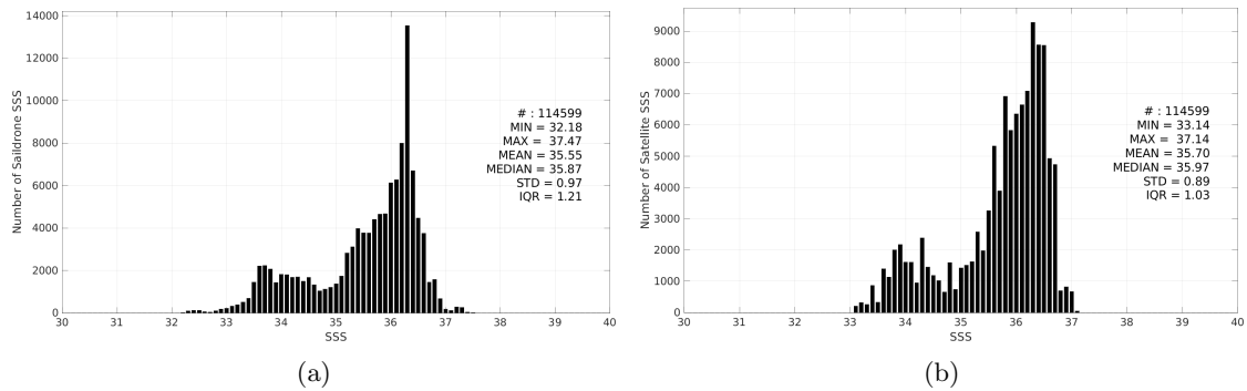
Figure 3: Histograms of SSS from Saildrone (a) and SMAP SSS L3 v6 - Monthly (RSS) (b) considering all match-up pairs per bins of 0.1 over the Tropical Atlantic Ocean Pi-MEP region and for the full satellite product period.
