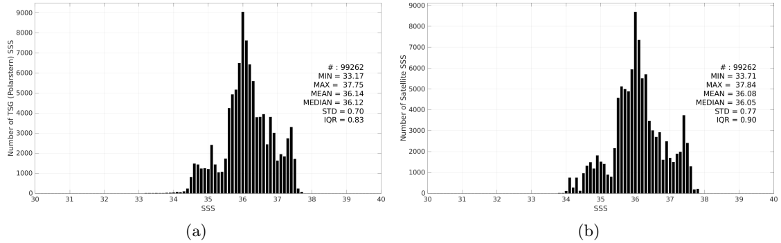
Figure 3: Histograms of SSS from TSG (Polarstern) (a) and SMAP SSS L3 v5.3 - 8-Day running (RSS) (b) considering all match-up pairs per bins of 0.1 over the Tropical Atlantic Ocean Pi-MEP region and for the full satellite product period.
