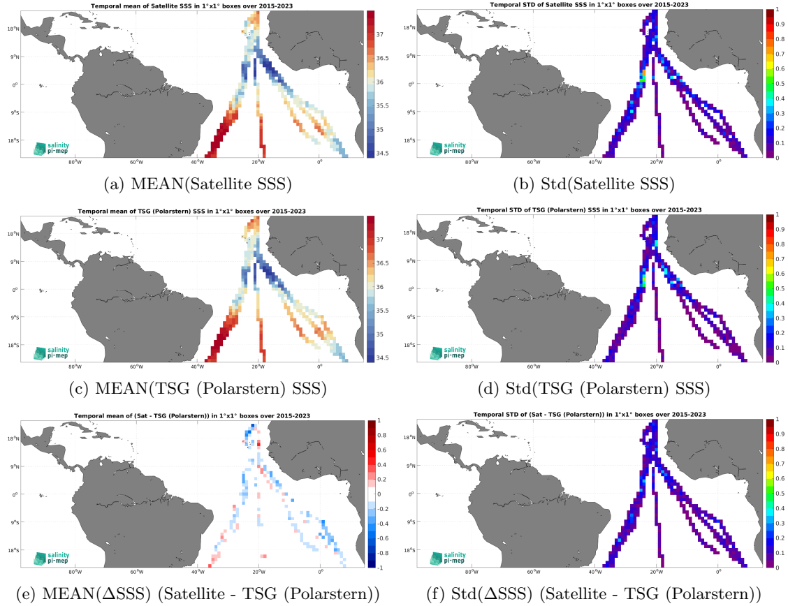
Figure 7: Temporal mean (left) and Std (right) of SSS from SMAP SSS L3 v5.3 - 8-Day running (RSS) (top), TSG (Polarstern) (middle), and of \Delta\text{SSS} (Satellite - TSG (Polarstern)). Only match-up pairs are used to generate these maps.
