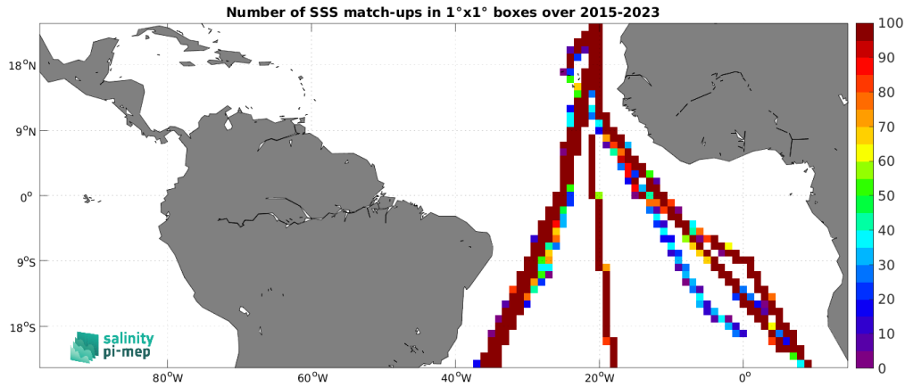
Figure 5: Number of SSS match-ups between TSG (Polarstern) SSS and the SMAP SSS L3 v5.3 - 8-Day running (RSS) SSS product for the Tropical Atlantic Ocean Pi-MEP region over 1^\circ \times 1^\circ boxes and for the full satellite product period.
