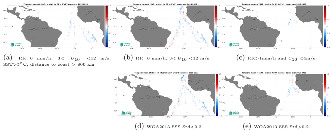
Figure 14: Temporal mean gridded over spatial boxes of size 1^\circ \times 1^\circ of \Delta\text{SSS} (SMAP SSS L3 v5.3 - 8-Day running (RSS) - TSG (Polarstern)) for 5 different subdatasets corresponding to:RR=0 mm/h, 3 < U_{10} < 12 m/s, SST >5^\circ\text{C} , distance to coast > 800 km (a), RR=0 mm/h, 3 < U_{10} < 12 m/s (b), RR >1 mm/h and U_{10} < 4 m/s (c), WOA2013 SSS Std <0.2 (d), WOA2013 SSS Std >0.2 (e).
