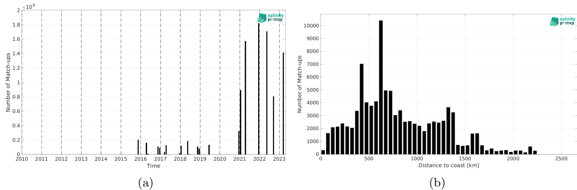
Figure 2: Number of match-ups between TSG (Polarstern) and SMAP SSS L3 v5.3 - 8-Day running (RSS) SSS as a function of time (a) and as function of the distance to coast (b) over the Tropical Atlantic Ocean Pi-MEP region and for the full satellite product period.
