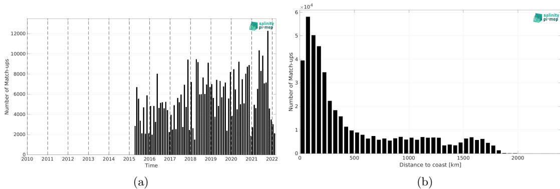
Figure 2: Number of match-ups between TSG (LEGOS-DM) and SMAP SSS L3 v5.3 - 8-Day running (RSS) SSS as a function of time (a) and as function of the distance to coast (b) over the Tropical Atlantic Ocean Pi-MEP region and for the full satellite product period.
