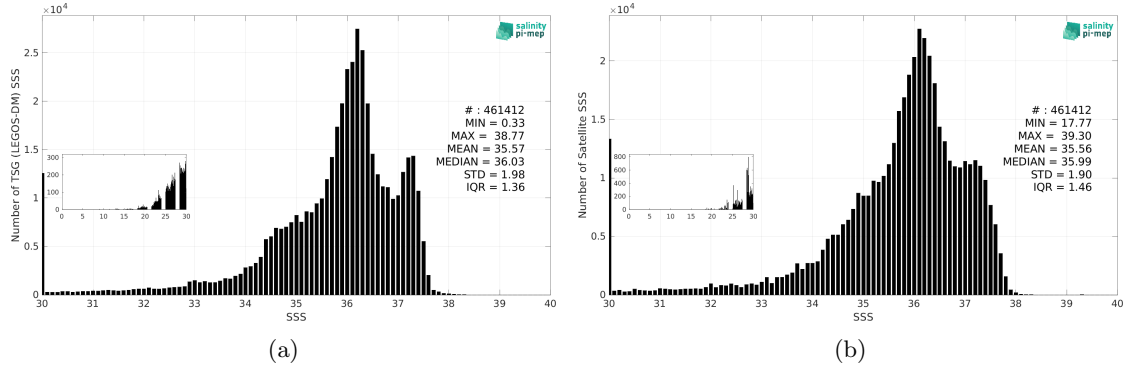
Figure 3: Histograms of SSS from TSG (LEGOS-DM) (a) and SMAP SSS L3 v5.3 - 8-Day running (RSS) (b) considering all match-up pairs per bins of 0.1 over the Tropical Atlantic Ocean Pi-MEP region and for the full satellite product period.
