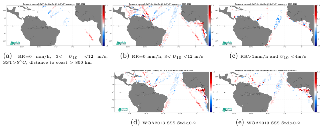
Figure 14: Temporal mean gridded over spatial boxes of size 1^\circ \times 1^\circ of \Delta SSS (SMAP SSS L3 v5.3 - 8-Day running (RSS) - TSG (LEGOS-DM)) for 5 different subdatasets corresponding to:RR=0 mm/h, 3 < U_{10} < 12 m/s, SST >5^\circ C, distance to coast > 800 km (a), RR=0 mm/h, 3 < U_{10} < 12 m/s (b), RR >1 mm/h and U_{10} < 4 m/s (c), WOA2013 SSS Std <0.2 (d), WOA2013 SSS Std >0.2 (e).
