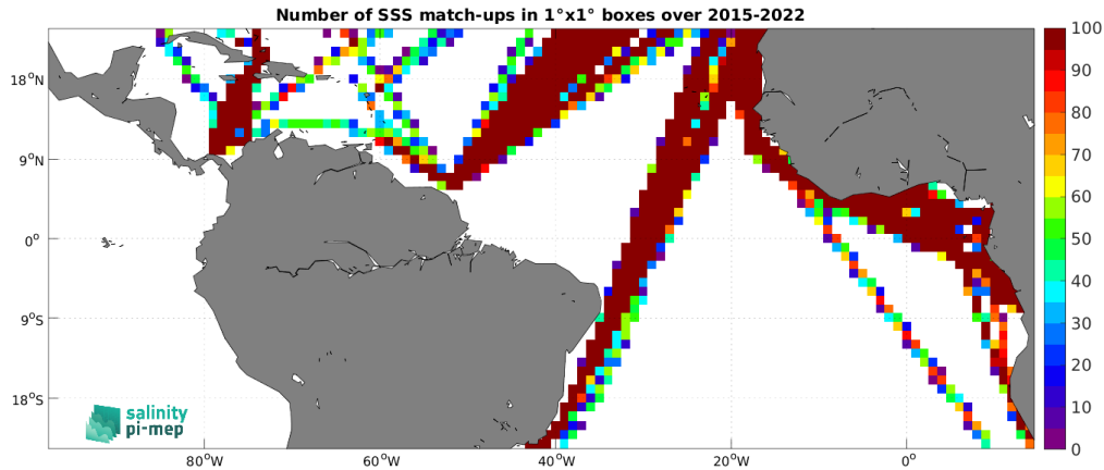
Figure 5: Number of SSS match-ups between TSG (LEGOS-DM) SSS and the SMAP SSS L3 v5.3 - 8-Day running (RSS) SSS product for the Tropical Atlantic Ocean Pi-MEP region over 1^\circ \times 1^\circ boxes and for the full satellite product period.
