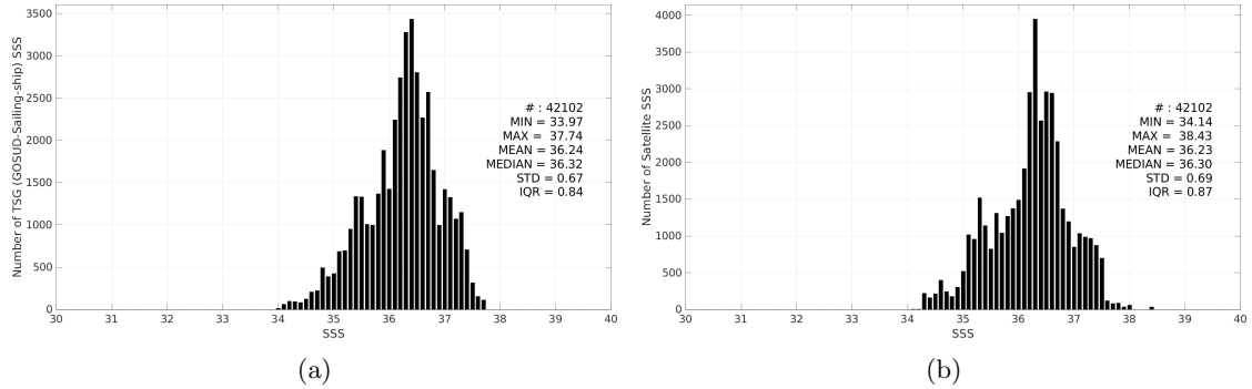
Figure 3: Histograms of SSS from TSG (GOSUD-Sailing-ship) (a) and SMAP SSS L3 v5.3 - 8-Day running (RSS) (b) considering all match-up pairs per bins of 0.1 over the Tropical Atlantic Ocean Pi-MEP region and for the full satellite product period.
