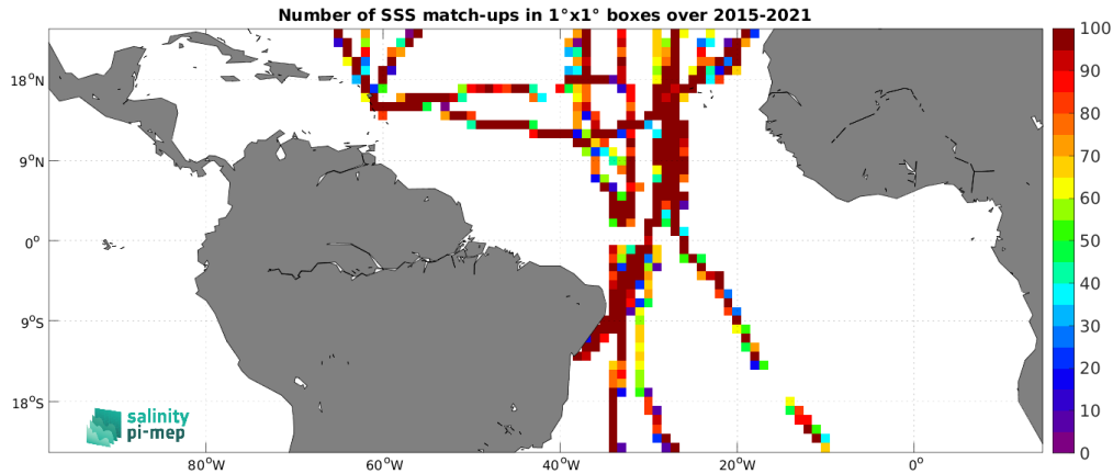
Figure 5: Number of SSS match-ups between TSG (GOSUD-Sailing-ship) SSS and the SMAP SSS L3 v5.3 - 8-Day running (RSS) SSS product for the Tropical Atlantic Ocean Pi-MEP region over 1^\circ \times 1^\circ boxes and for the full satellite product period.
