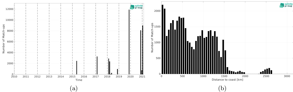
Figure 2: Number of match-ups between TSG (GOSUD-Sailing-ship) and SMAP SSS L3 v5.3 - 8-Day running (RSS) SSS as a function of time (a) and as function of the distance to coast (b) over the Tropical Atlantic Ocean Pi-MEP region and for the full satellite product period.
