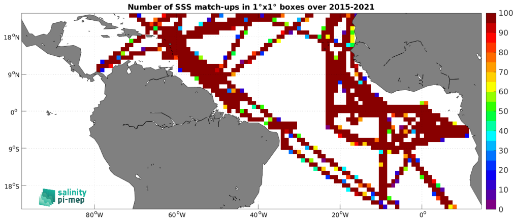
Figure 5: Number of SSS match-ups between TSG (GOSUD-Research-vessel) SSS and the SMAP SSS L3 v5.3 - 8-Day running (RSS) SSS product for the Tropical Atlantic Ocean Pi-MEP region over 1^\circ \times 1^\circ boxes and for the full satellite product period.
