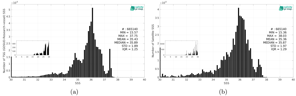
Figure 3: Histograms of SSS from TSG (GOSUD-Research-vessel) (a) and SMAP SSS L3 v5.3 - 8-Day running (RSS) (b) considering all match-up pairs per bins of 0.1 over the Tropical Atlantic Ocean Pi-MEP region and for the full satellite product period.
