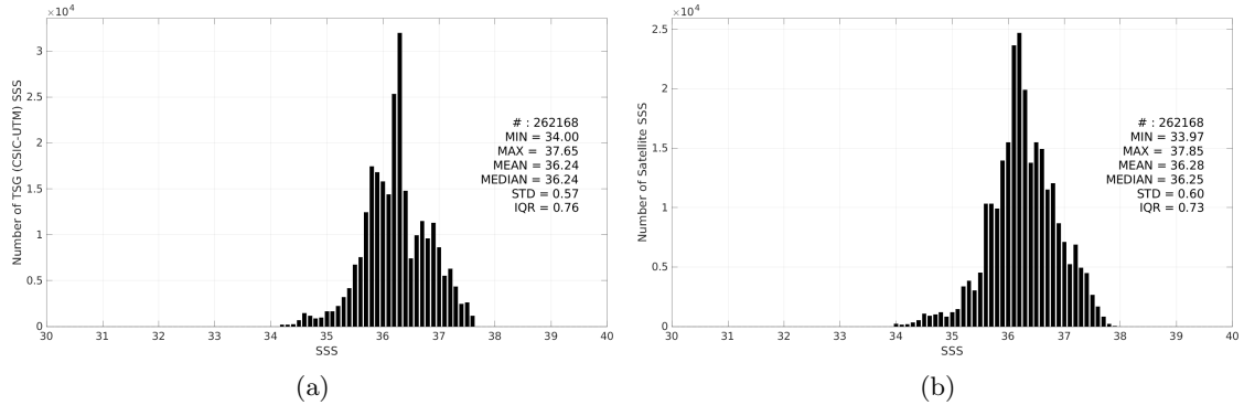
Figure 3: Histograms of SSS from TSG (CSIC-UTM) (a) and SMAP SSS L3 v5.3 - 8-Day running (RSS) (b) considering all match-up pairs per bins of 0.1 over the Tropical Atlantic Ocean Pi-MEP region and for the full satellite product period.
