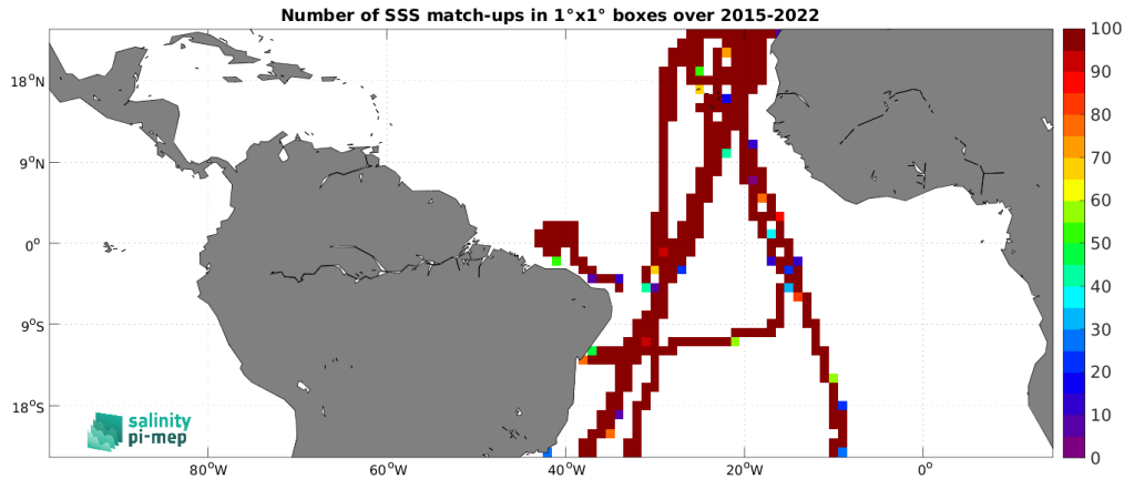
Figure 5: Number of SSS match-ups between TSG (CSIC-UTM) SSS and the SMAP SSS L3 v5.3 - 8-Day running (RSS) SSS product for the Tropical Atlantic Ocean Pi-MEP region over 1^\circ \times 1^\circ boxes and for the full satellite product period.
