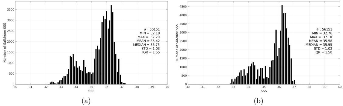
Figure 3: Histograms of SSS from Saildrone (a) and SMAP SSS L3 v5.3 - 8-Day running (RSS) (b) considering all match-up pairs per bins of 0.1 over the Tropical Atlantic Ocean Pi-MEP region and for the full satellite product period.
