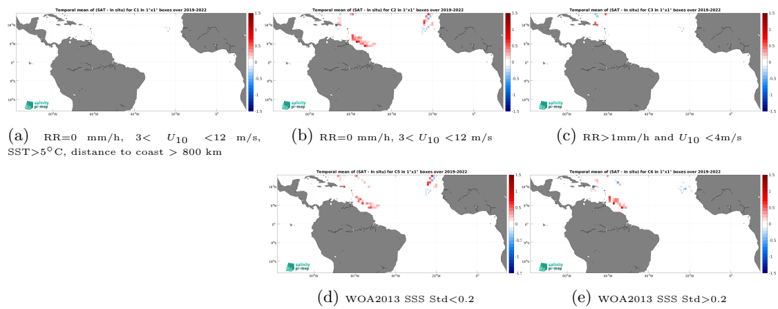
Figure 14: Temporal mean gridded over spatial boxes of size 1^\circ \times 1^\circ of \Delta\text{SSS} (SMAP SSS L3 v5.3 - 8-Day running (RSS) - Saildrone) for 5 different subdatasets corresponding to:RR=0 mm/h, 3 < U_{10} < 12 m/s, SST>5°C, distance to coast > 800 km (a), RR=0 mm/h, 3 < U_{10} < 12 m/s (b), RR>1mm/h and U_{10} < 4 m/s (c), WOA2013 SSS Std<0.2 (d), WOA2013 SSS Std>0.2 (e).
