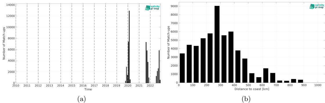
Figure 2: Number of match-ups between Saildrone and SMAP SSS L3 v5.3 - 8-Day running (RSS) SSS as a function of time (a) and as function of the distance to coast (b) over the Tropical Atlantic Ocean Pi-MEP region and for the full satellite product period.
