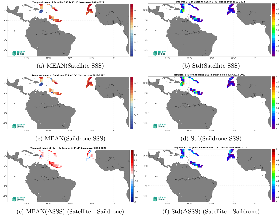
Figure 7: Temporal mean (left) and Std (right) of SSS from SMAP SSS L3 v5.3 - 8-Day running (RSS) (top), Saildrone (middle), and of \Delta SSS (Satellite - Saildrone). Only match-up pairs are used to generate these maps.
