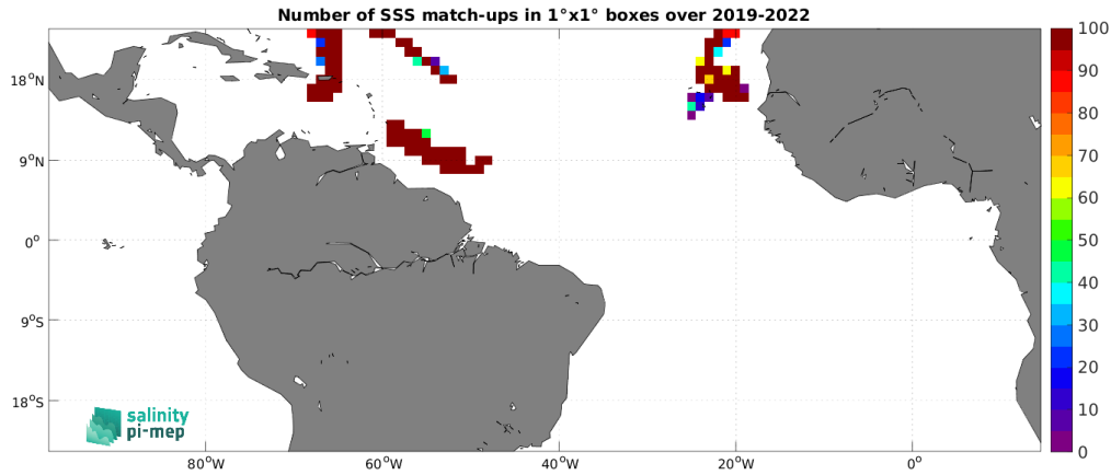
Figure 5: Number of SSS match-ups between Saildrone SSS and the SMAP SSS L3 v5.3 - 8-Day running (RSS) SSS product for the Tropical Atlantic Ocean Pi-MEP region over 1^\circ \times 1^\circ boxes and for the full satellite product period.
