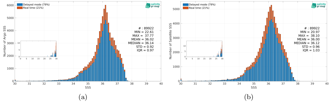
Figure 3: Histograms of SSS from Argo (a) and SMAP SSS L3 v5.3 - 8-Day running (RSS) (b) considering all match-up pairs per bins of 0.1 over the Tropical Atlantic Ocean Pi-MEP region and for the full satellite product period.
