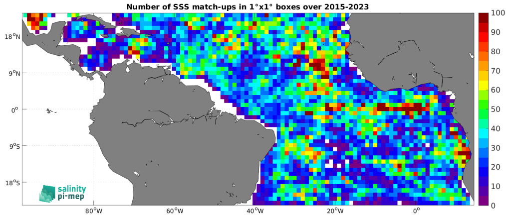
Figure 5: Number of SSS match-ups between Argo SSS and the SMAP SSS L3 v5.3 - 8-Day running (RSS) SSS product for the Tropical Atlantic Ocean Pi-MEP region over 1^\circ \times 1^\circ boxes and for the full satellite product period.
