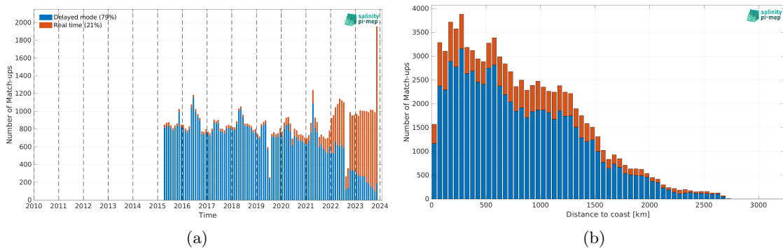
Figure 2: Number of match-ups between Argo and SMAP SSS L3 v5.3 - 8-Day running (RSS) SSS as a function of time (a) and as function of the distance to coast (b) over the Tropical Atlantic Ocean Pi-MEP region and for the full satellite product period.
