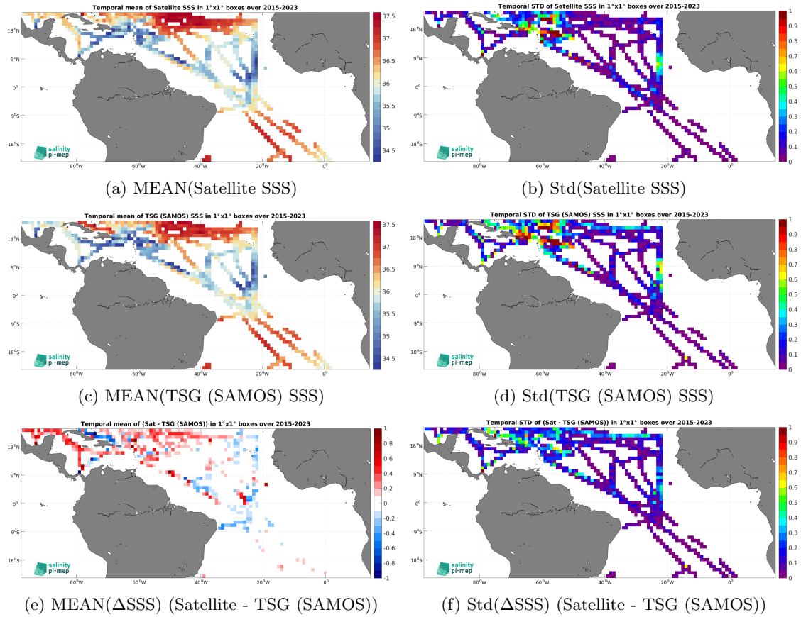
Figure 7: Temporal mean (left) and Std (right) of SSS from SMAP SSS L3 v5.3 - Monthly (RSS) (top), TSG (SAMOS) (middle), and of \Delta\text{SSS} (Satellite - TSG (SAMOS)). Only match-up pairs are used to generate these maps.
