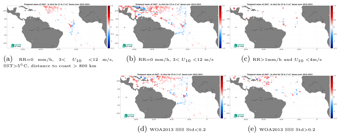
Figure 14: Temporal mean gridded over spatial boxes of size 1^\circ \times 1^\circ of \Delta\text{SSS} (SMAP SSS L3 v5.3 - Monthly (RSS) - TSG (SAMOS)) for 5 different subdatasets corresponding to:RR=0 mm/h, 3 < U_{10} < 12 m/s, SST >5^\circ\text{C} , distance to coast > 800 km (a), RR=0 mm/h, 3 < U_{10} < 12 m/s (b), RR >1 mm/h and U_{10} < 4 m/s (c), WOA2013 SSS Std <0.2 (d), WOA2013 SSS Std >0.2 (e).
