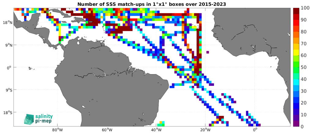
Figure 5: Number of SSS match-ups between TSG (SAMOS) SSS and the SMAP SSS L3 v5.3 - Monthly (RSS) SSS product for the Tropical Atlantic Ocean Pi-MEP region over 1^\circ \times 1^\circ boxes and for the full satellite product period.
