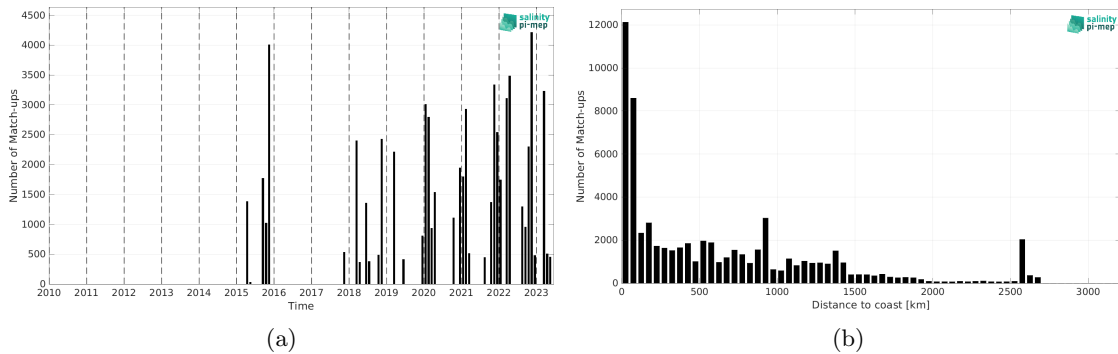
Figure 2: Number of match-ups between TSG (SAMOS) and SMAP SSS L3 v5.3 - Monthly (RSS) SSS as a function of time (a) and as function of the distance to coast (b) over the Tropical Atlantic Ocean Pi-MEP region and for the full satellite product period.
