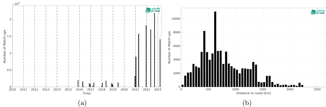
Figure 2: Number of match-ups between TSG (Polarstern) and SMAP SSS L3 v5.3 - Monthly (RSS) SSS as a function of time (a) and as function of the distance to coast (b) over the Tropical Atlantic Ocean Pi-MEP region and for the full satellite product period.
