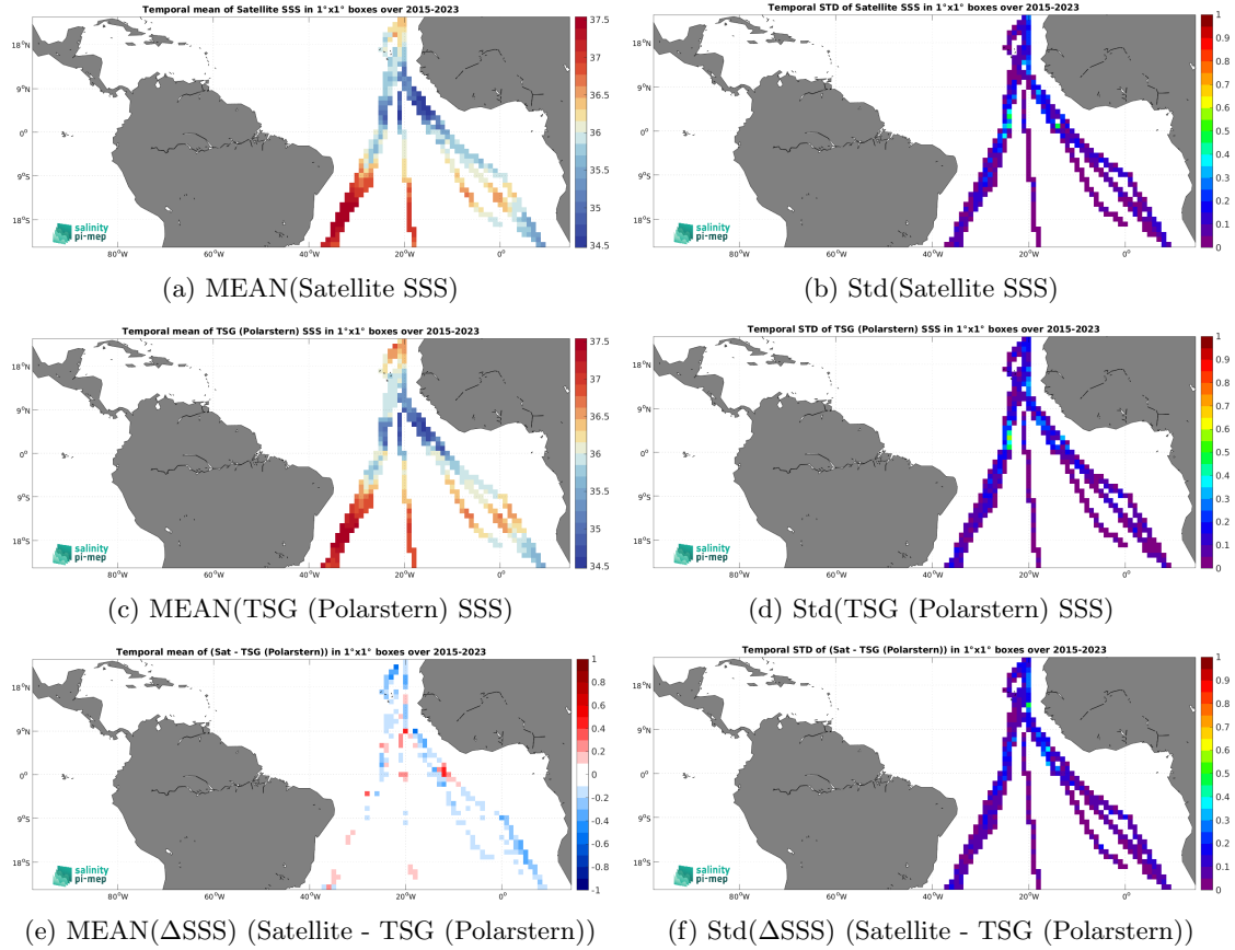
Figure 7: Temporal mean (left) and Std (right) of SSS from SMAP SSS L3 v5.3 - Monthly (RSS) (top), TSG (Polarstern) (middle), and of \Delta\text{SSS} (Satellite - TSG (Polarstern)). Only match-up pairs are used to generate these maps.
