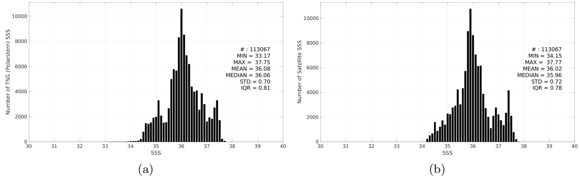
Figure 3: Histograms of SSS from TSG (Polarstern) (a) and SMAP SSS L3 v5.3 - Monthly (RSS) (b) considering all match-up pairs per bins of 0.1 over the Tropical Atlantic Ocean Pi-MEP region and for the full satellite product period.
