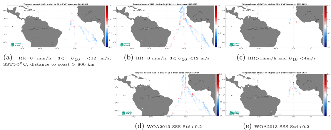
Figure 14: Temporal mean gridded over spatial boxes of size 1^\circ \times 1^\circ of \Delta\text{SSS} (SMAP SSS L3 v5.3 - Monthly (RSS) - TSG (Polarstern)) for 5 different subdatasets corresponding to:RR=0 mm/h, 3 < U_{10} < 12 m/s, SST >5^\circ\text{C} , distance to coast > 800 km (a), RR=0 mm/h, 3 < U_{10} < 12 m/s (b), RR >1 mm/h and U_{10} < 4 m/s (c), WOA2013 SSS Std <0.2 (d), WOA2013 SSS Std >0.2 (e).
