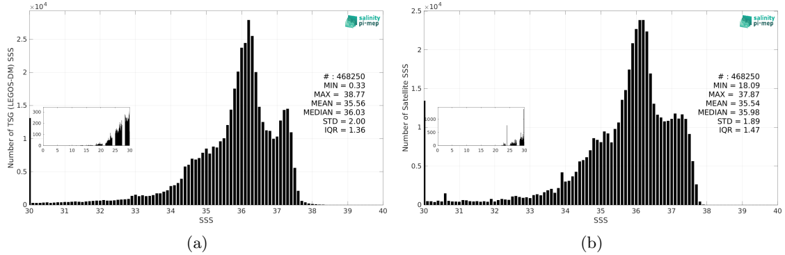
Figure 3: Histograms of SSS from TSG (LEGOS-DM) (a) and SMAP SSS L3 v5.3 - Monthly (RSS) (b) considering all match-up pairs per bins of 0.1 over the Tropical Atlantic Ocean Pi-MEP region and for the full satellite product period.
