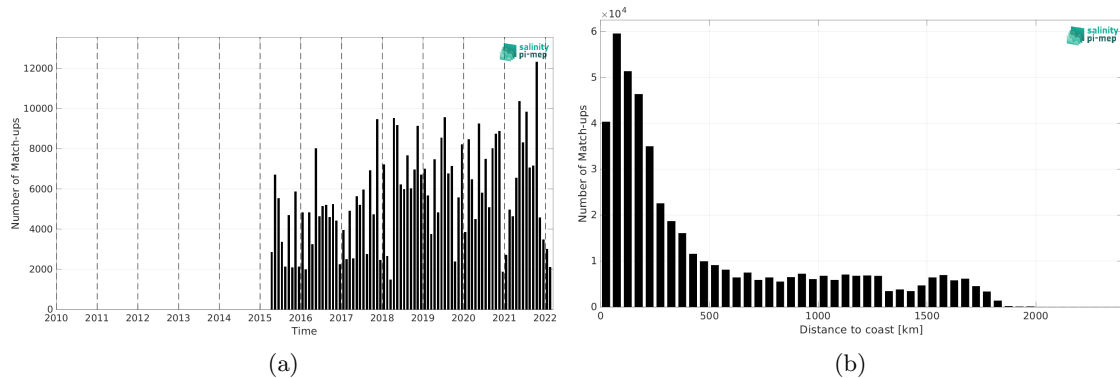
Figure 2: Number of match-ups between TSG (LEGOS-DM) and SMAP SSS L3 v5.3 - Monthly (RSS) SSS as a function of time (a) and as function of the distance to coast (b) over the Tropical Atlantic Ocean Pi-MEP region and for the full satellite product period.
