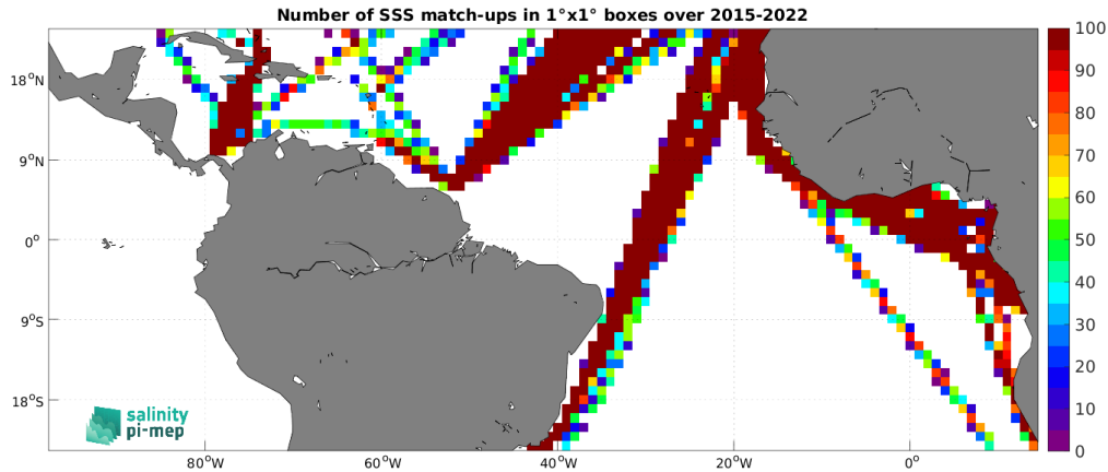
Figure 5: Number of SSS match-ups between TSG (LEGOS-DM) SSS and the SMAP SSS L3 v5.3 - Monthly (RSS) SSS product for the Tropical Atlantic Ocean Pi-MEP region over 1^\circ \times 1^\circ boxes and for the full satellite product period.
