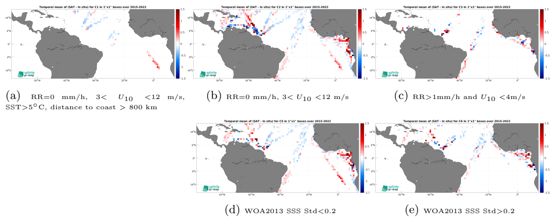
Figure 14: Temporal mean gridded over spatial boxes of size 1^\circ \times 1^\circ of \Delta\text{SSS} (SMAP SSS L3 v5.3 - Monthly (RSS) - TSG (LEGOS-DM)) for 5 different subdatasets corresponding to:RR=0 mm/h, 3 < U_{10} < 12 m/s, SST >5^\circ\text{C} , distance to coast > 800 km (a), RR=0 mm/h, 3 < U_{10} < 12 m/s (b), RR >1 mm/h and U_{10} < 4 m/s (c), WOA2013 SSS Std <0.2 (d), WOA2013 SSS Std >0.2 (e).
