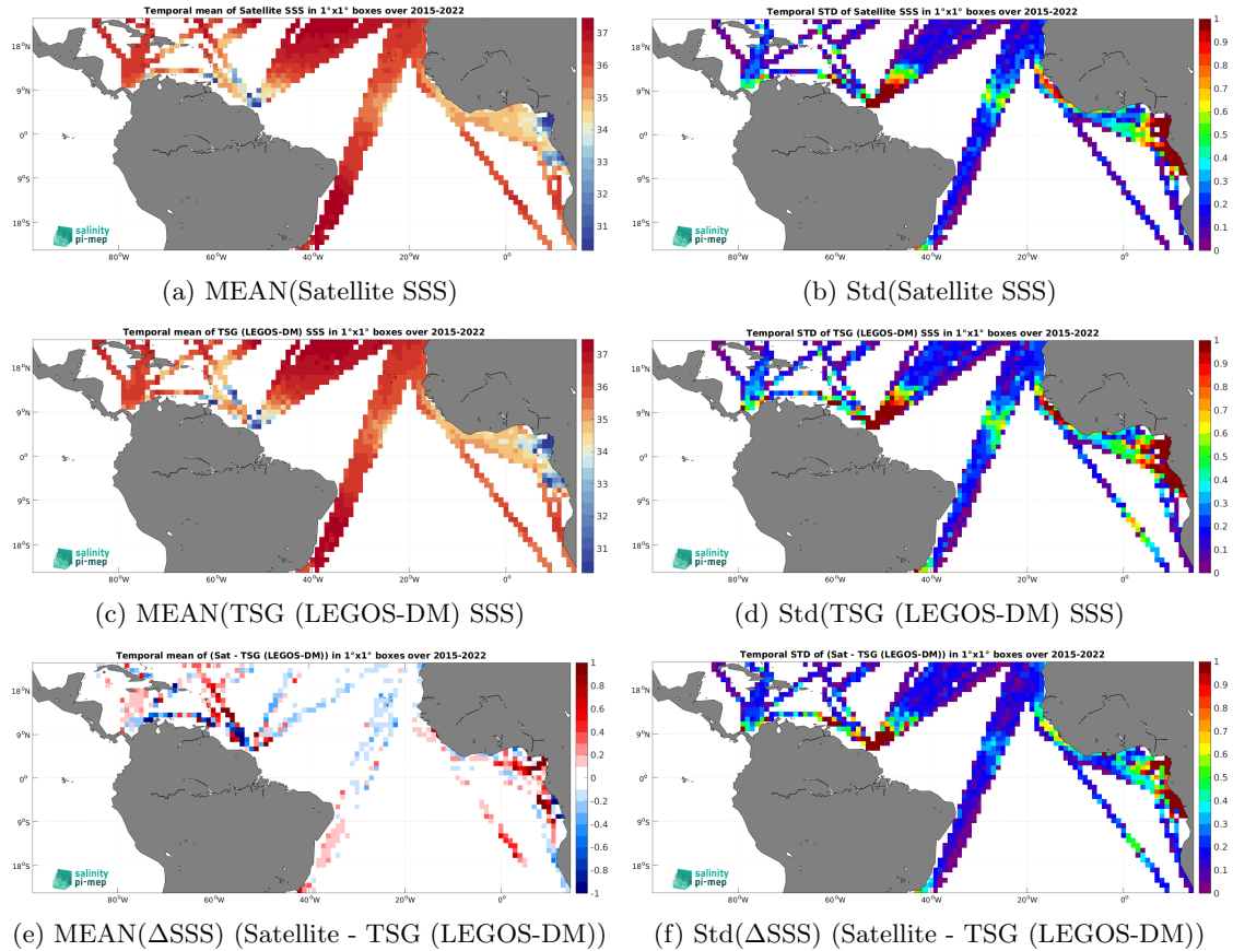
Figure 7: Temporal mean (left) and Std (right) of SSS from SMAP SSS L3 v5.3 - Monthly (RSS) (top), TSG (LEGOS-DM) (middle), and of \Delta\text{SSS} (Satellite - TSG (LEGOS-DM)). Only match-up pairs are used to generate these maps.
