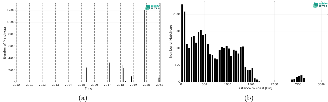
Figure 2: Number of match-ups between TSG (GOSUD-Sailing-ship) and SMAP SSS L3 v5.3 - Monthly (RSS) SSS as a function of time (a) and as function of the distance to coast (b) over the Tropical Atlantic Ocean Pi-MEP region and for the full satellite product period.
