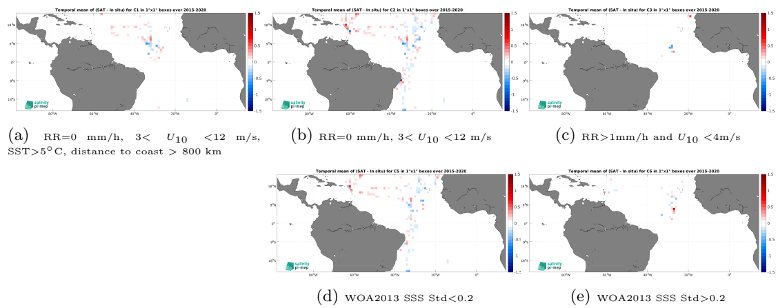
Figure 14: Temporal mean gridded over spatial boxes of size 1^\circ \times 1^\circ of \Delta\text{SSS} (SMAP SSS L3 v5.3 - Monthly (RSS) - TSG (GOSUD-Sailing-ship)) for 5 different subdatasets corresponding to:RR=0 mm/h, 3 < U_{10} < 12 m/s, SST >5^\circ\text{C} , distance to coast > 800 km (a), RR=0 mm/h, 3 < U_{10} < 12 m/s (b), RR >1 mm/h and U_{10} < 4 m/s (c), WOA2013 SSS Std <0.2 (d), WOA2013 SSS Std >0.2 (e).
