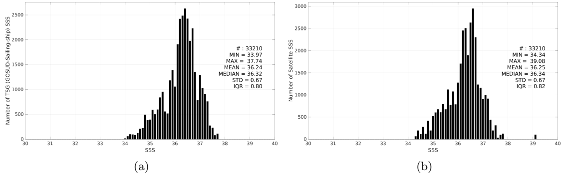
Figure 3: Histograms of SSS from TSG (GOSUD-Sailing-ship) (a) and SMAP SSS L3 v5.3 - Monthly (RSS) (b) considering all match-up pairs per bins of 0.1 over the Tropical Atlantic Ocean Pi-MEP region and for the full satellite product period.
