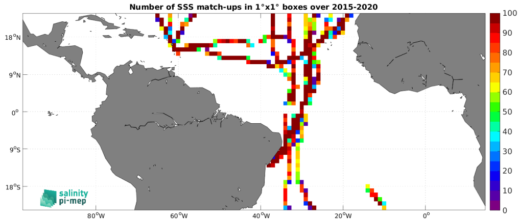
Figure 5: Number of SSS match-ups between TSG (GOSUD-Sailing-ship) SSS and the SMAP SSS L3 v5.3 - Monthly (RSS) SSS product for the Tropical Atlantic Ocean Pi-MEP region over 1^\circ \times 1^\circ boxes and for the full satellite product period.
