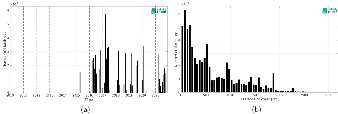
Figure 2: Number of match-ups between TSG (GOSUD-Research-vessel) and SMAP SSS L3 v5.3 - Monthly (RSS) SSS as a function of time (a) and as function of the distance to coast (b) over the Tropical Atlantic Ocean Pi-MEP region and for the full satellite product period.
