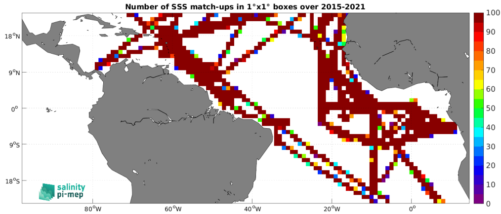
Figure 5: Number of SSS match-ups between TSG (GOSUD-Research-vessel) SSS and the SMAP SSS L3 v5.3 - Monthly (RSS) SSS product for the Tropical Atlantic Ocean Pi-MEP region over 1^\circ \times 1^\circ boxes and for the full satellite product period.
