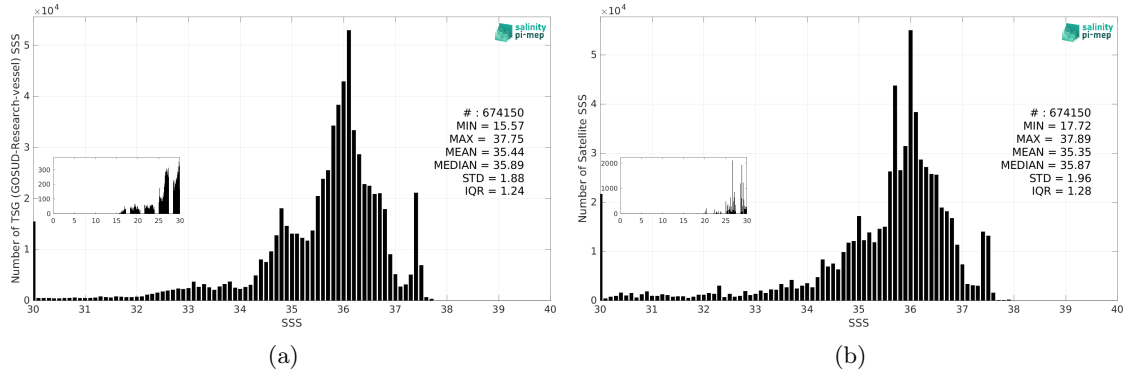
Figure 3: Histograms of SSS from TSG (GOSUD-Research-vessel) (a) and SMAP SSS L3 v5.3 - Monthly (RSS) (b) considering all match-up pairs per bins of 0.1 over the Tropical Atlantic Ocean Pi-MEP region and for the full satellite product period.
