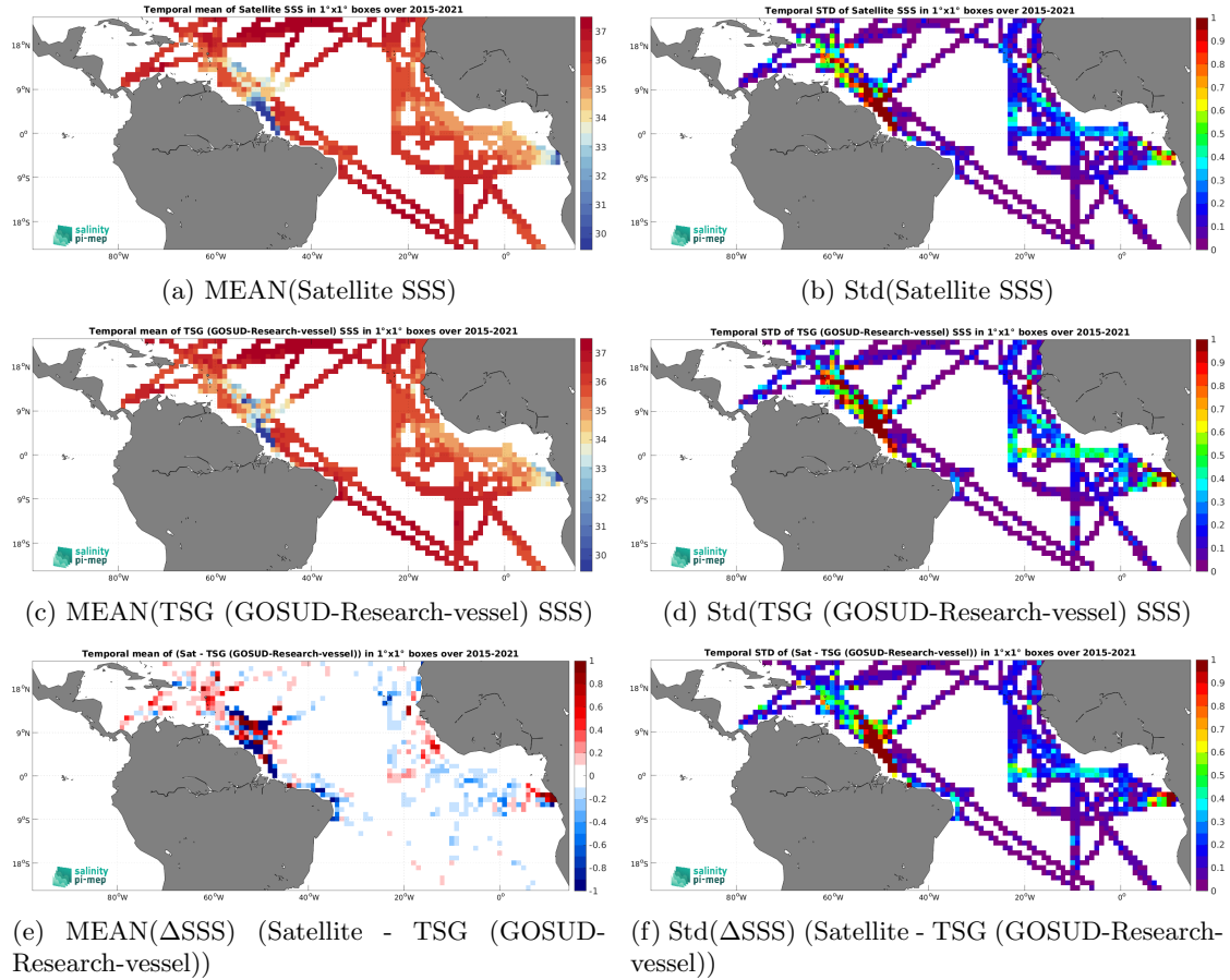
Figure 7: Temporal mean (left) and Std (right) of SSS from SMAP SSS L3 v5.3 - Monthly (RSS) (top), TSG (GOSUD-Research-vessel) (middle), and of \Delta\text{SSS} (Satellite - TSG (GOSUD-Research-vessel)). Only match-up pairs are used to generate these maps.
