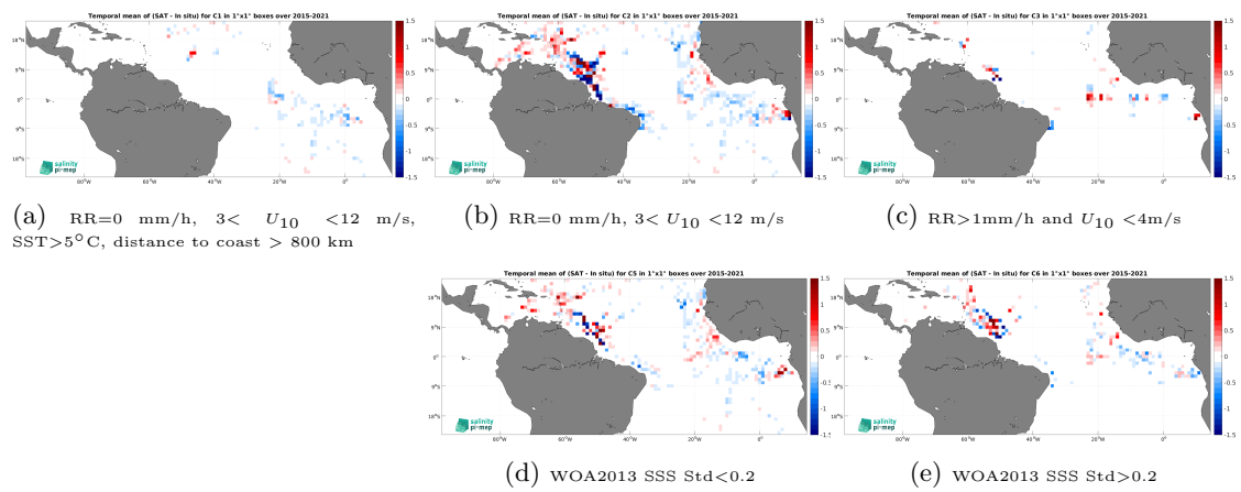
Figure 14: Temporal mean gridded over spatial boxes of size 1^\circ \times 1^\circ of \Delta\text{SSS} (SMAP SSS L3 v5.3 - Monthly (RSS) - TSG (GOSUD-Research-vessel)) for 5 different subdatasets corresponding to:RR=0 mm/h, 3 < U_{10} < 12 m/s, SST >5^\circ\text{C} , distance to coast > 800 km (a), RR=0 mm/h, 3 < U_{10} < 12 m/s (b), RR >1 mm/h and U_{10} < 4 m/s (c), WOA2013 SSS Std <0.2 (d), WOA2013 SSS Std >0.2 (e).
