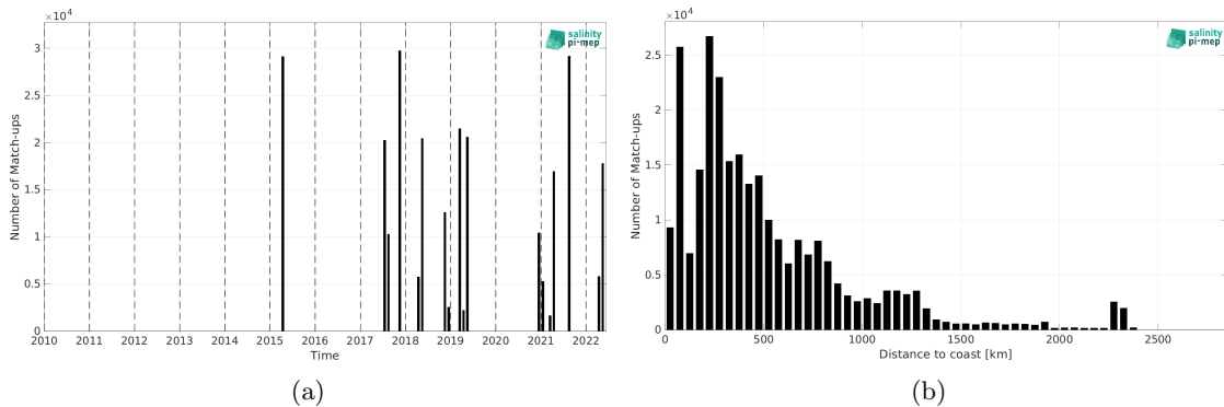
Figure 2: Number of match-ups between TSG (CSIC-UTM) and SMAP SSS L3 v5.3 - Monthly (RSS) SSS as a function of time (a) and as function of the distance to coast (b) over the Tropical Atlantic Ocean Pi-MEP region and for the full satellite product period.
