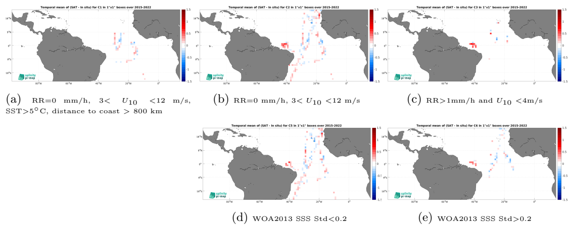
Figure 14: Temporal mean gridded over spatial boxes of size 1^\circ \times 1^\circ of \Delta SSS (SMAP SSS L3 v5.3 - Monthly (RSS) - TSG (CSIC-UTM)) for 5 different subdatasets corresponding to:RR=0 mm/h, 3 < U_{10} < 12 m/s, SST >5^\circ\text{C} , distance to coast > 800 km (a), RR=0 mm/h, 3 < U_{10} < 12 m/s (b), RR >1 mm/h and U_{10} < 4 m/s (c), WOA2013 SSS Std <0.2 (d), WOA2013 SSS Std >0.2 (e).
