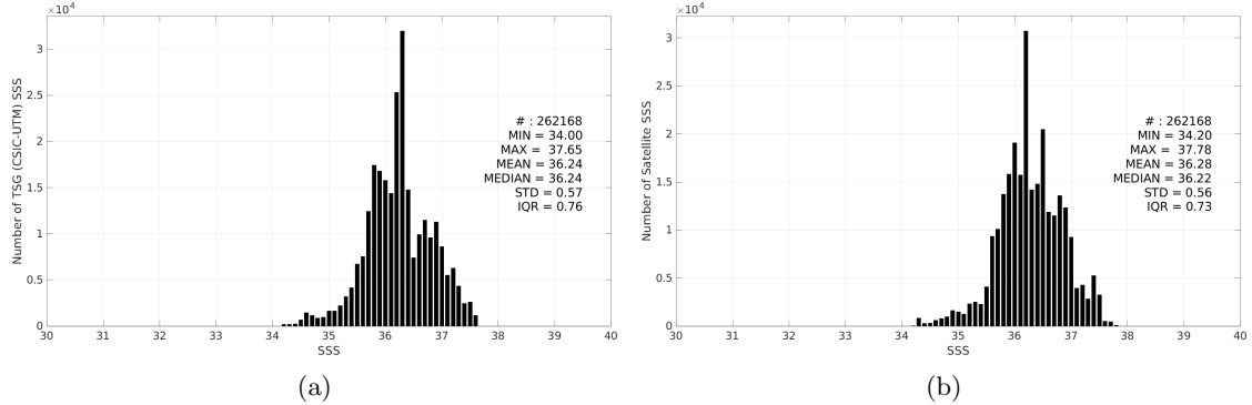
Figure 3: Histograms of SSS from TSG (CSIC-UTM) (a) and SMAP SSS L3 v5.3 - Monthly (RSS) (b) considering all match-up pairs per bins of 0.1 over the Tropical Atlantic Ocean Pi-MEP region and for the full satellite product period.
