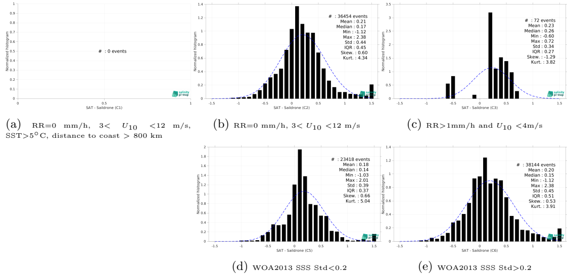
Figure 15: Normalized histogram of \Delta SSS (SMAP SSS L3 v5.3 - Monthly (RSS) - Saldrone) for 5 different subdatasets corresponding to: RR=0 mm/h, 3 < U_{10} < 12 m/s, SST > 5°C, distance to coast > 800 km (a), RR=0 mm/h, 3 < U_{10} < 12 m/s (b), RR > 1mm/h and U_{10} < 4 m/s (c), WOA2013 SSS Std < 0.2 (d), WOA2013 SSS Std > 0.2 (e).
