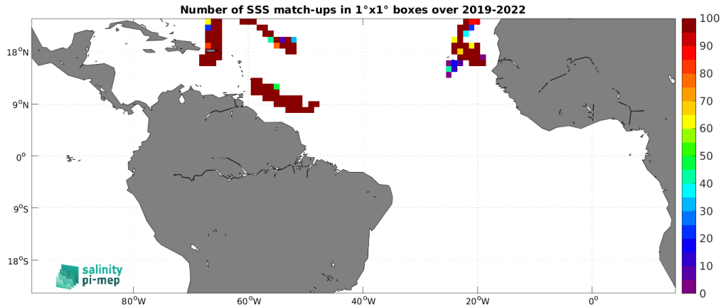
Figure 5: Number of SSS match-ups between Saildrone SSS and the SMAP SSS L3 v5.3 - Monthly (RSS) SSS product for the Tropical Atlantic Ocean Pi-MEP region over 1^\circ \times 1^\circ boxes and for the full satellite product period.
