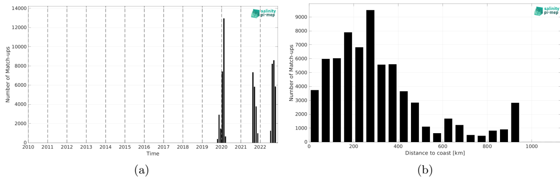
Figure 2: Number of match-ups between Saildrone and SMAP SSS L3 v5.3 - Monthly (RSS) SSS as a function of time (a) and as function of the distance to coast (b) over the Tropical Atlantic Ocean Pi-MEP region and for the full satellite product period.
