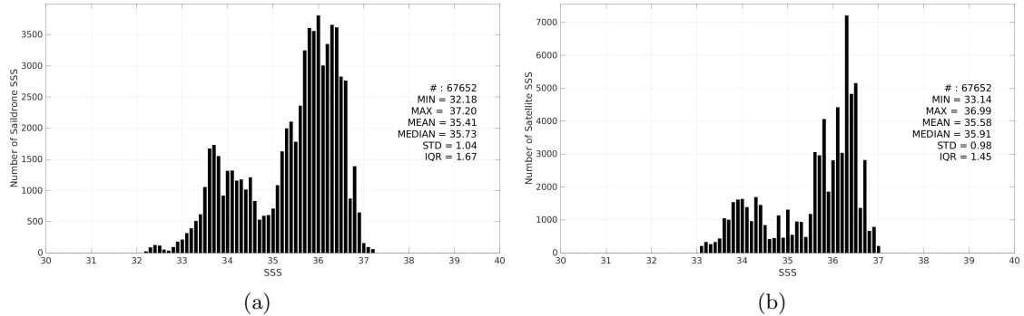
Figure 3: Histograms of SSS from Saildrone (a) and SMAP SSS L3 v5.3 - Monthly (RSS) (b) considering all match-up pairs per bins of 0.1 over the Tropical Atlantic Ocean Pi-MEP region and for the full satellite product period.
