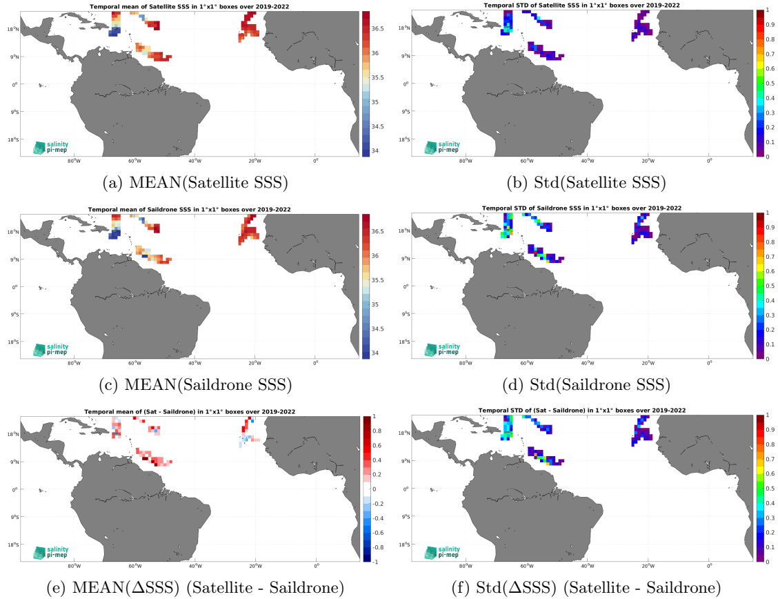
Figure 7: Temporal mean (left) and Std (right) of SSS from SMAP SSS L3 v5.3 - Monthly (RSS) (top), Saildrone (middle), and of \Delta\text{SSS} (Satellite - Saildrone). Only match-up pairs are used to generate these maps.
