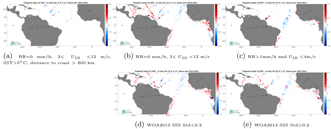
Figure 12: Temporal mean gridded over spatial boxes of size 1^\circ \times 1^\circ of \Delta\text{SSS} (SMAP SSS L3 v5 - 8-Day running (RSS) - TSG (LEGOS-DM)) for 5 different subdatasets corresponding to:RR=0 mm/h, 3 < U_{10} < 12 m/s, SST >5^\circ\text{C} , distance to coast > 800 km (a), RR=0 mm/h, 3 < U_{10} < 12 m/s (b), RR >1 mm/h and U_{10} < 4 m/s (c), WOA2013 SSS Std <0.2 (d), WOA2013 SSS Std >0.2 (e).
