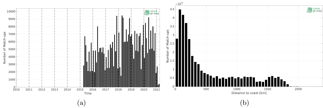
Figure 1: Number of match-ups between TSG (LEGOS-DM) and SMAP SSS L3 v5 - 8-Day running (RSS) SSS as a function of time (a) and as function of the distance to coast (b) over the Tropical Atlantic Ocean Pi-MEP region and for the full satellite product period.
