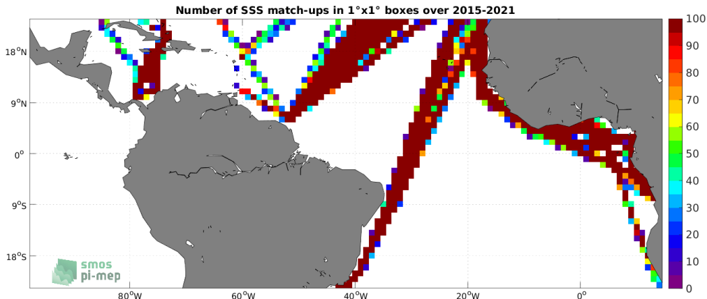
Figure 4: Number of SSS match-ups between TSG (LEGOS-DM) SSS and the SMAP SSS L3 v5 - 8-Day running (RSS) SSS product for the Tropical Atlantic Ocean Pi-MEP region over 1^\circ \times 1^\circ boxes and for the full satellite product period.
