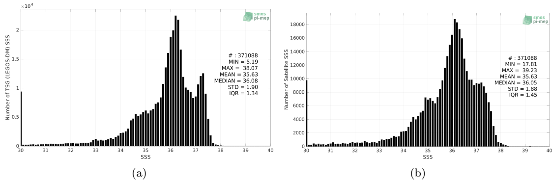
Figure 2: Histograms of SSS from TSG (LEGOS-DM) (a) and SMAP SSS L3 v5 - 8-Day running (RSS) (b) considering all match-up pairs per bins of 0.1 over the Tropical Atlantic Ocean Pi-MEP region and for the full satellite product period.
