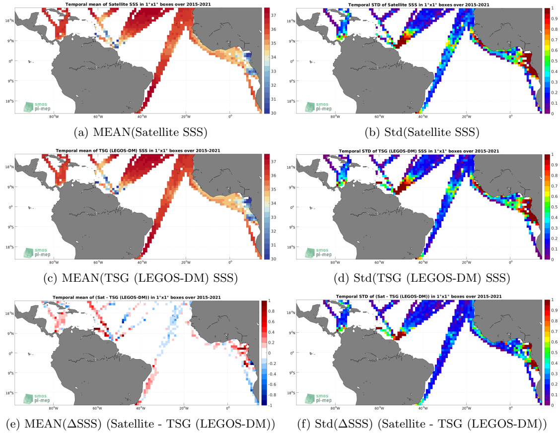
Figure 6: Temporal mean (left) and Std (right) of SSS from SMAP SSS L3 v5 - 8-Day running (RSS) (top), TSG (LEGOS-DM) (middle), and of \Delta SSS (Satellite - TSG (LEGOS-DM)). Only match-up pairs are used to generate these maps.
