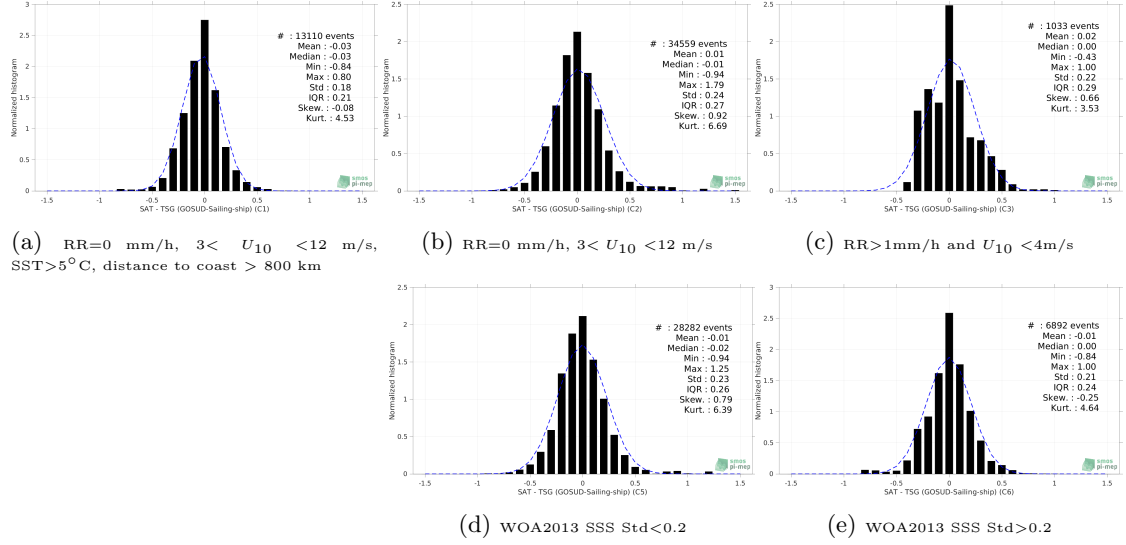
Figure 13: Normalized histogram of \Delta SSS (SMAP SSS L3 v5 - 8-Day running (RSS) - TSG (GOSUD-Sailing-ship)) for 5 different subdatasets corresponding to: RR=0 mm/h, 3 < U_{10} < 12 m/s, SST > 5°C, distance to coast > 800 km (a), RR=0 mm/h, 3 < U_{10} < 12 m/s (b), RR > 1mm/h and U_{10} < 4 m/s (c), WOA2013 SSS Std < 0.2 (d), WOA2013 SSS Std > 0.2 (e).
