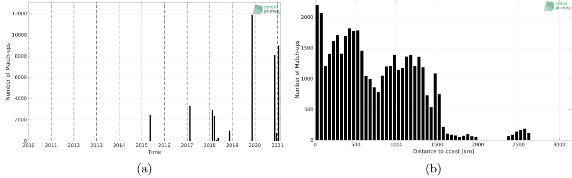
Figure 1: Number of match-ups between TSG (GOSUD-Sailing-ship) and SMAP SSS L3 v5 - 8-Day running (RSS) SSS as a function of time (a) and as function of the distance to coast (b) over the Tropical Atlantic Ocean Pi-MEP region and for the full satellite product period.
