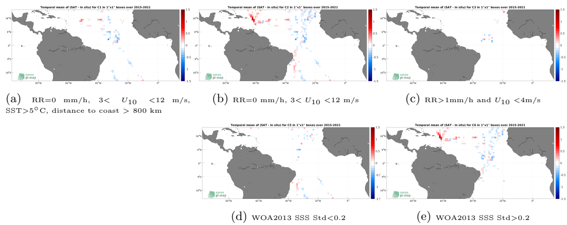
Figure 12: Temporal mean gridded over spatial boxes of size 1^\circ \times 1^\circ of \Delta SSS (SMAP SSS L3 v5 - 8-Day running (RSS) - TSG (GOSUD-Sailing-ship)) for 5 different subdatasets corresponding to:RR=0 mm/h, 3 < U_{10} < 12 m/s, SST>5°C, distance to coast > 800 km (a), RR=0 mm/h, 3 < U_{10} < 12 m/s (b), RR>1mm/h and U_{10} < 4 m/s (c), WOA2013 SSS Std<0.2 (d), WOA2013 SSS Std>0.2 (e).
