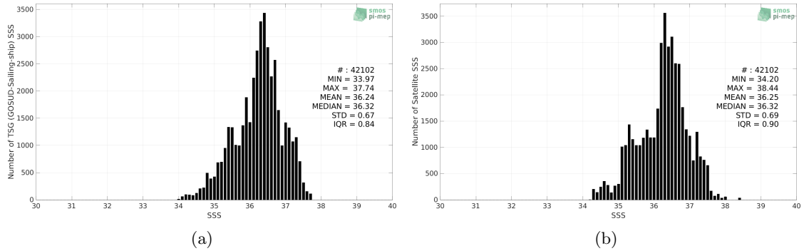
Figure 2: Histograms of SSS from TSG (GOSUD-Sailing-ship) (a) and SMAP SSS L3 v5 - 8-Day running (RSS) (b) considering all match-up pairs per bins of 0.1 over the Tropical Atlantic Ocean Pi-MEP region and for the full satellite product period.
