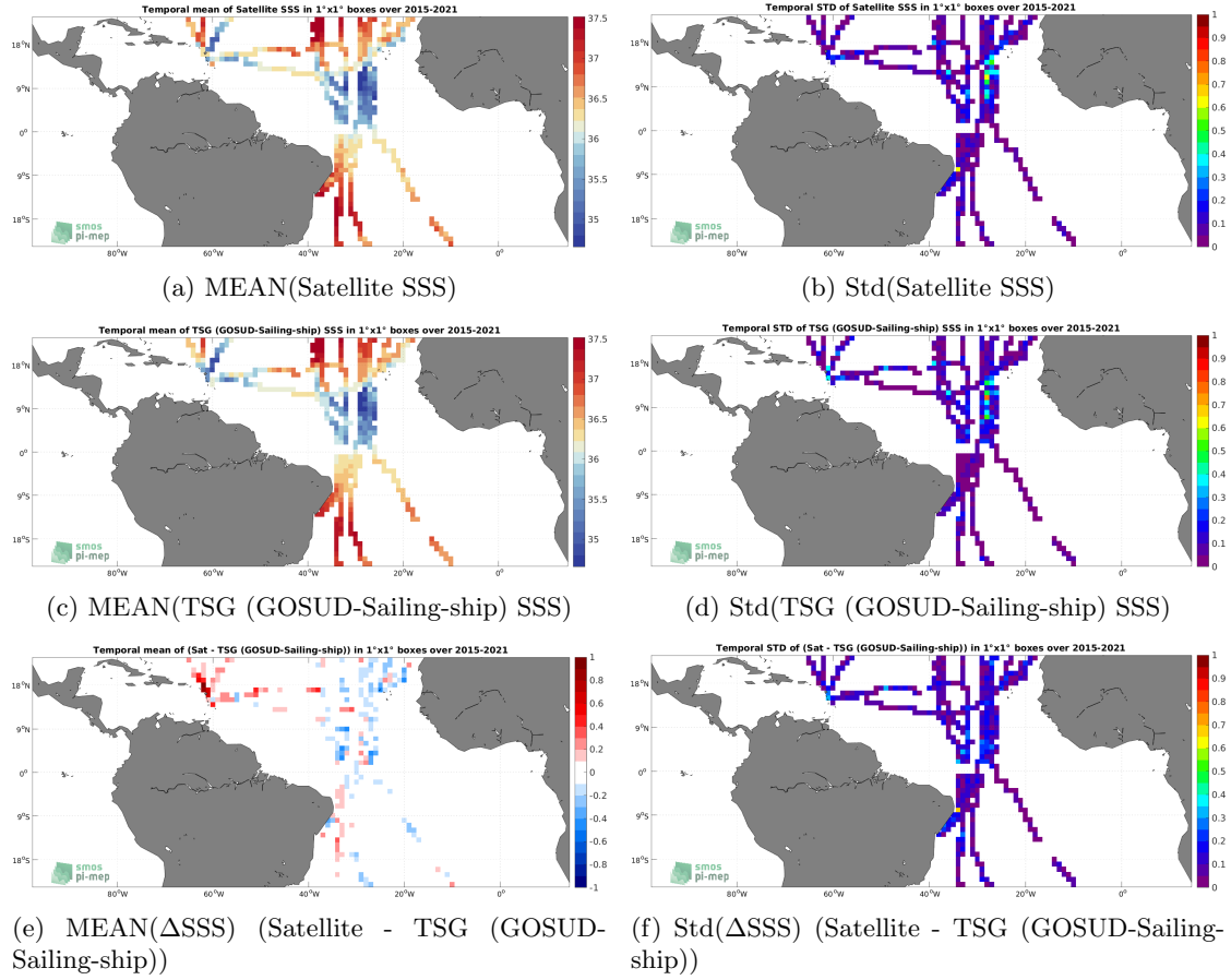
Figure 6: Temporal mean (left) and Std (right) of SSS from SMAP SSS L3 v5 - 8-Day running (RSS) (top), TSG (GOSUD-Sailing-ship) (middle), and of \Delta SSS (Satellite - TSG (GOSUD-Sailing-ship)). Only match-up pairs are used to generate these maps.
