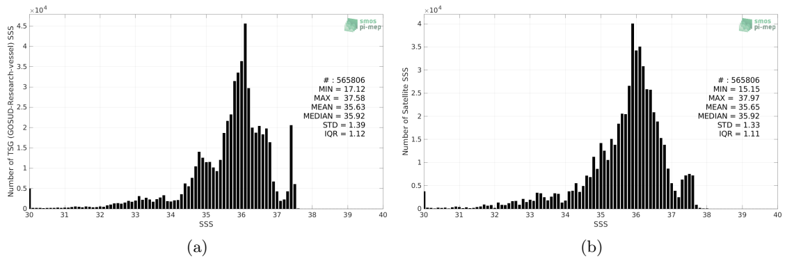
Figure 2: Histograms of SSS from TSG (GOSUD-Research-vessel) (a) and SMAP SSS L3 v5 - 8-Day running (RSS) (b) considering all match-up pairs per bins of 0.1 over the Tropical Atlantic Ocean Pi-MEP region and for the full satellite product period.
