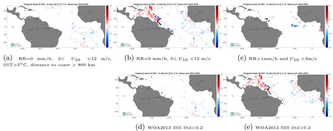
Figure 12: Temporal mean gridded over spatial boxes of size 1^\circ \times 1^\circ of \Delta SSS (SMAP SSS L3 v5 - 8-Day running (RSS) - TSG (GOSUD-Research-vessel)) for 5 different subdatasets corresponding to: RR=0 mm/h, 3 < U_{10} < 12 m/s, SST>5°C, distance to coast > 800 km (a), RR=0 mm/h, 3 < U_{10} < 12 m/s (b), RR>1mm/h and U_{10} < 4 m/s (c), WOA2013 SSS Std<0.2 (d), WOA2013 SSS Std>0.2 (e).
