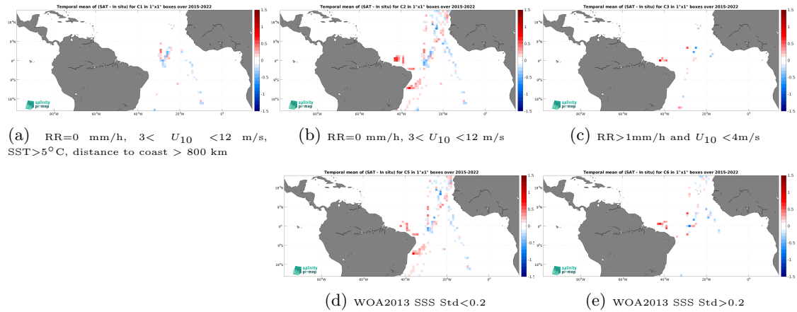
Figure 12: Temporal mean gridded over spatial boxes of size 1^\circ \times 1^\circ of \Delta\text{SSS} (SMAP SSS L3 v5 - 8-Day running (RSS) - TSG (CSIC-UTM)) for 5 different subdatasets corresponding to:RR=0 mm/h, 3 < U_{10} < 12 m/s, SST >5^\circ\text{C} , distance to coast > 800 km (a), RR=0 mm/h, 3 < U_{10} < 12 m/s (b), RR >1 mm/h and U_{10} < 4 m/s (c), WOA2013 SSS Std <0.2 (d), WOA2013 SSS Std >0.2 (e).
