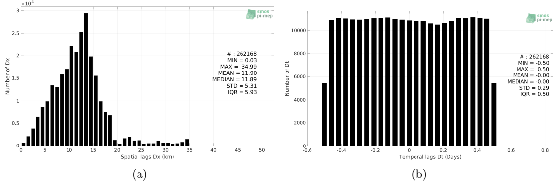
Figure 5: Histograms of the spatial (a) and temporal (b) lags between the location/time of the TSG (CSIC-UTM) measurement and the date of the corresponding SMAP SSS L3 v5 - 8-Day running (RSS) SSS pixel.
