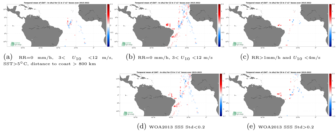
Figure 12: Temporal mean gridded over spatial boxes of size 1^\circ \times 1^\circ of \Delta SSS (SMAP SSS L3 v5 - 8-Day running (RSS) - TSG (CSIC-UTM)) for 5 different subdatasets corresponding to:RR=0 mm/h, 3 < U_{10} < 12 m/s, SST >5^\circ\text{C} , distance to coast > 800 km (a), RR=0 mm/h, 3 < U_{10} < 12 m/s (b), RR >1 mm/h and U_{10} < 4 m/s (c), WOA2013 SSS Std <0.2 (d), WOA2013 SSS Std >0.2 (e).
