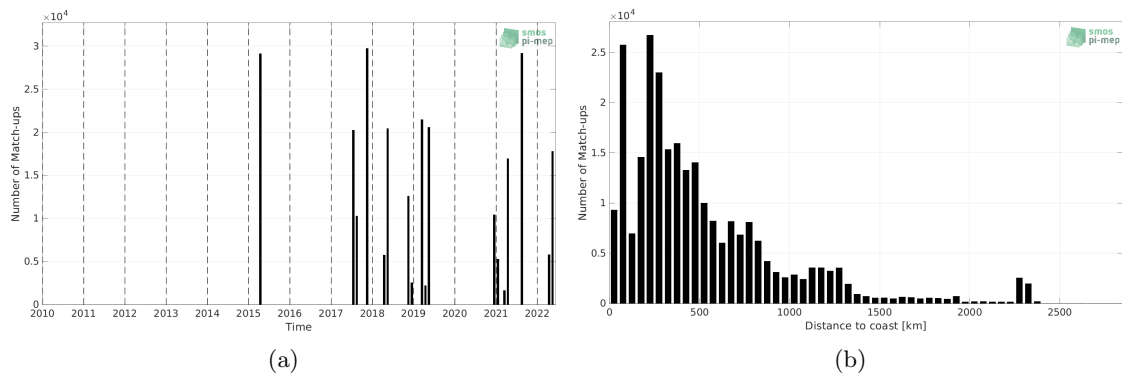
Figure 1: Number of match-ups between TSG (CSIC-UTM) and SMAP SSS L3 v5 - 8-Day running (RSS) SSS as a function of time (a) and as function of the distance to coast (b) over the Tropical Atlantic Ocean Pi-MEP region and for the full satellite product period.
