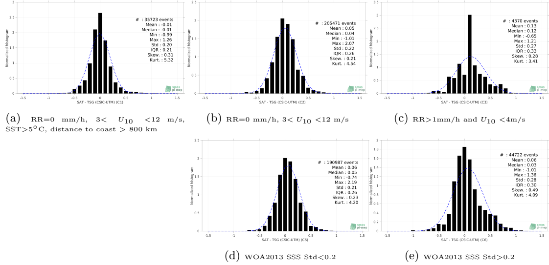
Figure 13: Normalized histogram of \Delta SSS (SMAP SSS L3 v5 - 8-Day running (RSS) - TSG (CSIC-UTM)) for 5 different subdatasets corresponding to: RR=0 mm/h, 3 < U_{10} < 12 m/s, SST > 5°C, distance to coast > 800 km (a), RR=0 mm/h, 3 < U_{10} < 12 m/s (b), RR > 1mm/h and U_{10} < 4 m/s (c), WOA2013 SSS Std < 0.2 (d), WOA2013 SSS Std > 0.2 (e).
