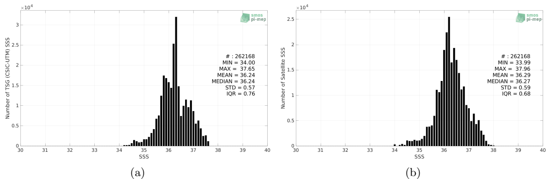
Figure 2: Histograms of SSS from TSG (CSIC-UTM) (a) and SMAP SSS L3 v5 - 8-Day running (RSS) (b) considering all match-up pairs per bins of 0.1 over the Tropical Atlantic Ocean Pi-MEP region and for the full satellite product period.
