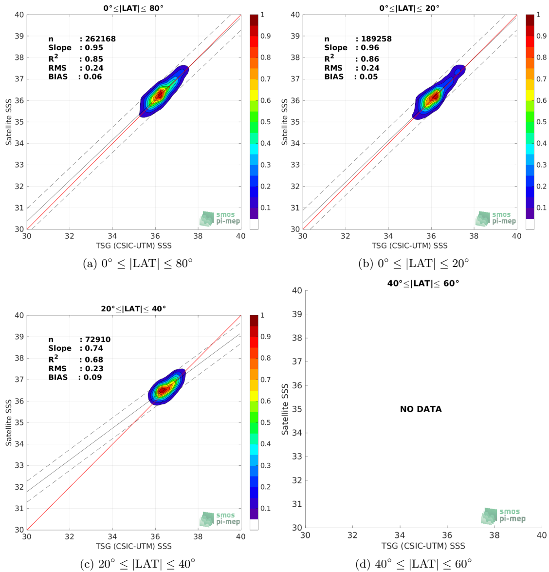
Figure 9: Contour maps of the concentration of SMAP SSS L3 v5 - 8-Day running (RSS) SSS (y-axis) versus TSG (CSIC-UTM) SSS (x-axis) at match-up pairs for different latitude bands. For each plot, the red line shows x=y . The black thin and dashed lines indicate a linear fit through the data cloud and the \pm 95\% confidence levels, respectively. The number match-up pairs n , the slope and R^2 coefficient of the linear fit, the root mean square (RMS) and the mean bias between satellite and in situ data are indicated for each latitude band in each plots.
