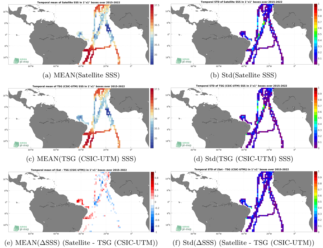
Figure 6: Temporal mean (left) and Std (right) of SSS from SMAP SSS L3 v5 - 8-Day running (RSS) (top), TSG (CSIC-UTM) (middle), and of \Delta SSS (Satellite - TSG (CSIC-UTM)). Only match-up pairs are used to generate these maps.
