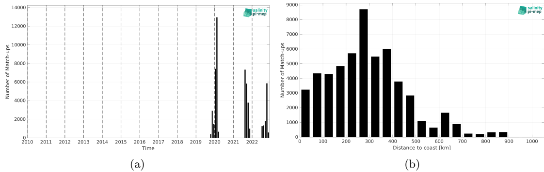
Figure 1: Number of match-ups between Saildrone and SMAP SSS L3 v5 - 8-Day running (RSS) SSS as a function of time (a) and as function of the distance to coast (b) over the Tropical Atlantic Ocean Pi-MEP region and for the full satellite product period.
