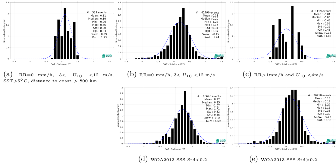
Figure 13: Normalized histogram of \Delta\text{SSS} (SMAP SSS L3 v5 - 8-Day running (RSS) - Saldrone) for 5 different subdatasets corresponding to: RR=0 mm/h, 3 < U_{10} < 12 m/s, SST>5°C, distance to coast > 800 km (a), RR=0 mm/h, 3 < U_{10} < 12 m/s (b), RR>1mm/h and U_{10} < 4 m/s (c), WOA2013 SSS Std<0.2 (d), WOA2013 SSS Std>0.2 (e).
