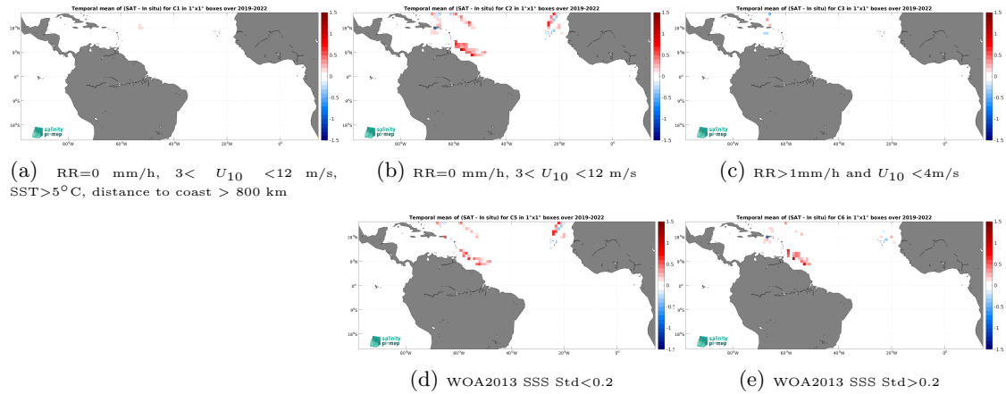
Figure 12: Temporal mean gridded over spatial boxes of size 1^\circ \times 1^\circ of \Delta\text{SSS} (SMAP SSS L3 v5 - 8-Day running (RSS) - Sairdrone) for 5 different subdatasets corresponding to:RR=0 mm/h, 3 < U_{10} < 12 m/s, SST >5^\circ\text{C} , distance to coast > 800 km (a), RR=0 mm/h, 3 < U_{10} < 12 m/s (b), RR >1 mm/h and U_{10} < 4 m/s (c), WOA2013 SSS Std <0.2 (d), WOA2013 SSS Std >0.2 (e).
