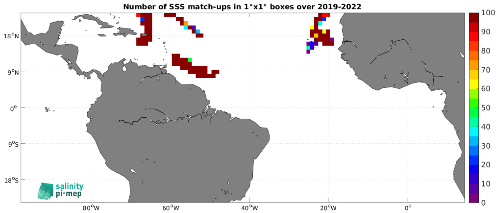
Figure 4: Number of SSS match-ups between Saildrone SSS and the SMAP SSS L3 v5 - 8-Day running (RSS) SSS product for the Tropical Atlantic Ocean Pi-MEP region over 1^\circ \times 1^\circ boxes and for the full satellite product period.
