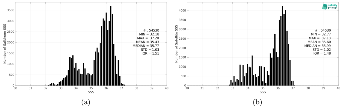
Figure 2: Histograms of SSS from Saildrone (a) and SMAP SSS L3 v5 - 8-Day running (RSS) (b) considering all match-up pairs per bins of 0.1 over the Tropical Atlantic Ocean Pi-MEP region and for the full satellite product period.
