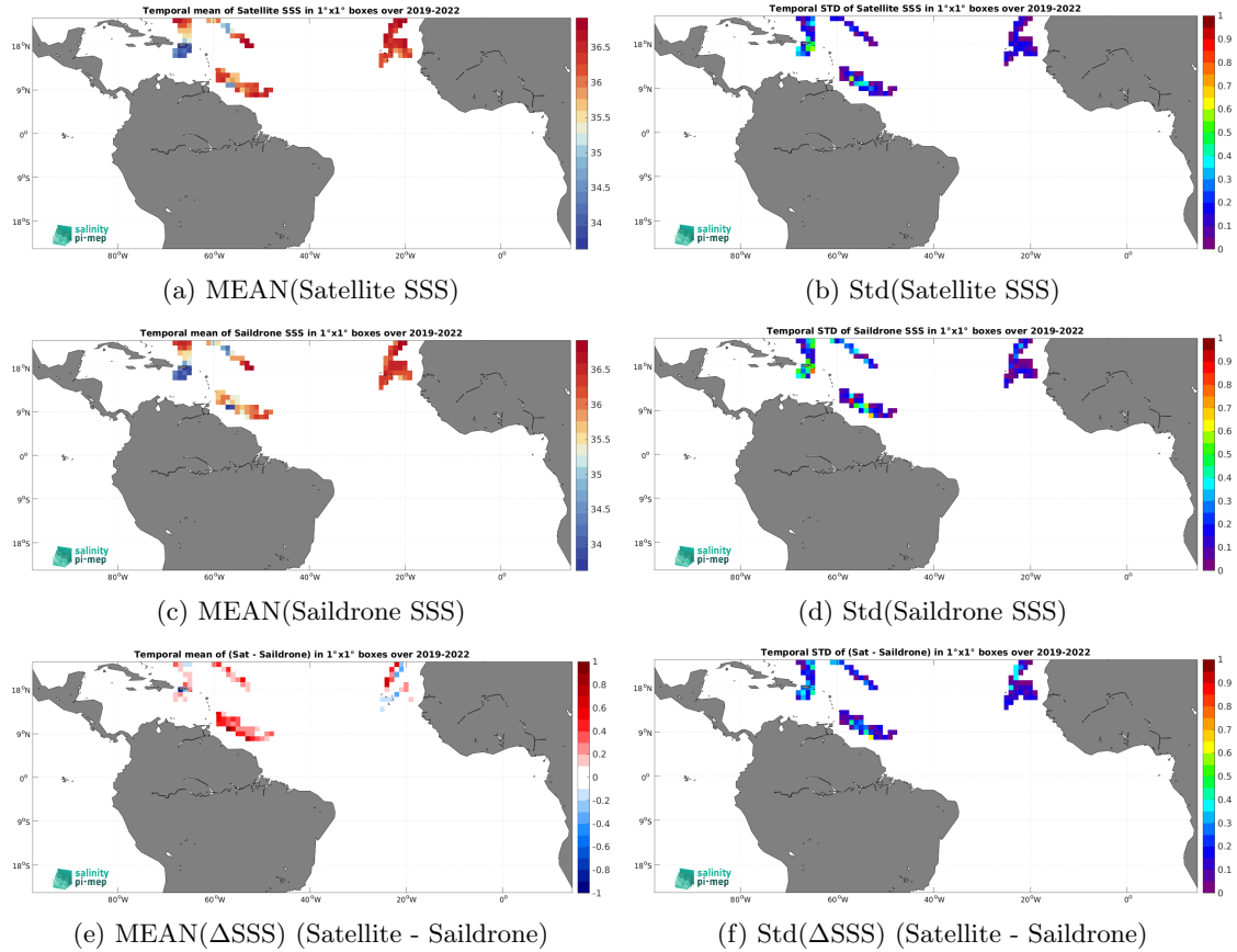
Figure 6: Temporal mean (left) and Std (right) of SSS from SMAP SSS L3 v5 - 8-Day running (RSS) (top), Saildrone (middle), and of \Delta\text{SSS} (Satellite - Saildrone). Only match-up pairs are used to generate these maps.
