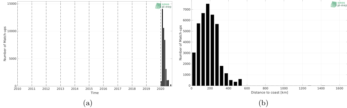
Figure 1: Number of match-ups between Surface drifters and SMAP SSS L3 v5 - 8-Day running (RSS) SSS as a function of time (a) and as function of the distance to coast (b) over the Tropical Atlantic Ocean Pi-MEP region and for the full satellite product period.
