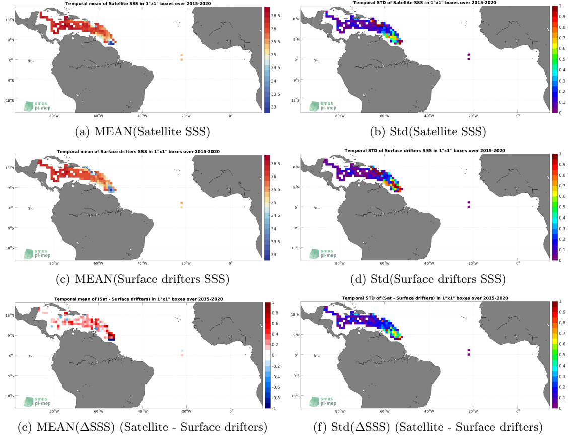
Figure 5: Temporal mean (left) and Std (right) of SSS from SMAP SSS L3 v5 - 8-Day running (RSS) (top), Surface drifters (middle), and of \Delta SSS (Satellite - Surface drifters). Only match-up pairs are used to generate these maps.
