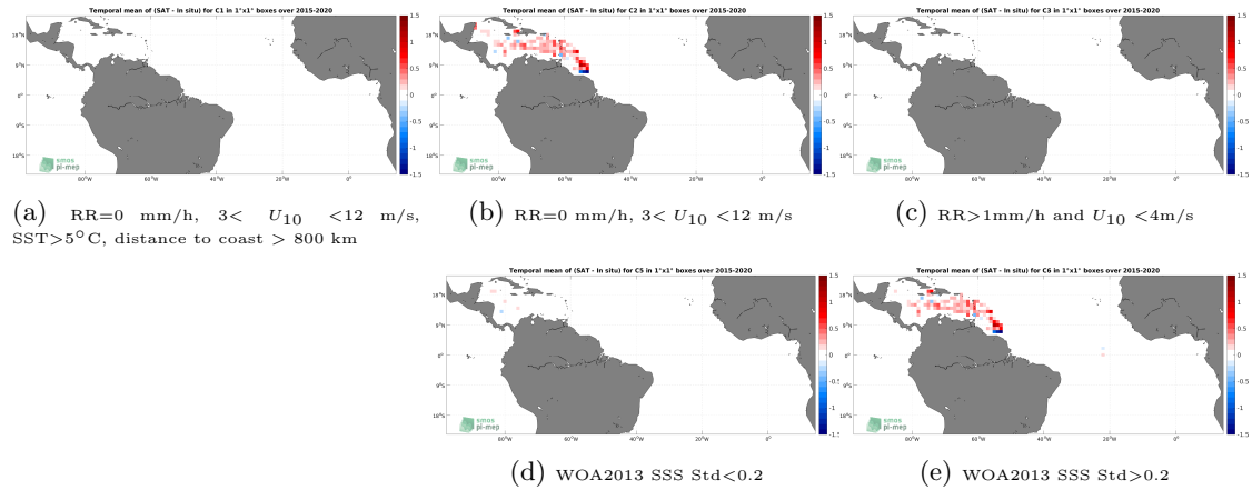
Figure 11: Temporal mean gridded over spatial boxes of size 1^\circ \times 1^\circ of \Delta SSS (SMAP SSS L3 v5 - 8-Day running (RSS) - Surface drifters) for 5 different subdatasets corresponding to:RR=0 mm/h, 3 < U_{10} < 12 m/s, SST >5^\circ\text{C} , distance to coast > 800 km (a), RR=0 mm/h, 3 < U_{10} < 12 m/s (b), RR >1 mm/h and U_{10} < 4 m/s (c), WOA2013 SSS Std <0.2 (d), WOA2013 SSS Std >0.2 (e).
