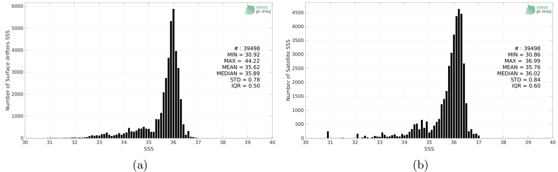
Figure 2: Histograms of SSS from Surface drifters (a) and SMAP SSS L3 v5 - 8-Day running (RSS) (b) considering all match-up pairs per bins of 0.1 over the Tropical Atlantic Ocean Pi-MEP region and for the full satellite product period.
