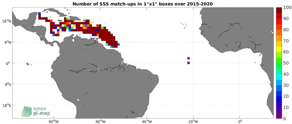
Figure 3: Number of SSS match-ups between Surface drifters SSS and the SMAP SSS L3 v5 - 8-Day running (RSS) SSS product for the Tropical Atlantic Ocean Pi-MEP region over 1^\circ \times 1^\circ boxes and for the full satellite product period.
