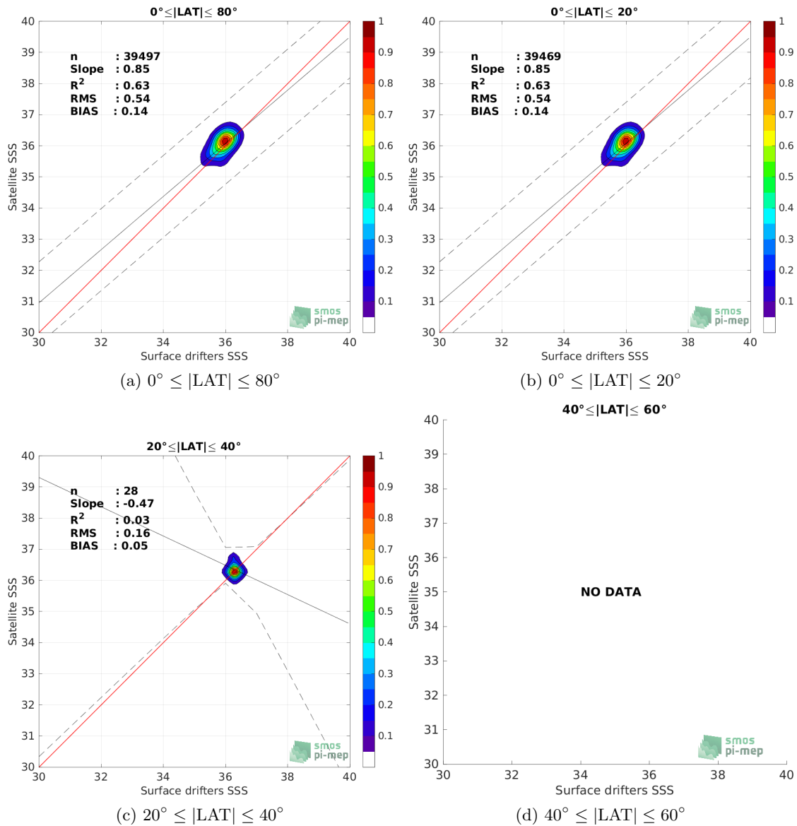
Figure 8: Contour maps of the concentration of SMAP SSS L3 v5 - 8-Day running (RSS) SSS (y-axis) versus Surface drifters SSS (x-axis) at match-up pairs for different latitude bands. For each plot, the red line shows x=y . The black thin and dashed lines indicate a linear fit through the data cloud and the \pm 95\% confidence levels, respectively. The number match-up pairs n , the slope and R^2 coefficient of the linear fit, the root mean square (RMS) and the mean bias between satellite and in situ data are indicated for each latitude band in each plots.
