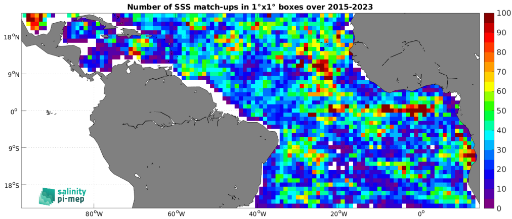
Figure 4: Number of SSS match-ups between Argo SSS and the SMAP SSS L3 v5 - 8-Day running (RSS) SSS product for the Tropical Atlantic Ocean Pi-MEP region over 1^\circ \times 1^\circ boxes and for the full satellite product period.
