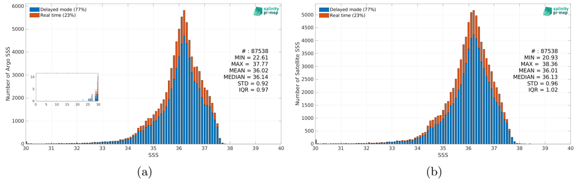
Figure 2: Histograms of SSS from Argo (a) and SMAP SSS L3 v5 - 8-Day running (RSS) (b) considering all match-up pairs per bins of 0.1 over the Tropical Atlantic Ocean Pi-MEP region and for the full satellite product period.
