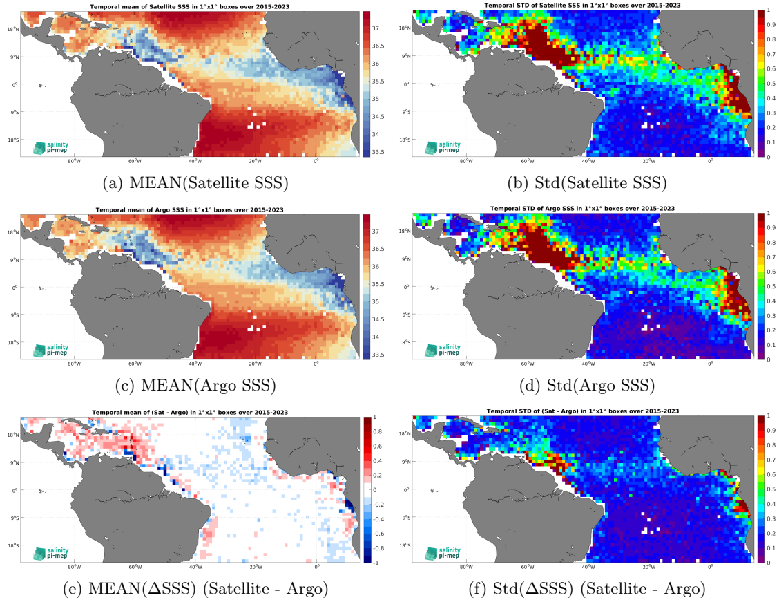
Figure 6: Temporal mean (left) and Std (right) of SSS from SMAP SSS L3 v5 - 8-Day running (RSS) (top), Argo (middle), and of \Delta\text{SSS}(\text{Satellite} - \text{Argo}) . Only match-up pairs are used to generate these maps.
