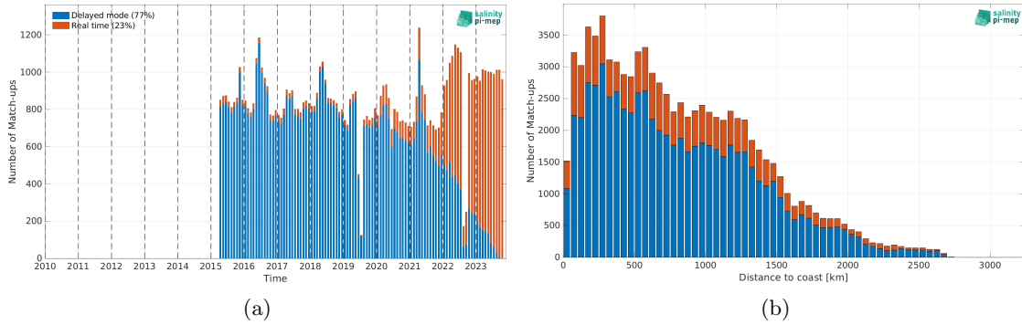
Figure 1: Number of match-ups between Argo and SMAP SSS L3 v5 - 8-Day running (RSS) SSS as a function of time (a) and as function of the distance to coast (b) over the Tropical Atlantic Ocean Pi-MEP region and for the full satellite product period.
