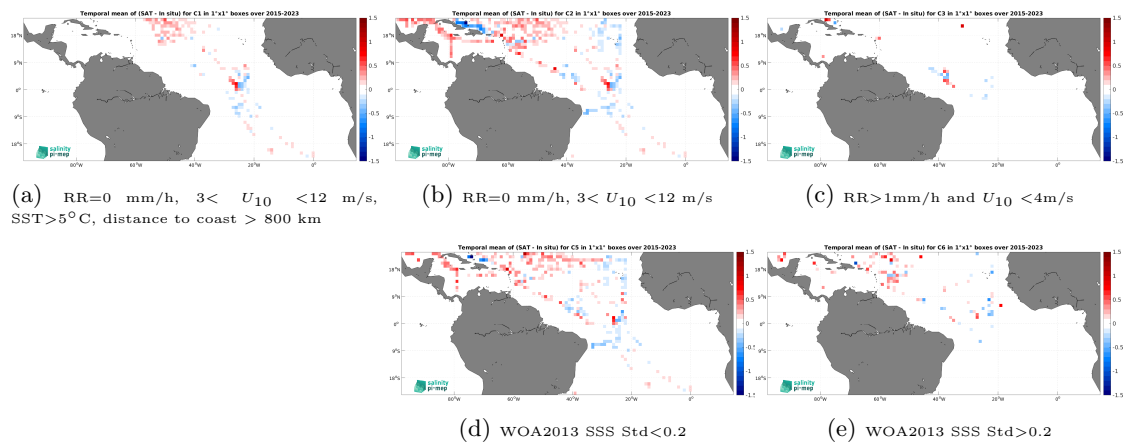
Figure 12: Temporal mean gridded over spatial boxes of size 1^\circ \times 1^\circ of \Delta\text{SSS} (SMAP SSS L3 v5 - Monthly (RSS) - TSG (SAMOS)) for 5 different subdatasets corresponding to:RR=0 mm/h, 3 < U_{10} < 12 m/s, SST >5^\circ\text{C} , distance to coast > 800 km (a), RR=0 mm/h, 3 < U_{10} < 12 m/s (b), RR >1 mm/h and U_{10} < 4 m/s (c), WOA2013 SSS Std <0.2 (d), WOA2013 SSS Std >0.2 (e).
