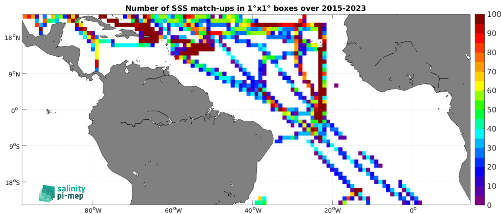
Figure 4: Number of SSS match-ups between TSG (SAMOS) SSS and the SMAP SSS L3 v5 - Monthly (RSS) SSS product for the Tropical Atlantic Ocean Pi-MEP region over 1^\circ \times 1^\circ boxes and for the full satellite product period.
