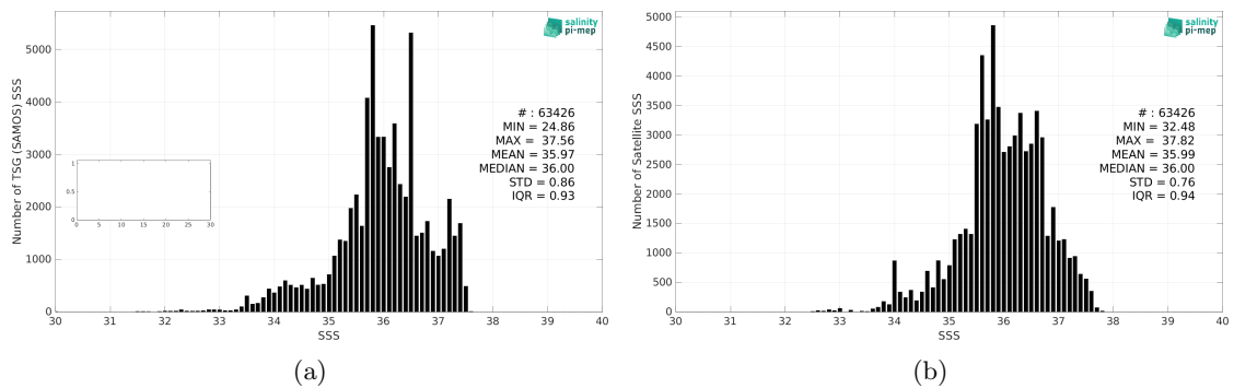
Figure 2: Histograms of SSS from TSG (SAMOS) (a) and SMAP SSS L3 v5 - Monthly (RSS) (b) considering all match-up pairs per bins of 0.1 over the Tropical Atlantic Ocean Pi-MEP region and for the full satellite product period.
