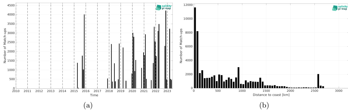
Figure 1: Number of match-ups between TSG (SAMOS) and SMAP SSS L3 v5 - Monthly (RSS) SSS as a function of time (a) and as function of the distance to coast (b) over the Tropical Atlantic Ocean Pi-MEP region and for the full satellite product period.
