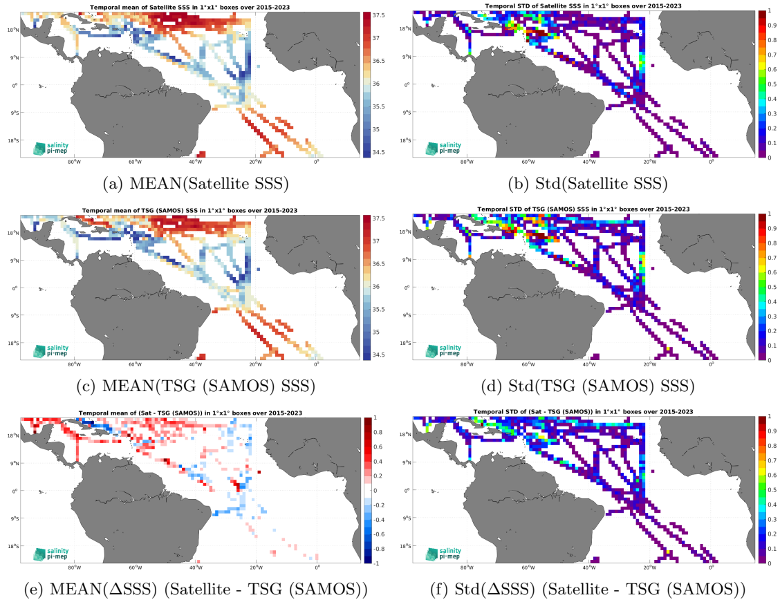
Figure 6: Temporal mean (left) and Std (right) of SSS from SMAP SSS L3 v5 - Monthly (RSS) (top), TSG (SAMOS) (middle), and of \Delta SSS (Satellite - TSG (SAMOS)). Only match-up pairs are used to generate these maps.
