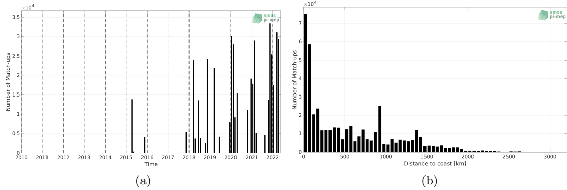
Figure 1: Number of match-ups between TSG (SAMOS) and SMAP SSS L3 v5 - Monthly (RSS) SSS as a function of time (a) and as function of the distance to coast (b) over the Tropical Atlantic Ocean Pi-MEP region and for the full satellite product period.
