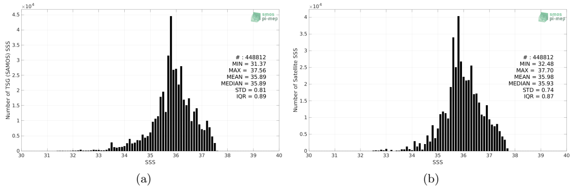
Figure 2: Histograms of SSS from TSG (SAMOS) (a) and SMAP SSS L3 v5 - Monthly (RSS) (b) considering all match-up pairs per bins of 0.1 over the Tropical Atlantic Ocean Pi-MEP region and for the full satellite product period.
