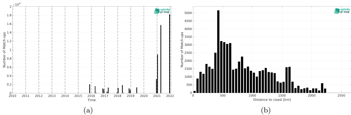
Figure 1: Number of match-ups between TSG (Polarstern) and SMAP SSS L3 v5 - Monthly (RSS) SSS as a function of time (a) and as function of the distance to coast (b) over the Tropical Atlantic Ocean Pi-MEP region and for the full satellite product period.
