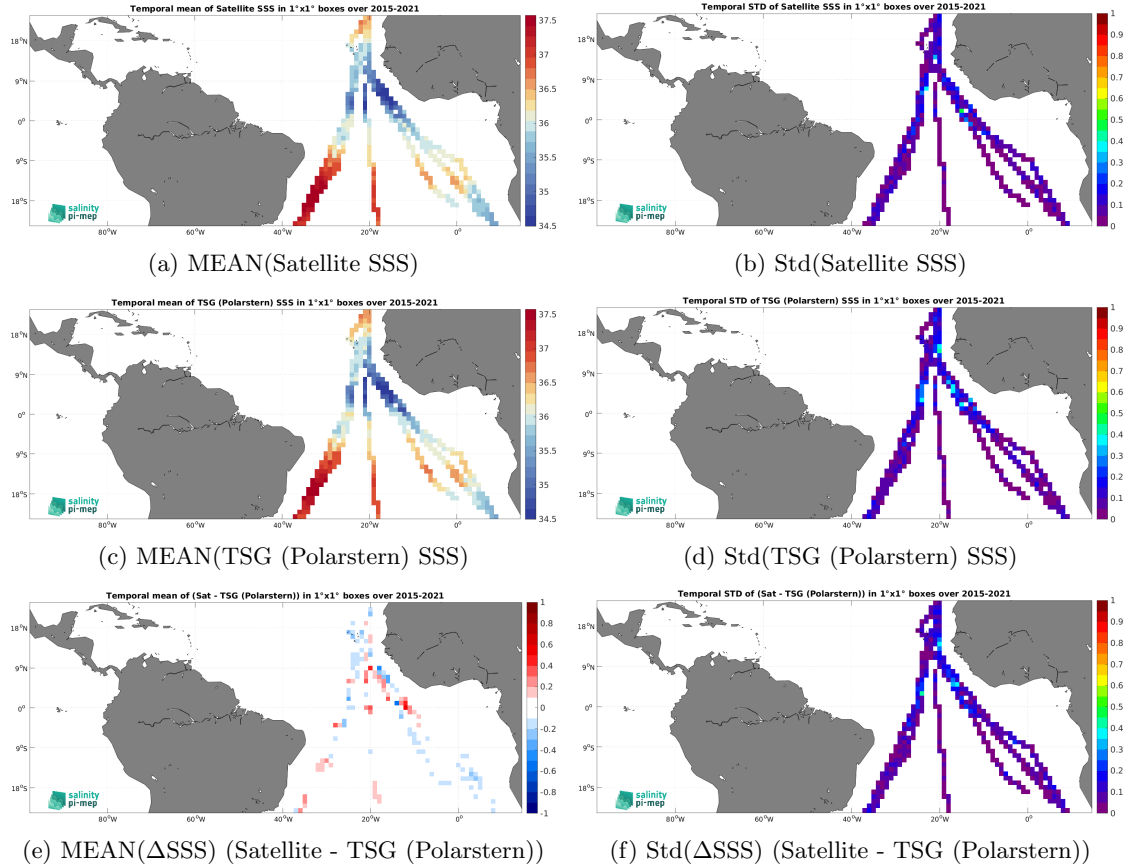
Figure 6: Temporal mean (left) and Std (right) of SSS from SMAP SSS L3 v5 - Monthly (RSS) (top), TSG (Polarstern) (middle), and of \Delta\text{SSS} (Satellite - TSG (Polarstern)). Only match-up pairs are used to generate these maps.
