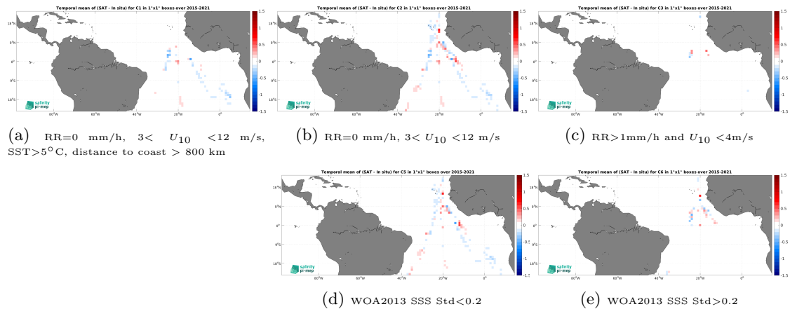
Figure 12: Temporal mean gridded over spatial boxes of size 1^\circ \times 1^\circ of \Delta\text{SSS} (SMAP SSS L3 v5 - Monthly (RSS) - TSG (Polarstern)) for 5 different subdatasets corresponding to:RR=0 mm/h, 3 < U_{10} < 12 m/s, SST >5^\circ\text{C} , distance to coast > 800 km (a), RR=0 mm/h, 3 < U_{10} < 12 m/s (b), RR >1 mm/h and U_{10} < 4 m/s (c), WOA2013 SSS Std <0.2 (d), WOA2013 SSS Std >0.2 (e).
