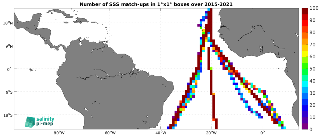
Figure 4: Number of SSS match-ups between TSG (Polarstern) SSS and the SMAP SSS L3 v5 - Monthly (RSS) SSS product for the Tropical Atlantic Ocean Pi-MEP region over 1^\circ \times 1^\circ boxes and for the full satellite product period.
