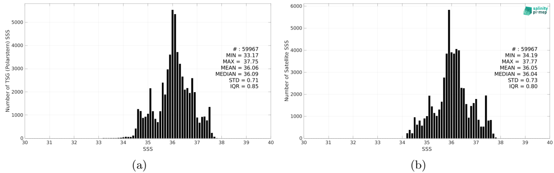
Figure 2: Histograms of SSS from TSG (Polarstern) (a) and SMAP SSS L3 v5 - Monthly (RSS) (b) considering all match-up pairs per bins of 0.1 over the Tropical Atlantic Ocean Pi-MEP region and for the full satellite product period.
