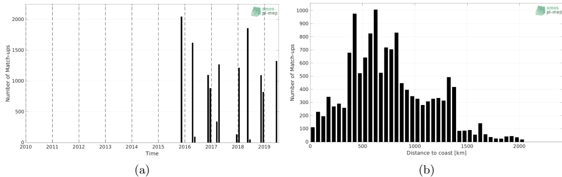
Figure 1: Number of match-ups between TSG (Polarstern) and SMAP SSS L3 v5 - Monthly (RSS) SSS as a function of time (a) and as function of the distance to coast (b) over the Tropical Atlantic Ocean Pi-MEP region and for the full satellite product period.
