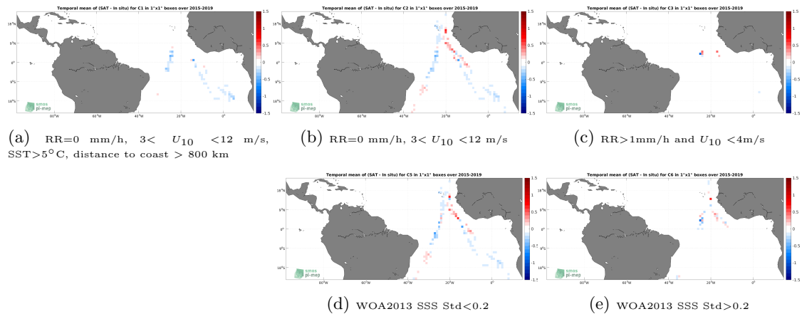
Figure 12: Temporal mean gridded over spatial boxes of size 1^\circ \times 1^\circ of \Delta SSS (SMAP SSS L3 v5 - Monthly (RSS) - TSG (Polarstern)) for 5 different subdatasets corresponding to:RR=0 mm/h, 3 < U_{10} < 12 m/s, SST >5^\circ\text{C} , distance to coast > 800 km (a), RR=0 mm/h, 3 < U_{10} < 12 m/s (b), RR >1 mm/h and U_{10} < 4 m/s (c), WOA2013 SSS Std <0.2 (d), WOA2013 SSS Std >0.2 (e).
