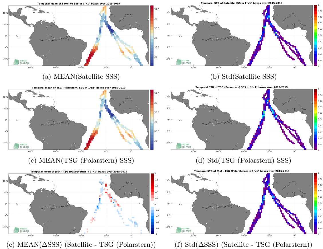
Figure 6: Temporal mean (left) and Std (right) of SSS from SMAP SSS L3 v5 - Monthly (RSS) (top), TSG (Polarstern) (middle), and of \Delta SSS (Satellite - TSG (Polarstern)). Only match-up pairs are used to generate these maps.
