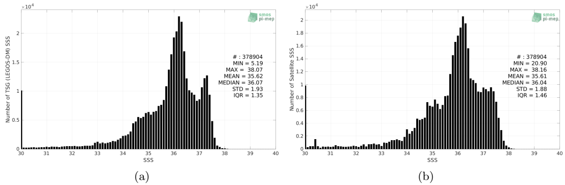
Figure 2: Histograms of SSS from TSG (LEGOS-DM) (a) and SMAP SSS L3 v5 - Monthly (RSS) (b) considering all match-up pairs per bins of 0.1 over the Tropical Atlantic Ocean Pi-MEP region and for the full satellite product period.
