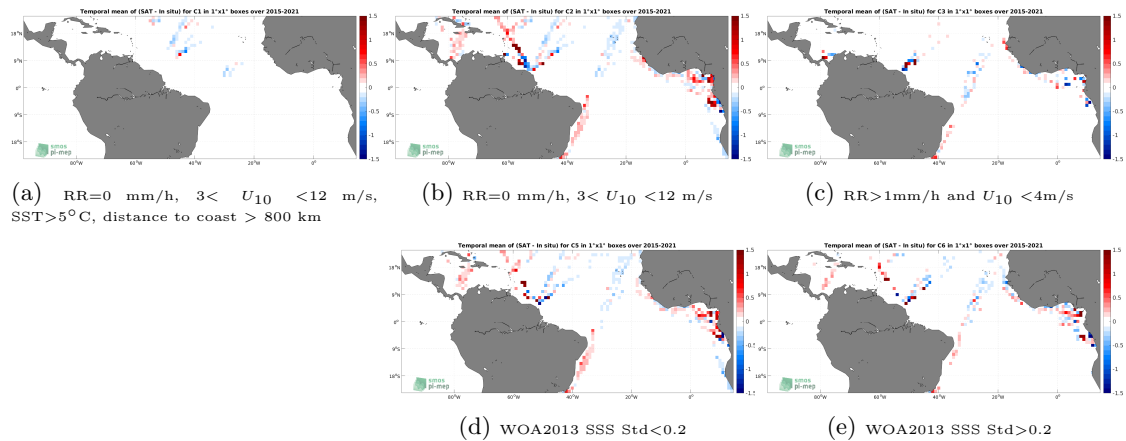
Figure 12: Temporal mean gridded over spatial boxes of size 1^\circ \times 1^\circ of \Delta\text{SSS} (SMAP SSS L3 v5 - Monthly (RSS) - TSG (LEGOS-DM)) for 5 different subdatasets corresponding to:RR=0 mm/h, 3 < U_{10} < 12 m/s, SST >5^\circ\text{C} , distance to coast > 800 km (a), RR=0 mm/h, 3 < U_{10} < 12 m/s (b), RR >1 mm/h and U_{10} < 4 m/s (c), WOA2013 SSS Std <0.2 (d), WOA2013 SSS Std >0.2 (e).
