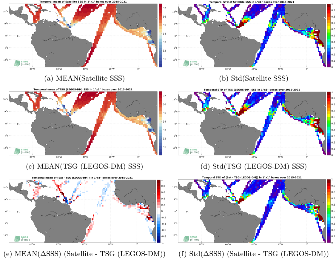
Figure 6: Temporal mean (left) and Std (right) of SSS from SMAP SSS L3 v5 - Monthly (RSS) (top), TSG (LEGOS-DM) (middle), and of \Delta\text{SSS} (Satellite - TSG (LEGOS-DM)). Only match-up pairs are used to generate these maps.
