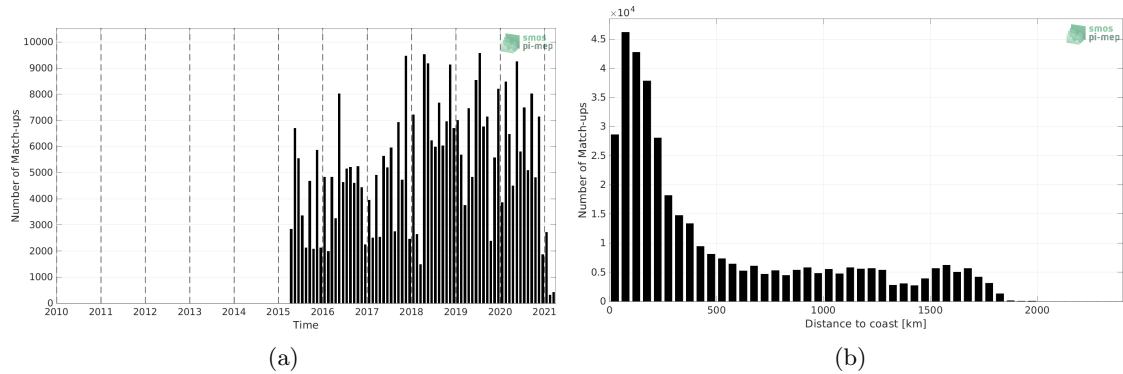
Figure 1: Number of match-ups between TSG (LEGOS-DM) and SMAP SSS L3 v5 - Monthly (RSS) SSS as a function of time (a) and as function of the distance to coast (b) over the Tropical Atlantic Ocean Pi-MEP region and for the full satellite product period.
