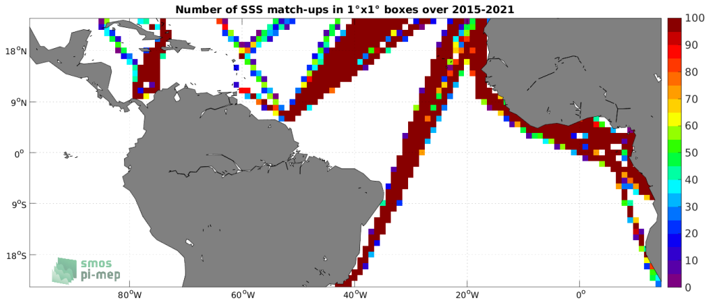
Figure 4: Number of SSS match-ups between TSG (LEGOS-DM) SSS and the SMAP SSS L3 v5 - Monthly (RSS) SSS product for the Tropical Atlantic Ocean Pi-MEP region over 1^\circ \times 1^\circ boxes and for the full satellite product period.
