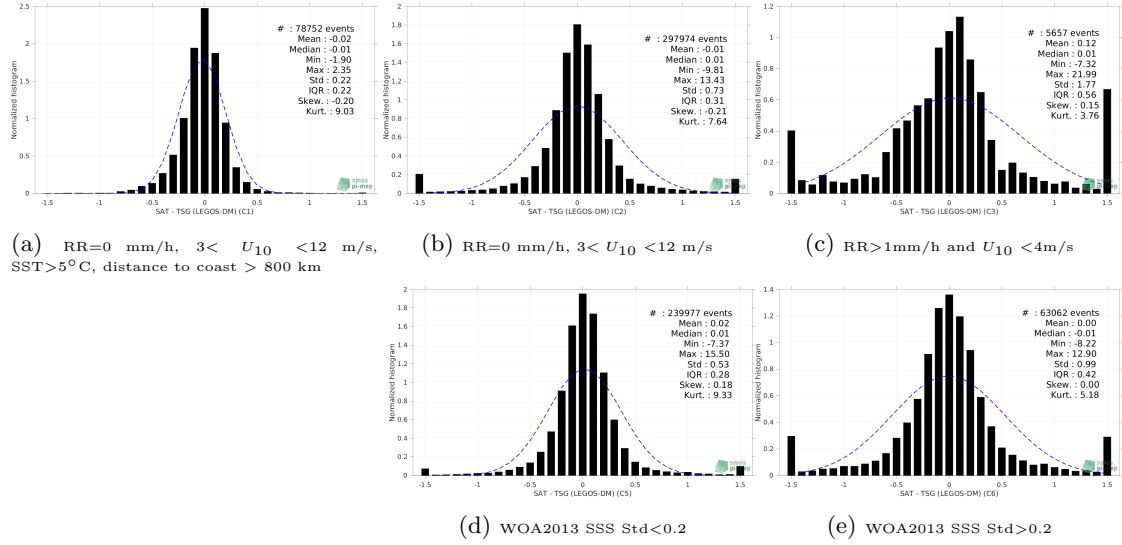
Figure 13: Normalized histogram of \Delta SSS (SMAP SSS L3 v5 - Monthly (RSS) - TSG (LEGOS-DM)) for 5 different subdatasets corresponding to: RR=0 mm/h, 3 < U_{10} < 12 m/s, SST>5°C, distance to coast > 800 km (a), RR=0 mm/h, 3 < U_{10} < 12 m/s (b), RR>1mm/h and U_{10} < 4 m/s (c), WOA2013 SSS Std<0.2 (d), WOA2013 SSS Std>0.2 (e).
