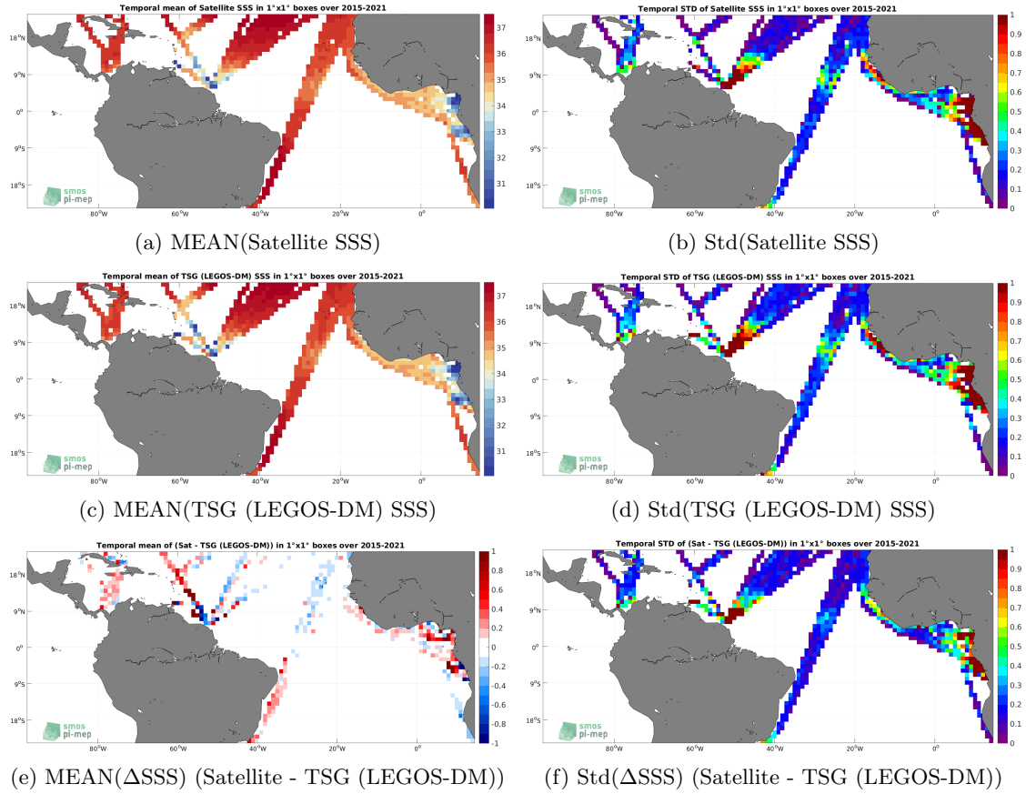
Figure 6: Temporal mean (left) and Std (right) of SSS from SMAP SSS L3 v5 - Monthly (RSS) (top), TSG (LEGOS-DM) (middle), and of \Delta SSS (Satellite - TSG (LEGOS-DM)). Only match-up pairs are used to generate these maps.
