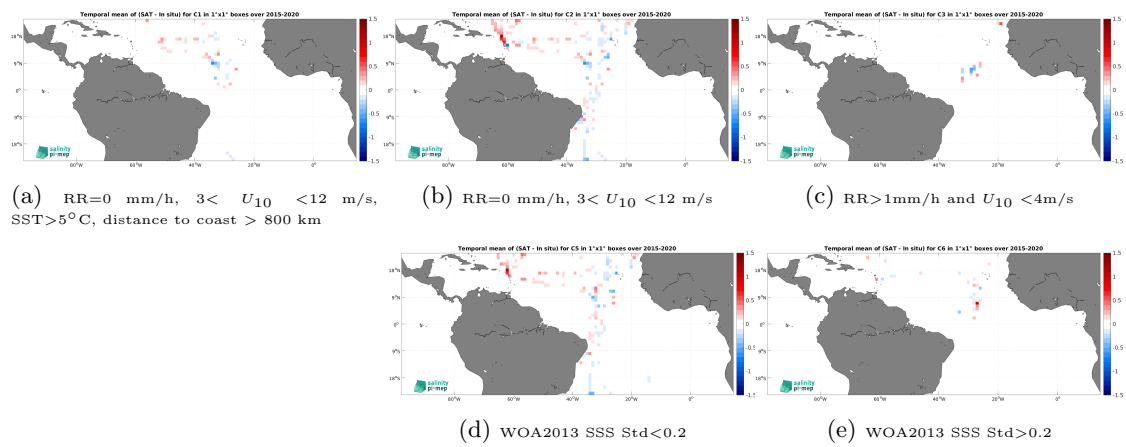
Figure 12: Temporal mean gridded over spatial boxes of size 1^\circ \times 1^\circ of \Delta\text{SSS} (SMAP SSS L3 v5 - Monthly (RSS) - TSG (GOSUD-Sailing-ship)) for 5 different subdatasets corresponding to:RR=0 mm/h, 3 < U_{10} < 12 m/s, SST >5^\circ\text{C} , distance to coast > 800 km (a), RR=0 mm/h, 3 < U_{10} < 12 m/s (b), RR >1 mm/h and U_{10} < 4 m/s (c), WOA2013 SSS Std <0.2 (d), WOA2013 SSS Std >0.2 (e).
