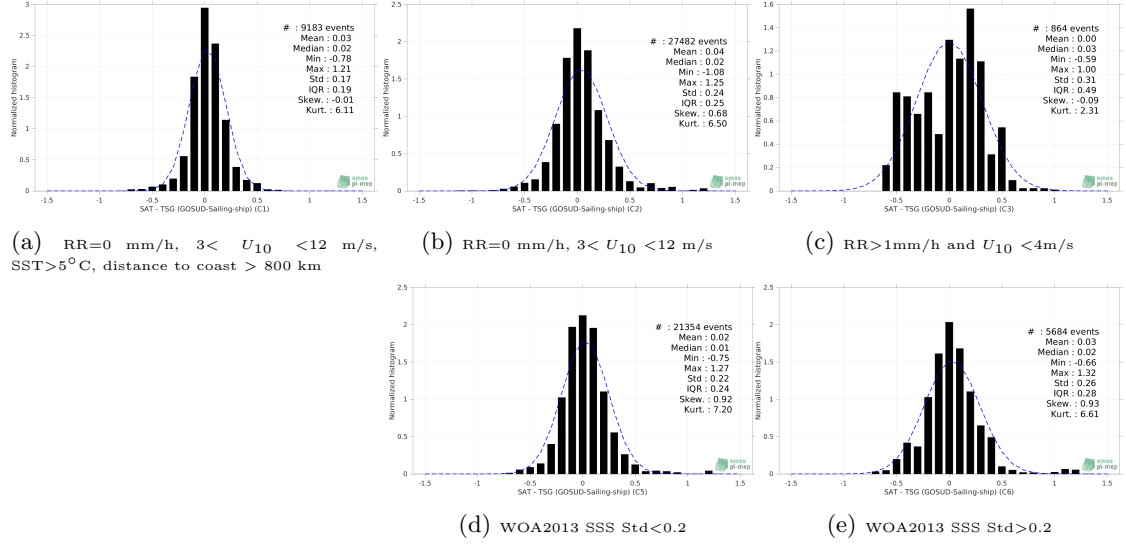
Figure 13: Normalized histogram of \Delta SSS (SMAP SSS L3 v5 - Monthly (RSS) - TSG (GOSUD-Sailing-ship)) for 5 different subdatasets corresponding to: RR=0 mm/h, 3 < U_{10} < 12 m/s, SST>5°C, distance to coast > 800 km (a), RR=0 mm/h, 3 < U_{10} < 12 m/s (b), RR>1mm/h and U_{10} < 4 m/s (c), WOA2013 SSS Std<0.2 (d), WOA2013 SSS Std>0.2 (e).
