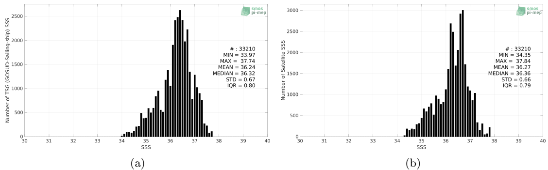
Figure 2: Histograms of SSS from TSG (GOSUD-Sailing-ship) (a) and SMAP SSS L3 v5 - Monthly (RSS) (b) considering all match-up pairs per bins of 0.1 over the Tropical Atlantic Ocean Pi-MEP region and for the full satellite product period.
