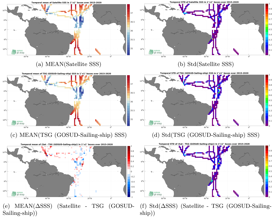
Figure 6: Temporal mean (left) and Std (right) of SSS from SMAP SSS L3 v5 - Monthly (RSS) (top), TSG (GOSUD-Sailing-ship) (middle), and of \Delta SSS (Satellite - TSG (GOSUD-Sailing-ship)). Only match-up pairs are used to generate these maps.
