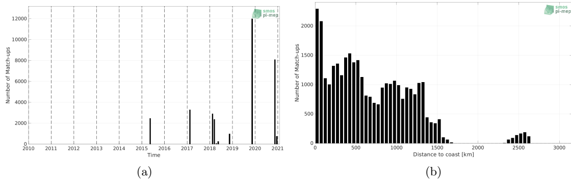
Figure 1: Number of match-ups between TSG (GOSUD-Sailing-ship) and SMAP SSS L3 v5 - Monthly (RSS) SSS as a function of time (a) and as function of the distance to coast (b) over the Tropical Atlantic Ocean Pi-MEP region and for the full satellite product period.
