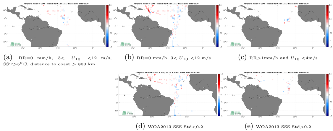
Figure 12: Temporal mean gridded over spatial boxes of size 1^\circ \times 1^\circ of \Delta\text{SSS} (SMAP SSS L3 v5 - Monthly (RSS) - TSG (GOSUD-Sailing-ship)) for 5 different subdatasets corresponding to:RR=0 mm/h, 3 < U_{10} < 12 m/s, SST >5^\circ\text{C} , distance to coast > 800 km (a), RR=0 mm/h, 3 < U_{10} < 12 m/s (b), RR >1 mm/h and U_{10} < 4 m/s (c), WOA2013 SSS Std <0.2 (d), WOA2013 SSS Std >0.2 (e).
