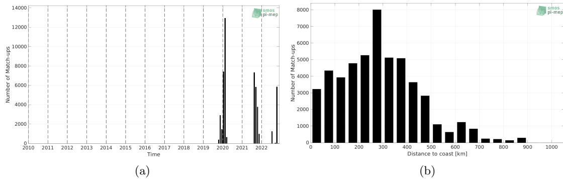
Figure 1: Number of match-ups between Saildrone and SMAP SSS L3 v5 - Monthly (RSS) SSS as a function of time (a) and as function of the distance to coast (b) over the Tropical Atlantic Ocean Pi-MEP region and for the full satellite product period.
