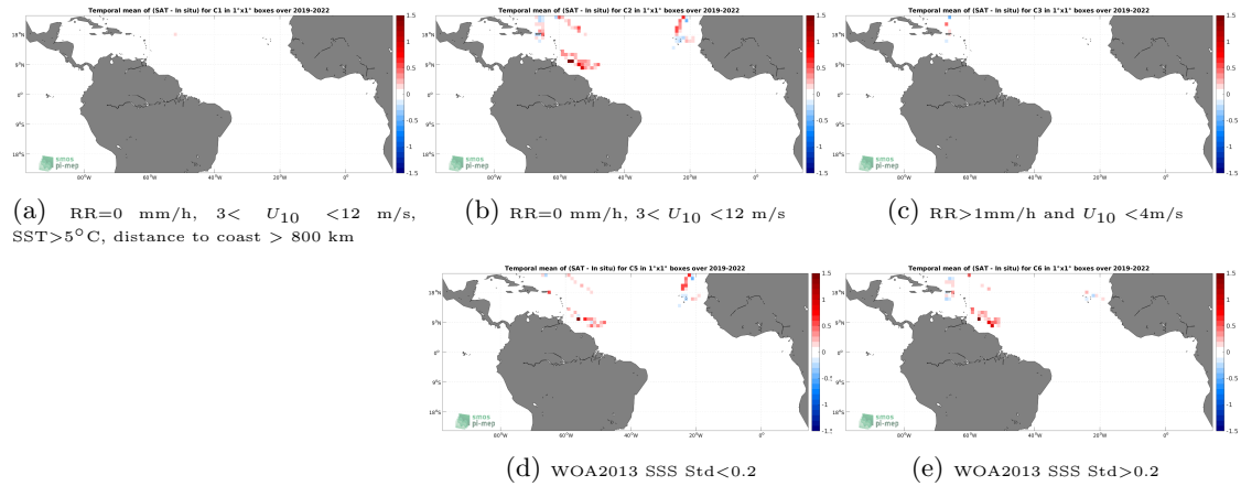
Figure 12: Temporal mean gridded over spatial boxes of size 1^\circ \times 1^\circ of \Delta SSS (SMAP SSS L3 v5 - Monthly (RSS) - Saildron) for 5 different subdatasets corresponding to:RR=0 mm/h, 3 < U_{10} < 12 m/s, SST >5^\circ\text{C} , distance to coast > 800 km (a), RR=0 mm/h, 3 < U_{10} < 12 m/s (b), RR >1 mm/h and U_{10} < 4 m/s (c), WOA2013 SSS Std <0.2 (d), WOA2013 SSS Std >0.2 (e).
