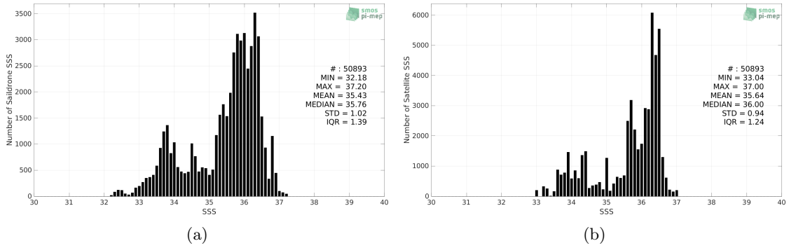
Figure 2: Histograms of SSS from Saildrone (a) and SMAP SSS L3 v5 - Monthly (RSS) (b) considering all match-up pairs per bins of 0.1 over the Tropical Atlantic Ocean Pi-MEP region and for the full satellite product period.
