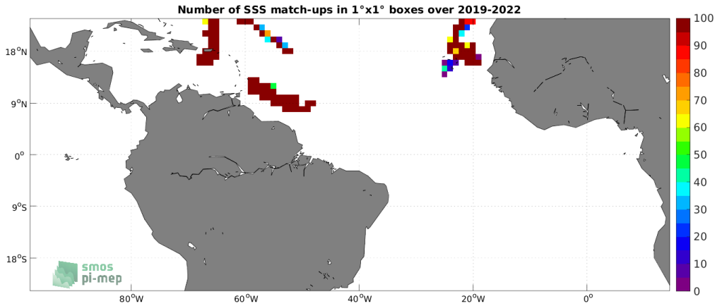
Figure 4: Number of SSS match-ups between Saildrone SSS and the SMAP SSS L3 v5 - Monthly (RSS) SSS product for the Tropical Atlantic Ocean Pi-MEP region over 1^\circ \times 1^\circ boxes and for the full satellite product period.
