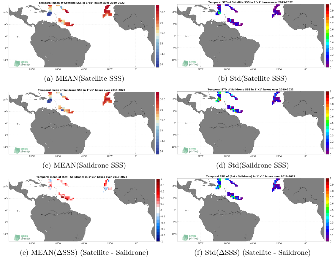
Figure 6: Temporal mean (left) and Std (right) of SSS from SMAP SSS L3 v5 - Monthly (RSS) (top), Sairdrone (middle), and of \Delta SSS (Satellite - Sairdrone). Only match-up pairs are used to generate these maps.
