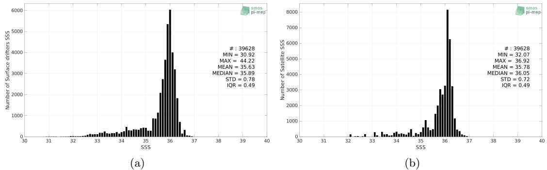
Figure 2: Histograms of SSS from Surface drifters (a) and SMAP SSS L3 v5 - Monthly (RSS) (b) considering all match-up pairs per bins of 0.1 over the Tropical Atlantic Ocean Pi-MEP region and for the full satellite product period.
