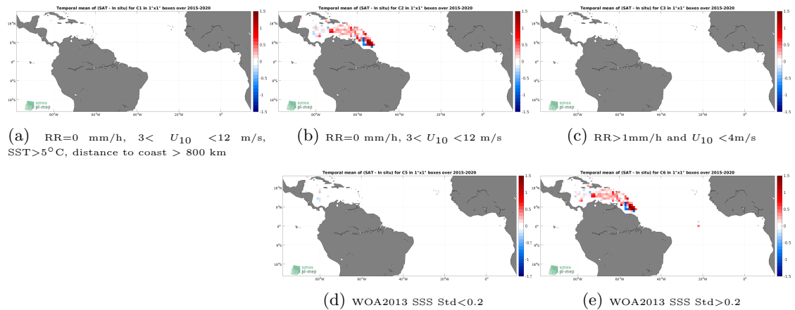
Figure 11: Temporal mean gridded over spatial boxes of size 1^\circ \times 1^\circ of \Delta SSS (SMAP SSS L3 v5 - Monthly (RSS) - Surface drifters) for 5 different subdatasets corresponding to:RR=0 mm/h, 3 < U_{10} < 12 m/s, SST >5^\circ\text{C} , distance to coast > 800 km (a), RR=0 mm/h, 3 < U_{10} < 12 m/s (b), RR >1 mm/h and U_{10} < 4 m/s (c), WOA2013 SSS Std <0.2 (d), WOA2013 SSS Std >0.2 (e).
