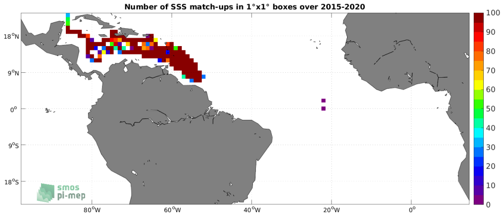
Figure 3: Number of SSS match-ups between Surface drifters SSS and the SMAP SSS L3 v5 - Monthly (RSS) SSS product for the Tropical Atlantic Ocean Pi-MEP region over 1^\circ \times 1^\circ boxes and for the full satellite product period.
