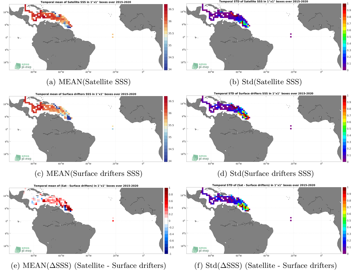
Figure 5: Temporal mean (left) and Std (right) of SSS from SMAP SSS L3 v5 - Monthly (RSS) (top), Surface drifters (middle), and of \Delta SSS (Satellite - Surface drifters). Only match-up pairs are used to generate these maps.
