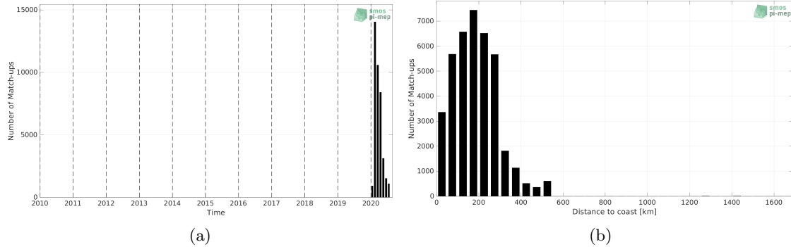
Figure 1: Number of match-ups between Surface drifters and SMAP SSS L3 v5 - Monthly (RSS) SSS as a function of time (a) and as function of the distance to coast (b) over the Tropical Atlantic Ocean Pi-MEP region and for the full satellite product period.
