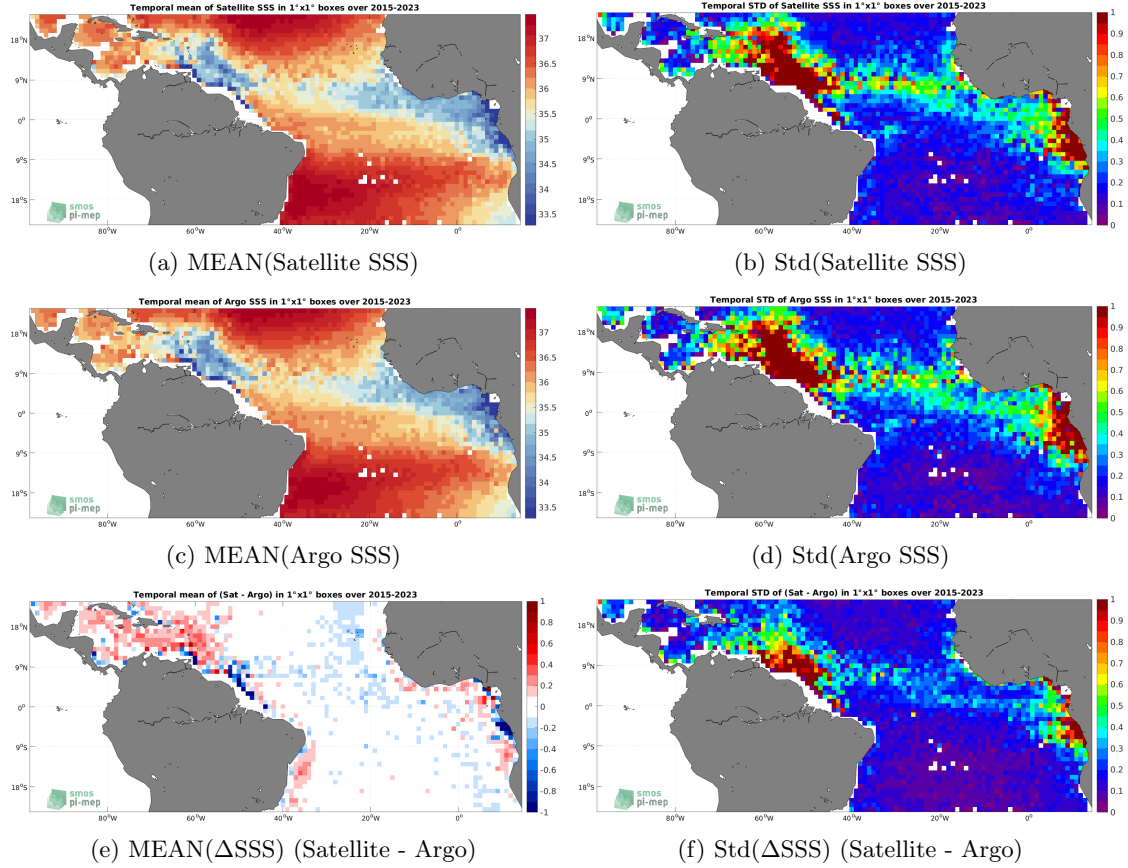
Figure 6: Temporal mean (left) and Std (right) of SSS from SMAP SSS L3 v5 - Monthly (RSS) (top), Argo (middle), and of \Delta\text{SSS} (Satellite - Argo). Only match-up pairs are used to generate these maps.
