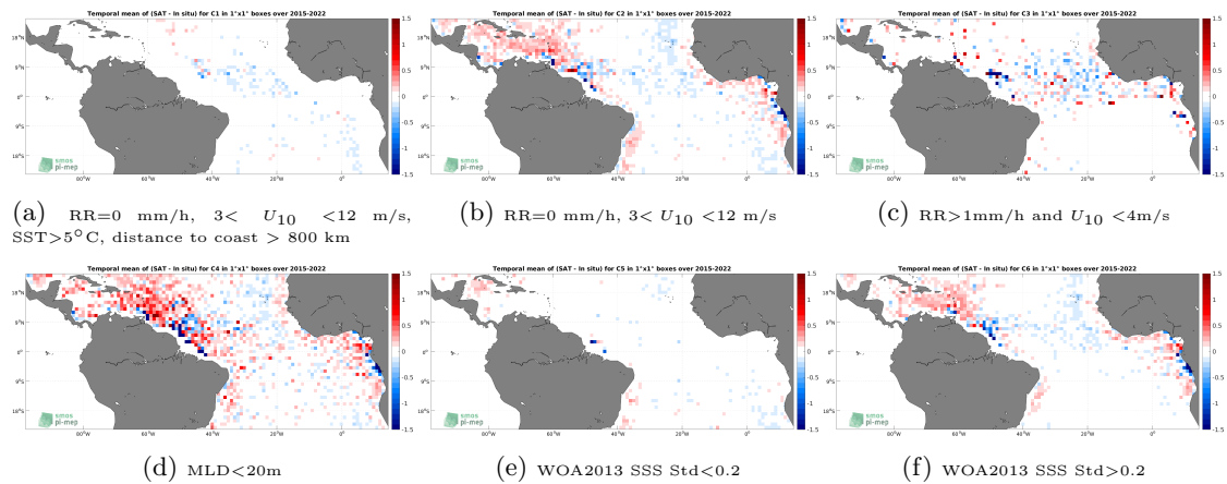
Figure 12: Temporal mean gridded over spatial boxes of size 1^\circ \times 1^\circ of \Delta SSS (SMAP SSS L3 v5 - Monthly (RSS) - Argo) for 6 different subdatasets corresponding to:RR=0 mm/h, 3 < U_{10} < 12 m/s, SST >5^\circ\text{C} , distance to coast > 800 km (a), RR=0 mm/h, 3 < U_{10} < 12 m/s (b), RR >1 mm/h and U_{10} < 4 m/s (c),MLD <20 m (d),WOA2013 SSS Std <0.2 (e),WOA2013 SSS Std >0.2 (f).
