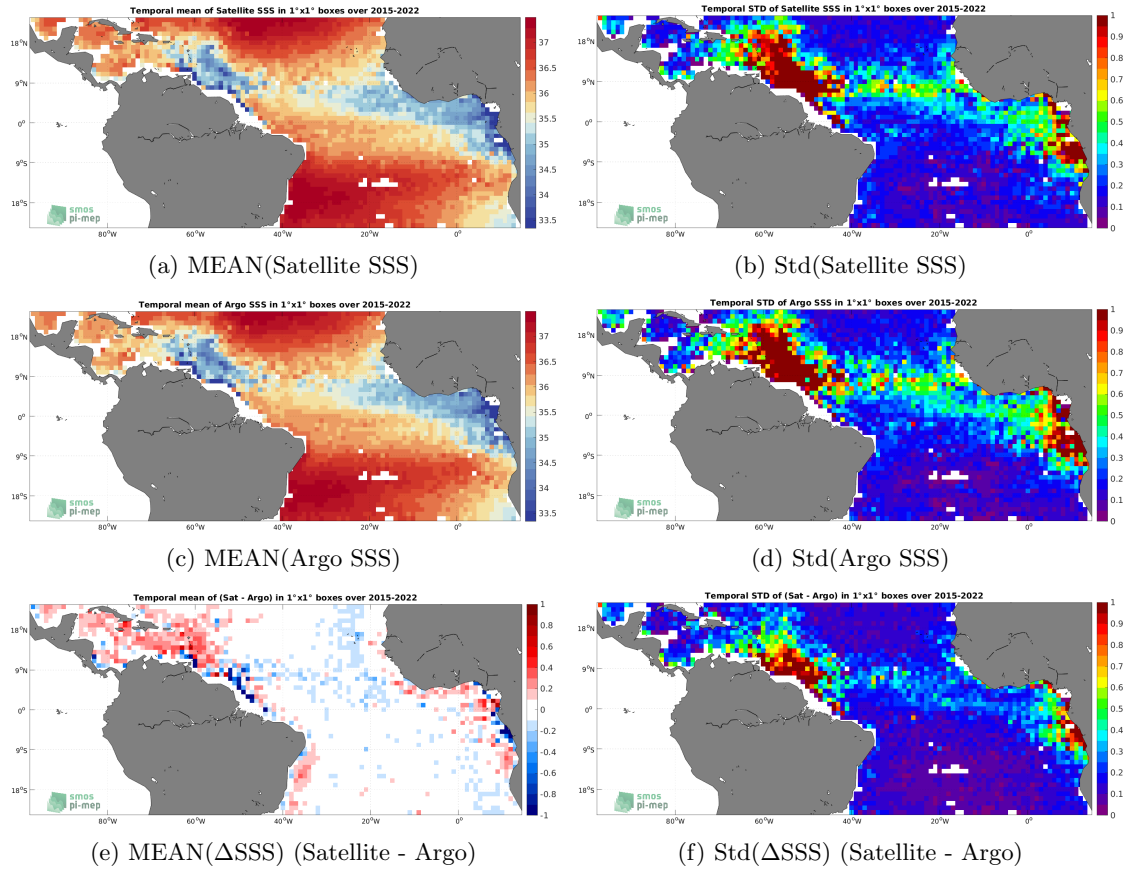
Figure 6: Temporal mean (left) and Std (right) of SSS from SMAP SSS L3 v5 - Monthly (RSS) (top), Argo (middle), and of \Delta SSS (Satellite - Argo). Only match-up pairs are used to generate these maps.
