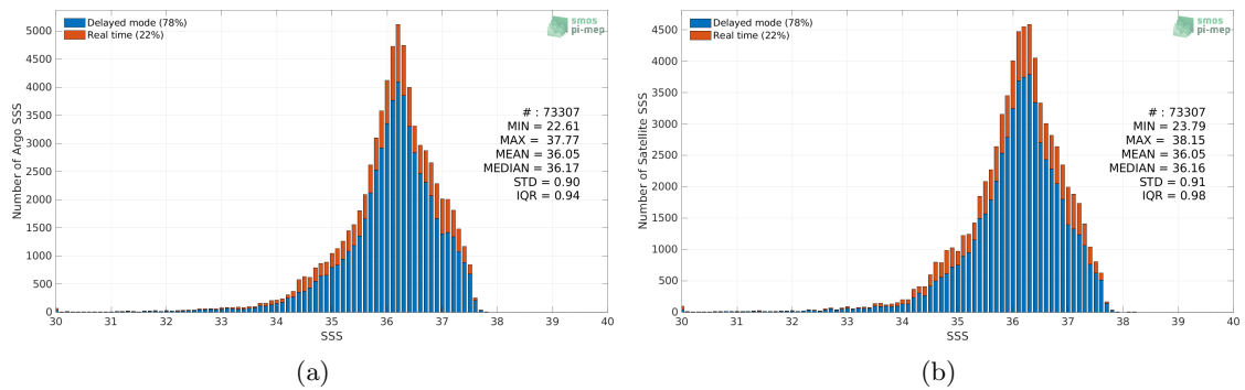
Figure 2: Histograms of SSS from Argo (a) and SMAP SSS L3 v5 - Monthly (RSS) (b) considering all match-up pairs per bins of 0.1 over the Tropical Atlantic Ocean Pi-MEP region and for the full satellite product period.
