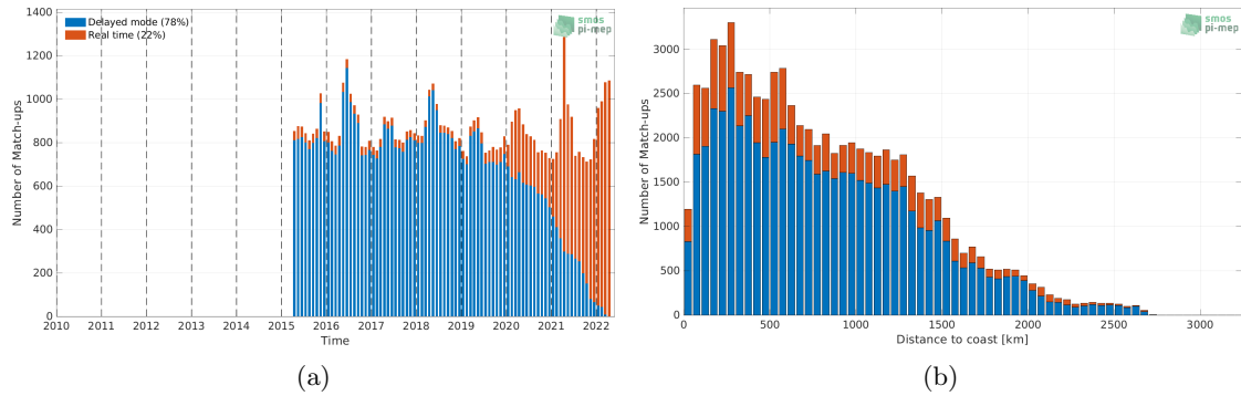
Figure 1: Number of match-ups between Argo and SMAP SSS L3 v5 - Monthly (RSS) SSS as a function of time (a) and as function of the distance to coast (b) over the Tropical Atlantic Ocean Pi-MEP region and for the full satellite product period.
