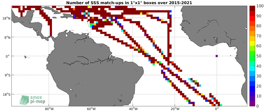
Figure 4: Number of SSS match-ups between TSG (SAMOS) SSS and the SMAP SSS L3 v4 - 8-Day running (RSS) SSS product for the Tropical Atlantic Ocean Pi-MEP region over 1^\circ \times 1^\circ boxes and for the full satellite product period.
