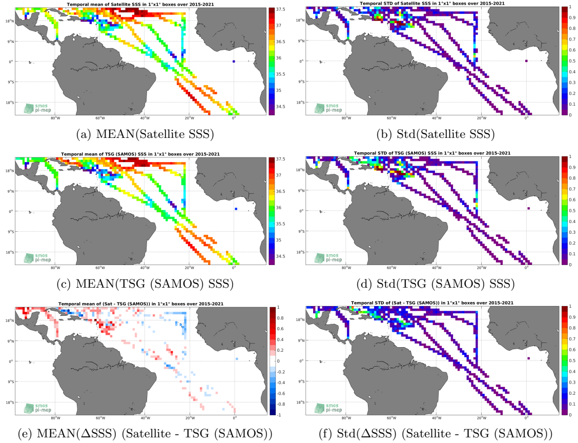
Figure 6: Temporal mean (left) and Std (right) of SSS from SMAP SSS L3 v4 - 8-Day running (RSS) (top), TSG (SAMOS) (middle), and of \Delta SSS (Satellite - TSG (SAMOS)). Only match-up pairs are used to generate these maps.
