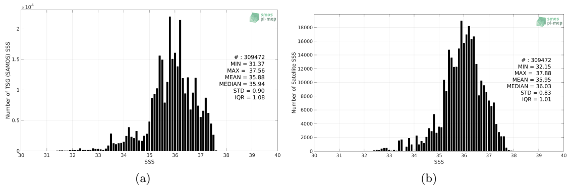
Figure 2: Histograms of SSS from TSG (SAMOS) (a) and SMAP SSS L3 v4 - 8-Day running (RSS) (b) considering all match-up pairs per bins of 0.1 over the Tropical Atlantic Ocean Pi-MEP region and for the full satellite product period.
