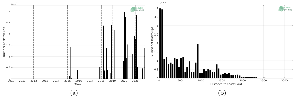
Figure 1: Number of match-ups between TSG (SAMOS) and SMAP SSS L3 v4 - 8-Day running (RSS) SSS as a function of time (a) and as function of the distance to coast (b) over the Tropical Atlantic Ocean Pi-MEP region and for the full satellite product period.
