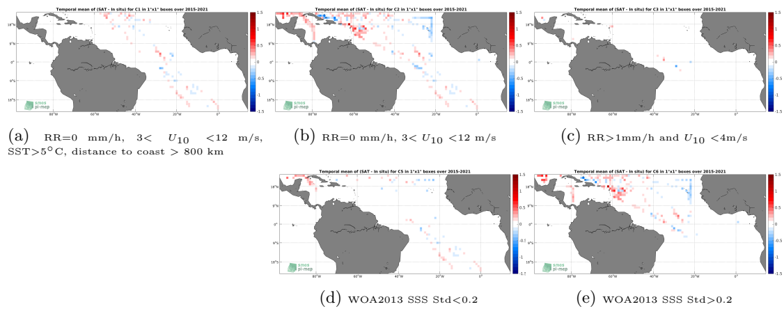
Figure 12: Temporal mean gridded over spatial boxes of size 1^\circ \times 1^\circ of \Delta\text{SSS} (SMAP SSS L3 v4 - 8-Day running (RSS) - TSG (SAMOS)) for 5 different subdatasets corresponding to:RR=0 mm/h, 3 < U_{10} < 12 m/s, SST >5^\circ\text{C} , distance to coast > 800 km (a), RR=0 mm/h, 3 < U_{10} < 12 m/s (b), RR >1 mm/h and U_{10} < 4 m/s (c), WOA2013 SSS Std <0.2 (d), WOA2013 SSS Std >0.2 (e).
