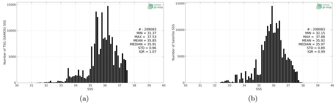
Figure 2: Histograms of SSS from TSG (SAMOS) (a) and SMAP SSS L3 v4 - 8-Day running (RSS) (b) considering all match-up pairs per bins of 0.1 over the Tropical Atlantic Ocean Pi-MEP region and for the full satellite product period.
